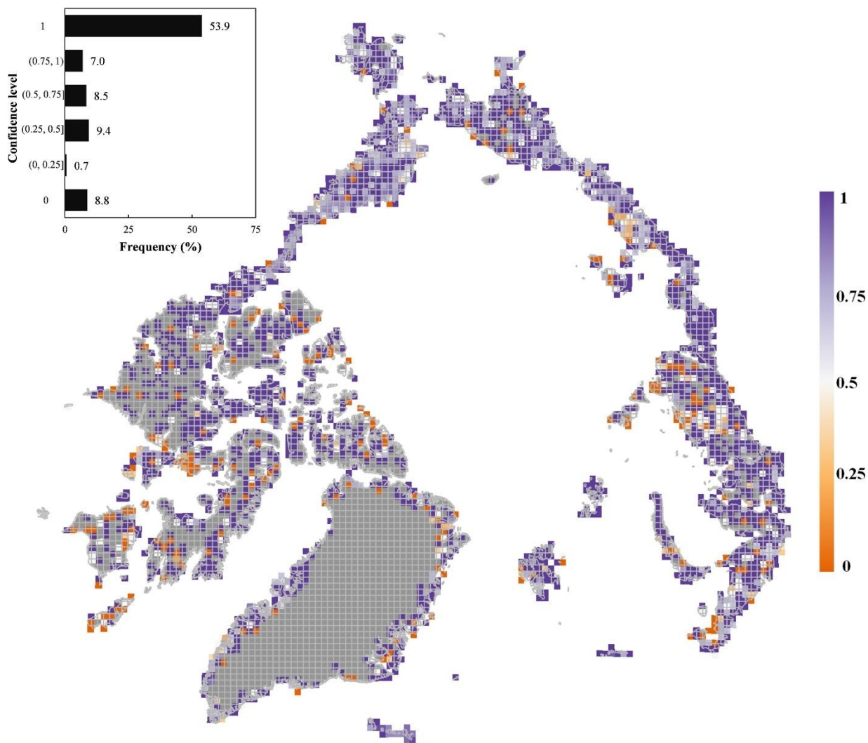
Figure 4: Map of CALC-2020 classification confidence calculated at a 50 \text{ km} \times 50 \text{ km} tile scale. The grey grid denotes no validation sample point distribution. The bar plot shows the statistical distribution of six broad classification confidence intervals.
