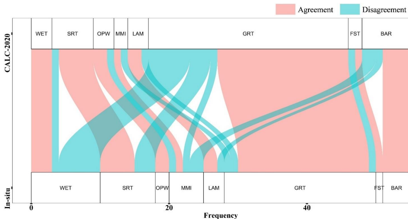
Figure 5: CALC-2020 map performance in 55 field and flux tower sites. The block width represents the frequency (site number) identified by our estimation and in-situ reports, respectively. Land cover abbreviations are given in Table 1.
