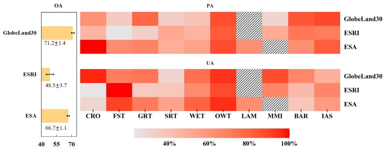
325 Figure 7: Accuracy statistics of three global land cover products for the circumpolar Arctic based on validation sample. Grass (ESA WorldCover, ESRI Global Land Cover) and wet tundra classes (GlobeLand30) are treated as equivalents of graminoid tundra and wetland, respectively. Stripped blocks represent the absence or less than 0.25% area proportion of specific class(es).
