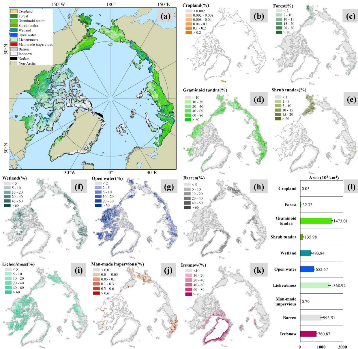
365 Figure 9: Circumpolar Arctic land cover estimated by the CALC-2020 map. (a) Land cover distribution at the 10 m pixel scale. (b)-(k) display the biome-specific area proportion in each 1°x1° land tile. (l) shows area statistics of all land cover types across the terrestrial Arctic (unit of 10³ km²). Error bars represent 95% confidence intervals.
