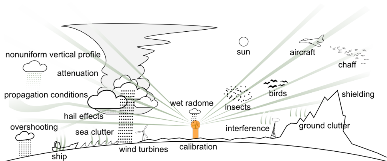
20 Figure 1. Example of error sources effecting weather radar measurements. Figure by Markus Peura, Finnish Meteorological Institute (FMI), used with permission.
