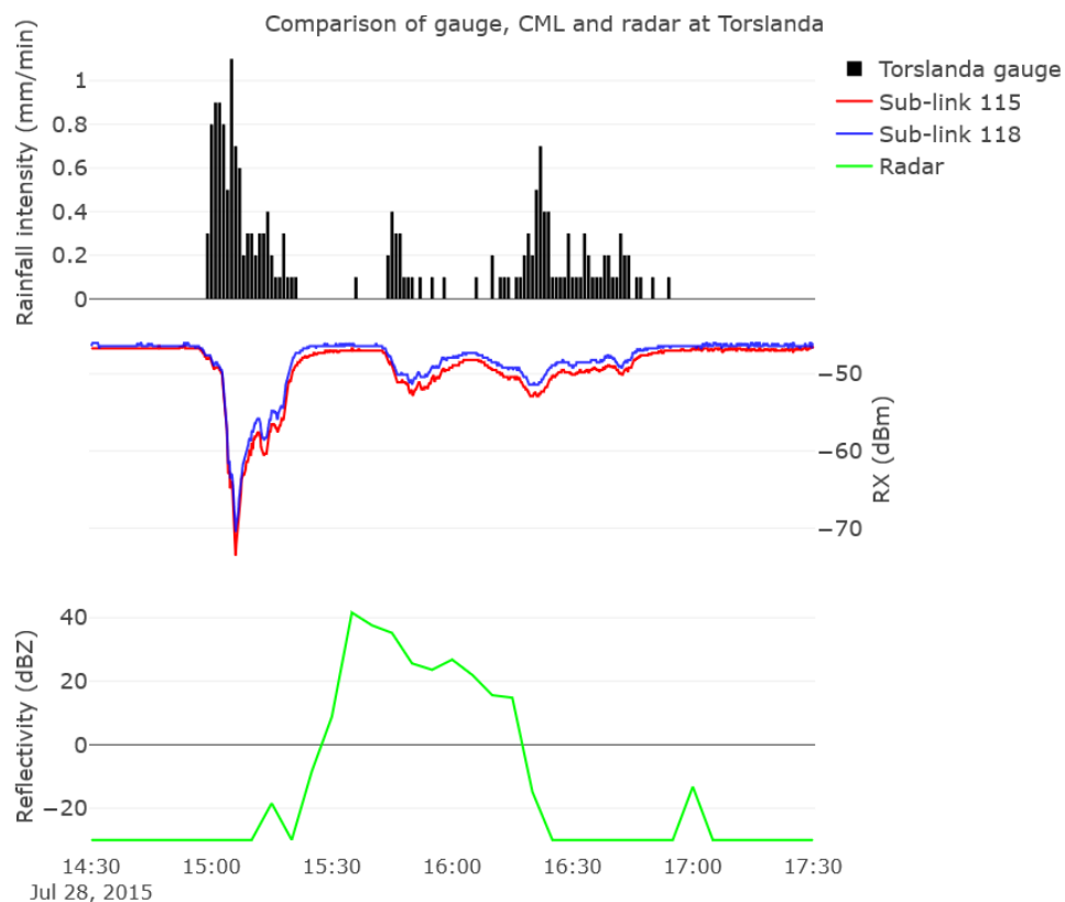
5 Figure 11. An intense rainfall event at the Torslanda gauge on the 28 July 2015 (top), and the corresponding RX signal fade for a nearby microwave link (middle, link 10227, sub-links 115 and 118) as well as the reflectivity of the overlying radar pixel (bottom). The location of the gauge and link are shown in Figure 12. Sub-link 115 is vertically polarized, with frequency 28.23 GHz, covering a 1.8km distance. Sub-link 118 is identical except for operating at 29.24 GHz. An interactive version of this figure is available together with the data set (see section 6).
