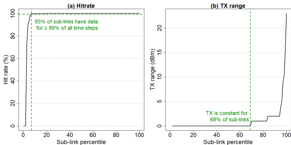
Figure 6. CML data collection performance. (a) Distribution of the data collection hit rate (% of time steps with valid RX and TX measurements) across all sub-links. 93% of sub-links have both RX and TX data for \geq 99\% of all time steps in the sampling period. (b) Stability of the transmitted signal strength (TX) across all sub-links. TX does not vary at all for a majority of the sub-links (68%).
