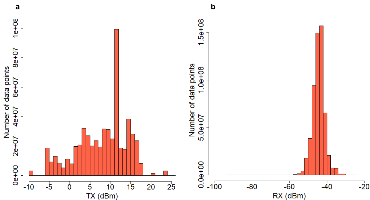
Figure 7. Histograms of (a) transmitted signal strength (TX), and (b) received signal strength (RX).
