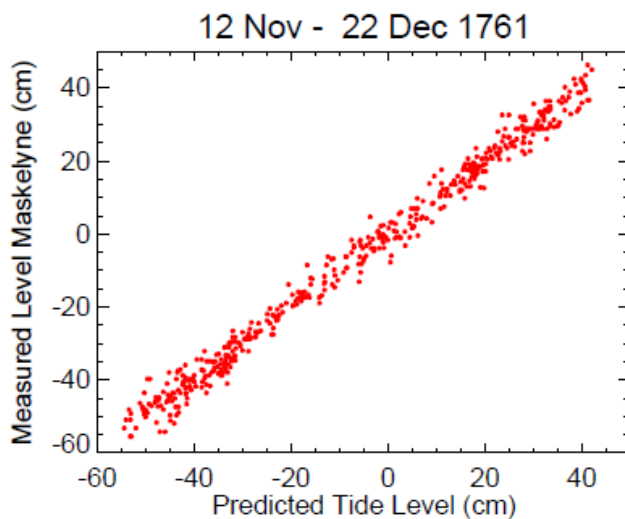
Figure 4 (a). Predicted and Maskelyne sea levels values after datum shift adjustment.
