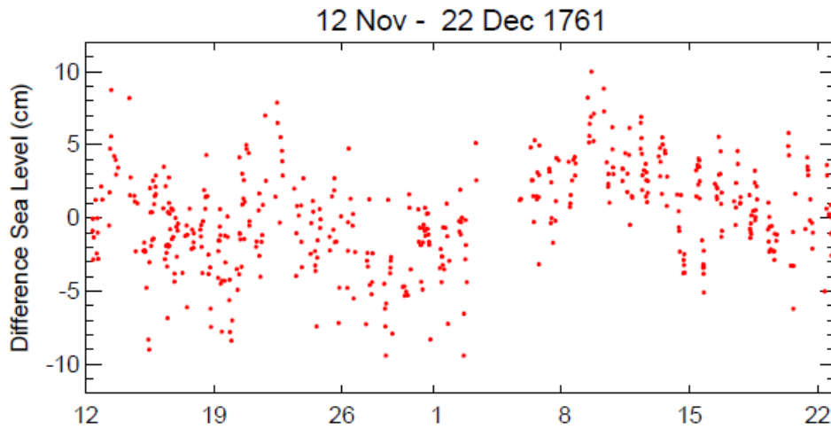
Figure 3(c). Sea level differences (Maskelyne - Predicted) with the overall mean difference removed.
