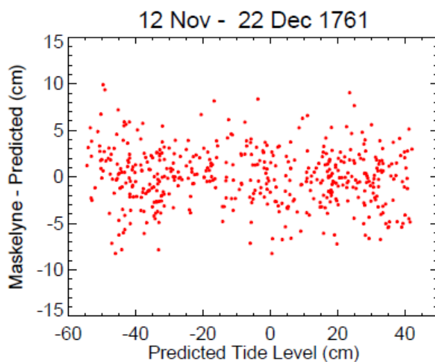
Figure 4 (b). Sea level differences (Maskelyne-Predicted) after datum shift correction showing no major dependence on tidal level.
