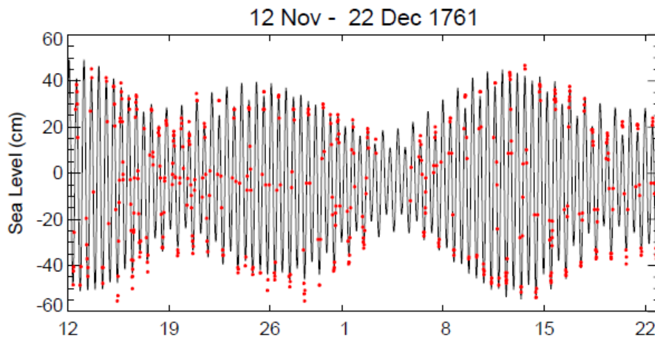
Figure 3(a). 1-minute predicted heights for 12 November - 22 December 1761 together with the Maskelyne sea levels shown by red dots. The two sets of values have been adjusted to have zero mean.
