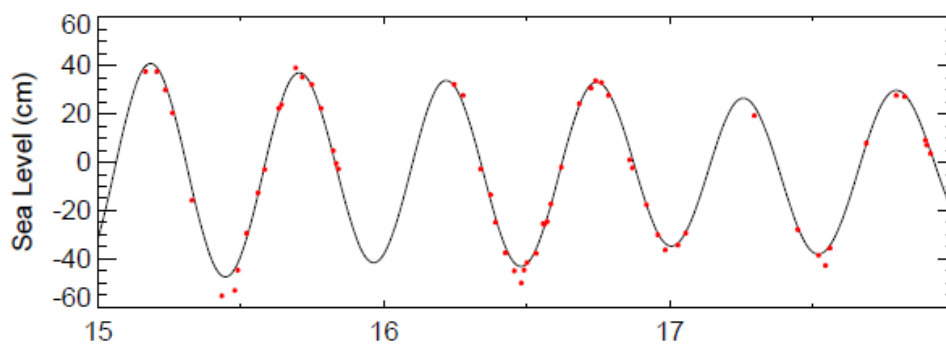
Figure 3(a). 1-minute predicted heights for 12 November - 22 December 1761 together with the Maskelyne sea levels shown by red dots. The two sets of values have been adjusted to have zero mean.
