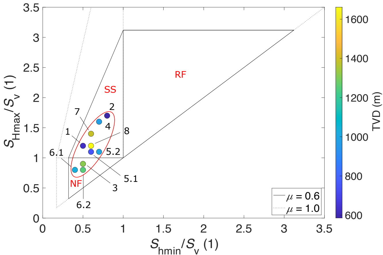
Figure 6. Normalized-Normalised stress polygon for two different coefficients of friction, \mu , of 0.6 and 1.0 with averaged stress magnitude values recorded across the greater Ruhr region (see Table 3 for the actual values) for each test location and depth level (NF - normal faulting, SS - strike-slip faulting, RF - reverse/thrust faulting, TVD - true vertical depth). Numbers correlate to references from Table 3. The stress regime of the study area, based on the collected data within this study, is shaded in light grey outlined with a red ellipse .
