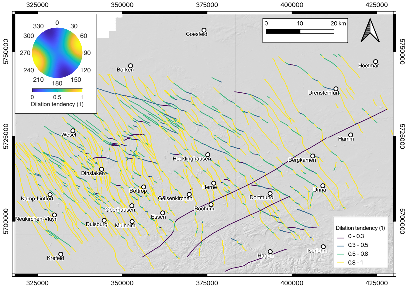
Figure 10. Dilation Dilation tendency of geological discontinuities within the Ruhr region (GD NRW, 2017) (GD NRW, 2017, 2019) at depth of 1200 m computed based on the stress tensor constrained from this study with P_p of 13.2 11.8 MPa, S_{hmin} of 17.4 MPa, S_{Hmax} of 33.7 MPa, S_v of 29.3 MPa, and average S_{Hmax} orientation of 161^\circ ; Stereographic projection of dilation tendency based on the constructed stress tensor is presented in the top left corner.
