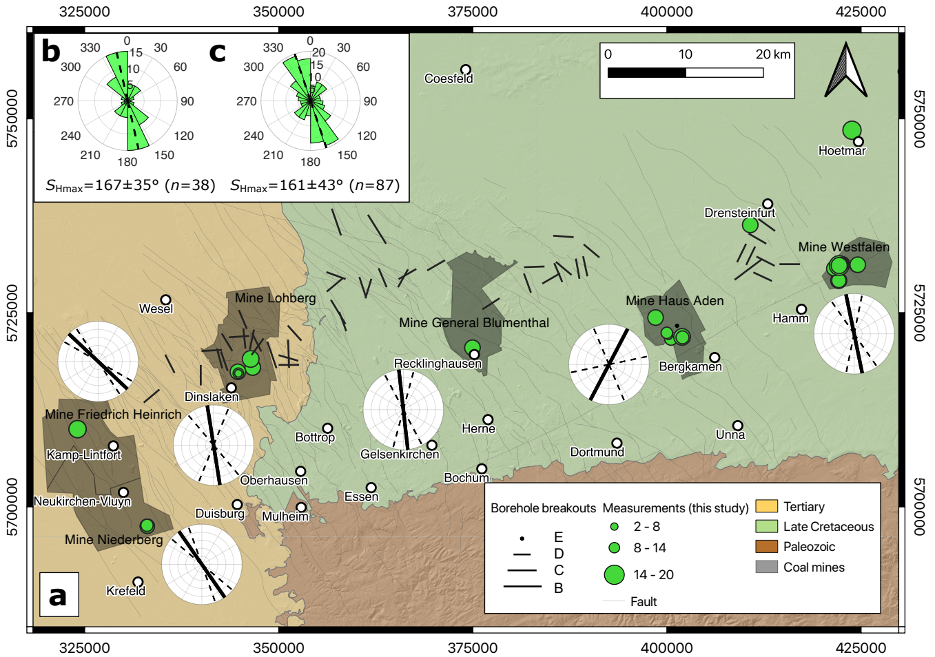
Figure 7. a) A map of the greater Ruhr region with major geological discontinuities (modified after GD-NRW (2017) / GD NRW (2017, 2019) ) and locations of stress magnitude data records described in this study; black shaded areas represent coal mining areas active in 1980s; polar plots represent average S_{Hmax} orientations (solid line) and its standard deviation (dashed line) registered in each coal mine (black thick lines show the orientation of the maximum horizontal stress, S_{Hmax} , available in the World Stress Map database 2016 (Heidbach et al., 2018), where line length is proportional to data quality); b) rose plot of S_{Hmax} orientations based on hydrofracturing tests collected in this study ( n = 38 ) with D- and E-qualities where average S_{Hmax} orientation (dashed line) amounted to 167 \pm 35^\circ ; c) rose plot of S_{Hmax} orientation data records based on this study and data points from the greater Ruhr region available in the World Stress Map database release from 2016 (Heidbach et al., 2018), with B- to E-qualities, with an average S_{Hmax} orientation (dashed line) of 161 \pm 43^\circ ( n = 87 ).
