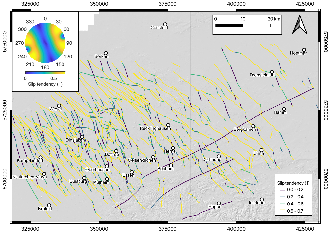
Figure 9. Slip tendency of geological discontinuities within the Ruhr region (GD NRW, 2017) (GD NRW, 2017, 2019) at depth of 1200 m computed based on the stress tensor constrained from this study with P_p of 13.2 – 11.8 MPa, S_{hmin} of 17.4 MPa, S_{Hmax} of 33.7 MPa, S_v of 29.3 MPa, and average S_{Hmax} orientation of 161^\circ . Stereographic projection of slip tendency based on the constructed stress tensor is presented in the top left corner.
