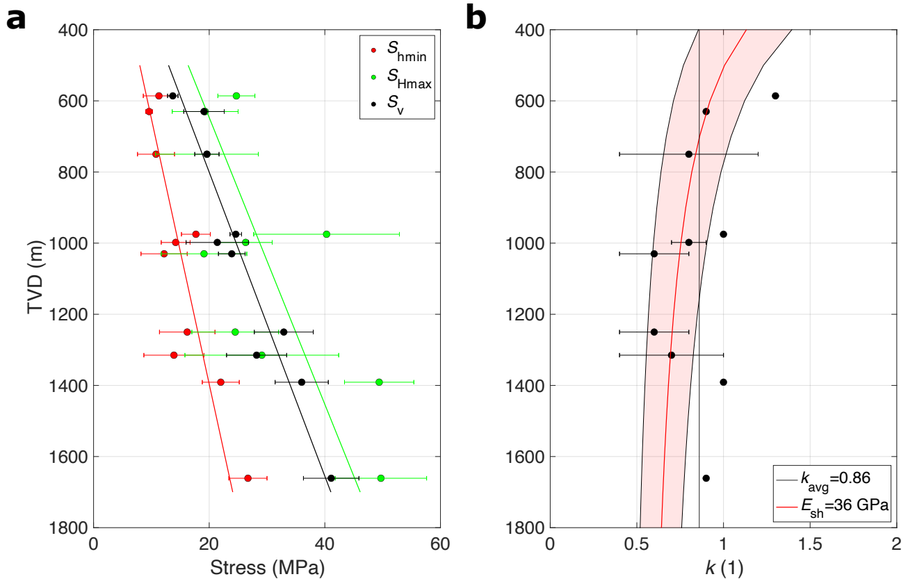
Figure 5. a) In situ stress test magnitudes recorded across the greater Ruhr region based on averaged values from each test location (differentiation was made for values from different depth levels in the same coal mine) with trend lines computed based on Equation 7, 8, and 9 (see Table 3 for the actual values; TVD - true vertical depth); b) mean stress ratio, k , (i.e., ratio of average horizontal stress and the vertical stress) based on the averaged stress tests magnitudes recorded across the greater Ruhr region (see Table 3 for actual values). The average k of 0.86 based on hydrofracturing test results acquired from this study, is marked with a solid black line; for comparison k computed based on the approach by Sheorey (1994) for Young's modulus, E_{sh} , of 36 \pm 11 GPa based on laboratory measurements on core samples from the Westfalen coal mine (MeSy, 1994) is presented with solid red line and area shaded in red represent represents its standard deviation.
