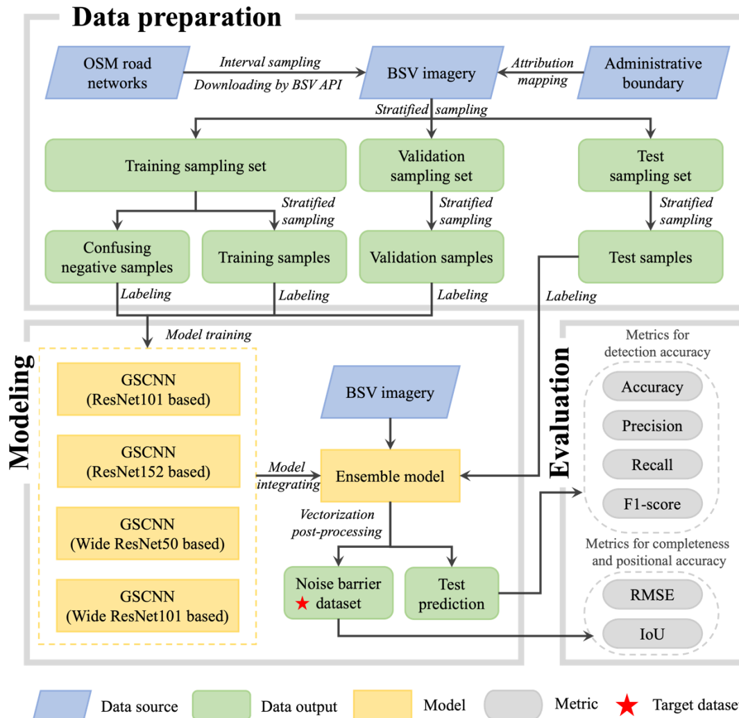
120 Figure 1: The flow chart of GeoAI framework to generate the vectorized RNB dataset.
