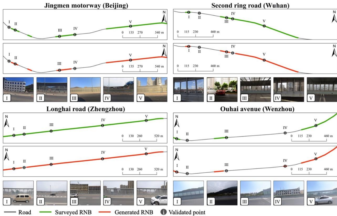
Figure 10: RNB mapping result in city scale. (BSV images are from Baidu Maps)
