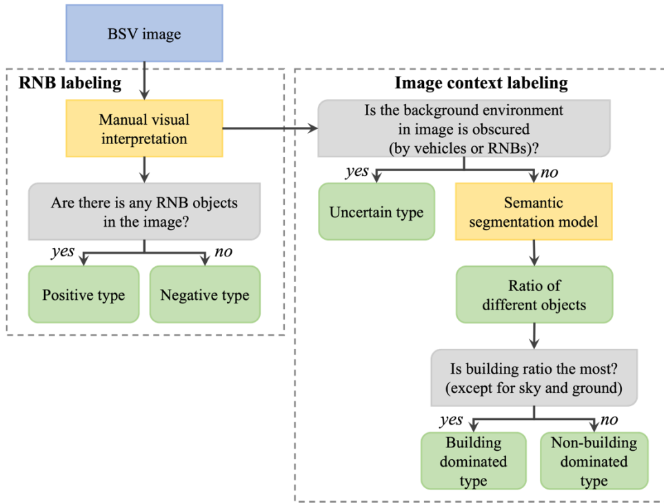
Figure 6: The flow chart of BSV image labeling.
