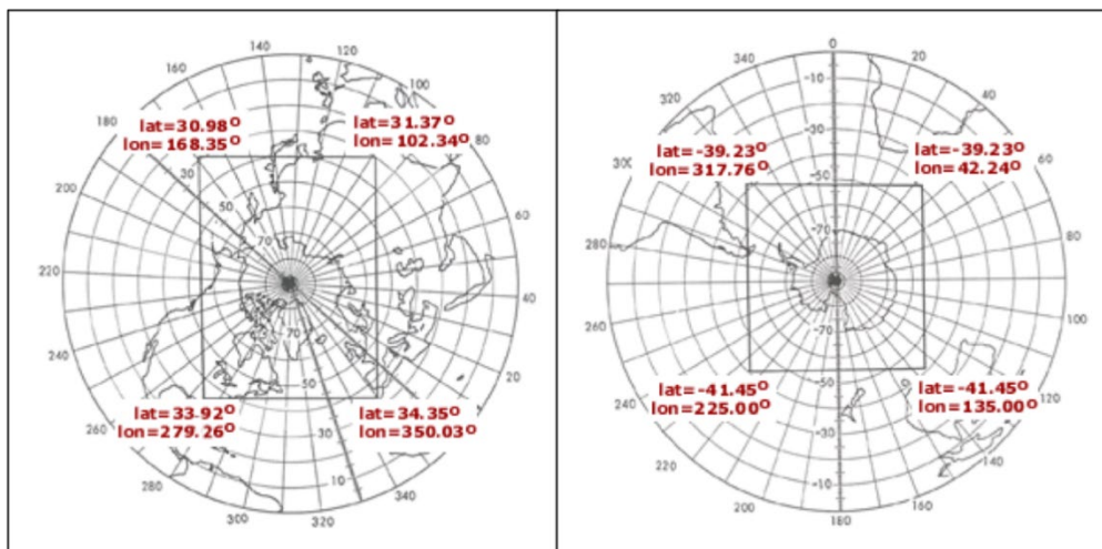
Figure S1. NSIDC Polar Stereographic Projection coverage maps in the Arctic (left) and Antarctic (right) (from NSIDC, https://nsidc.org/data/polar-stereo ).
