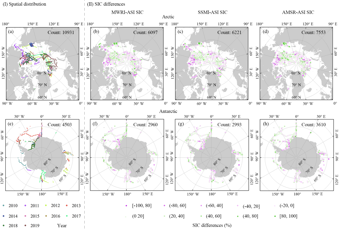
380 Figure 8: (I). Spatial distributions of the ship-based observational SIC in 2010–2019. (II). SIC differences between the PM SIC products and ship-based observations.
