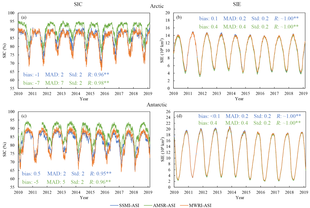
210 Figure 1: Daily average SIC and daily SIE from November 2010 to December 2019. Also shown are the differences in SIC and SIE between the MWRI-ASI and SSMI-ASI (blue number) and between the MWRI-ASI and AMSR-ASI (green number). The statistical significance at 95% and 99% confidence levels are marked by * and **, respectively, and those below 95% confidence level are not marked, the same below.
