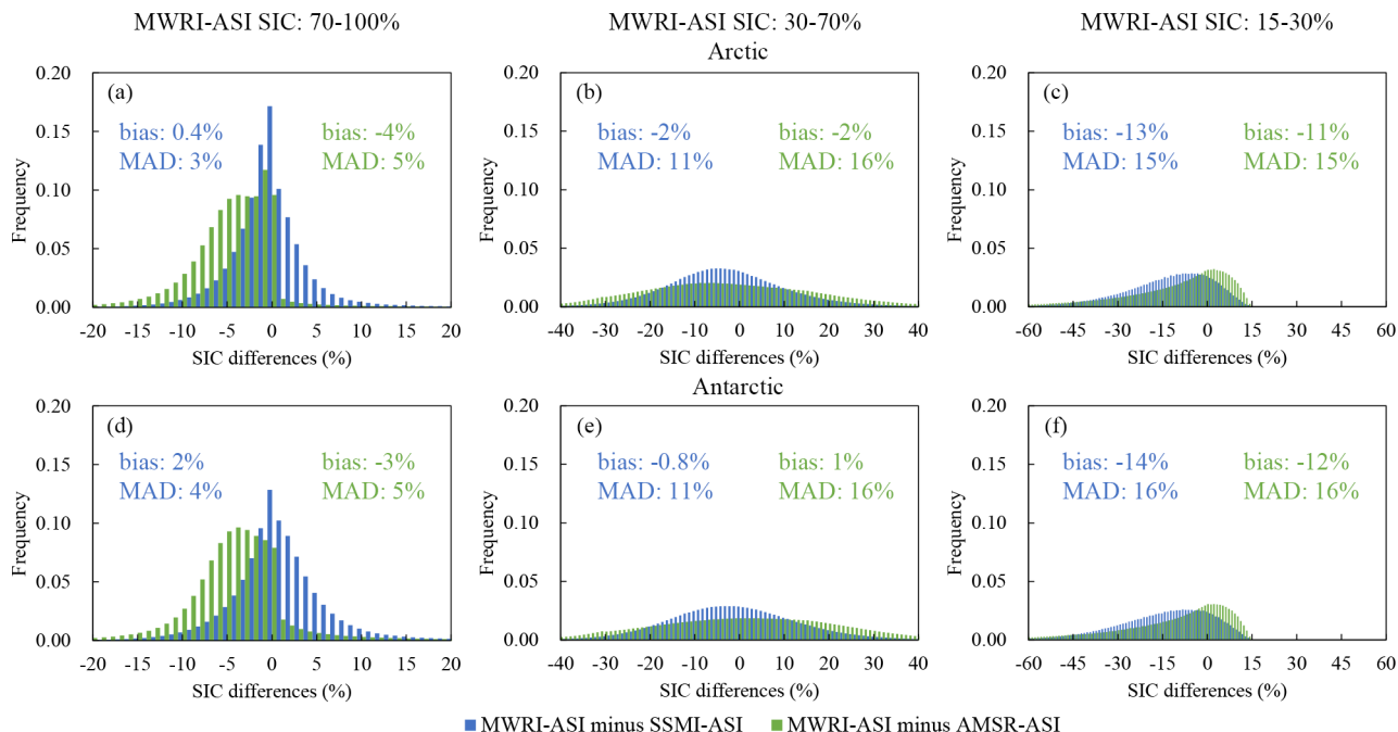
265 Figure 4: Histogram of SIC differences between the MWRI-ASI and SSMI-ASI and between the MWRI-ASI and AMSR-ASI with the MWRI-ASI SIC of 70–100%, 30–70%, and 15–30% from November 2010 to December 2019. Also shown are the differences in SIC between the MWRI-ASI and SSMI-ASI (blue number) and between the MWRI-ASI and AMSR-ASI (green number).
