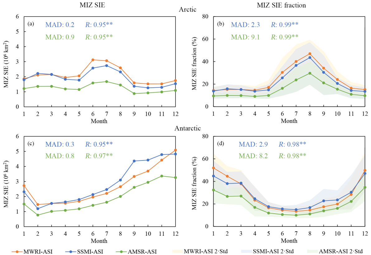
225 Figure 2: Monthly MIZ SIE and MIZ SIE fraction from November 2010 to December 2019. Also shown are the differences in MIZ SIE and MIZ SIE fraction between the MWRI-ASI and SSMI-ASI (blue number) and between the MWRI-ASI and AMSR-ASI (green number). The shades present the 2 Stds from the monthly MIZ SIE fraction.
