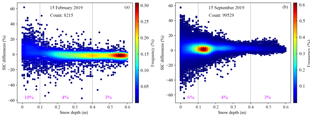
270 Figure 5: Frequency of SIC differences between the MWRI-ASI and SSMI-ASI with different snow depths in the Antarctic on 15 February (a) and 15 September (b) 2019. The purple numbers present the MADs in SIC between the MWRI-ASI and SSMI-ASI with the snow depth of 0-0.1 m, 0.1-0.4 m, and 0.4-0.6 m.
