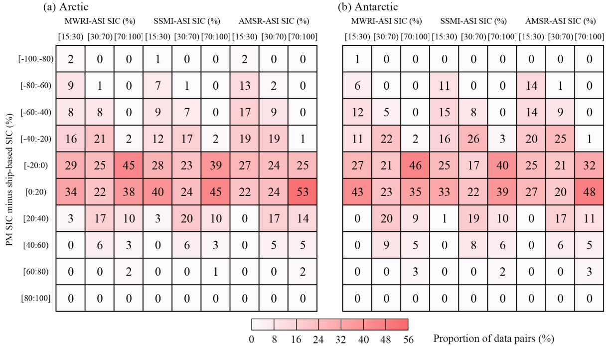
Figure 7: Proportion of data pairs (number in the grid) of the PM SIC products vs SIC differences between the PM SIC products and ship-based SIC. The PM SIC is divided to three categories of 15–30%, 30–70%, and 70–100% (horizontal axis). The SIC differences are grouped with an interval of 20% (vertical axis).
