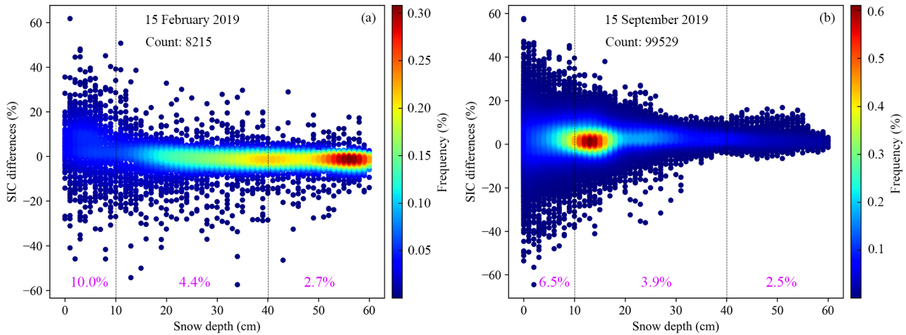
275 Figure 5: Frequency of SIC differences between the MWRI-ASI and SSMI-ASI with different snow depths in the Antarctic on 15 February (a) and 15 September (b) 2019. The purple numbers present the MADs in SIC between the MWRI-ASI and SSMI-ASI with the snow depth of 0-10 cm, 10-40 cm, and 40-60 cm.
