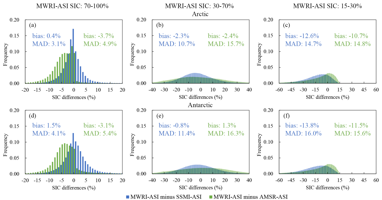
270 Figure 4: Histogram of SIC differences between the MWRI-ASI and SSMI-ASI and between the MWRI-ASI and AMSR-ASI with the MWRI-ASI SIC of 70–100%, 30–70%, and 15–30% from November 2010 to December 2019. Also shown are the differences in SIC between the MWRI-ASI and SSMI-ASI (blue number) and between the MWRI-ASI and AMSR-ASI (green number).
