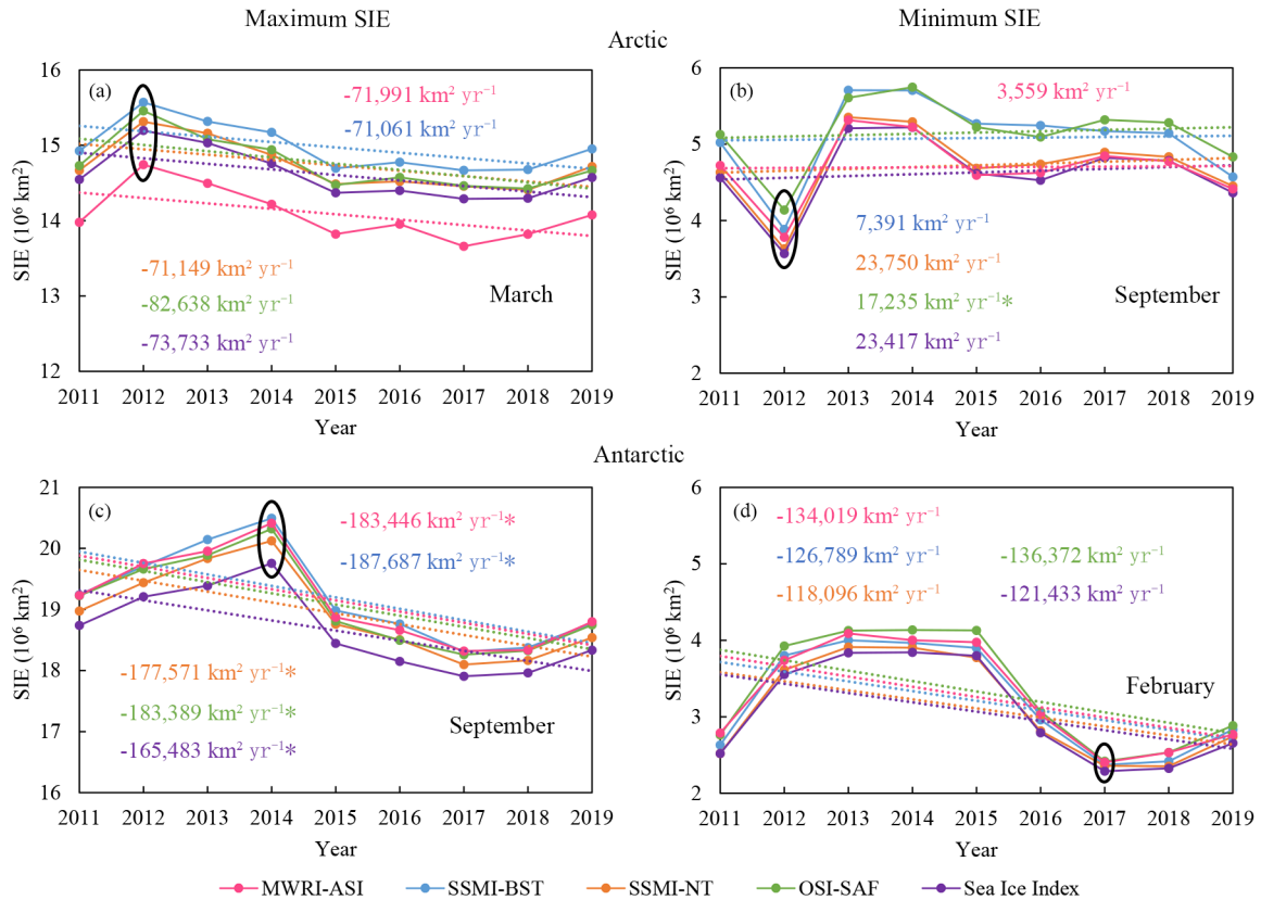
335 Figure 6: Annual maximum and minimum SIEs from 2011 to 2019. Also shown are the corresponding SIE trends of the MWRI-ASI (pink number), SSMI-BST (blue number), SSMI-NT (orange number), OSI-SAF (green number), and Sea Ice Index (purple number). The black circles present the largest annual maximum SIE and the smallest annual minimum SIE. Note that the smallest Antarctic annual minimum SIE of the SSMI-NT is observed in February 2018.
