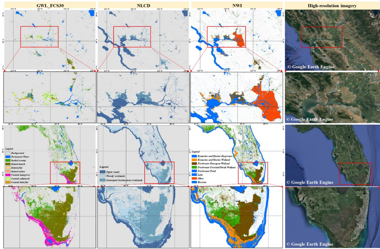
815 Figure 16. The comparisons between GWL_FCS30 in 2020, National Land Cover Database (NLCD) wetland Layer (Homer et al., 2020) and National Wetlands Inventory (NWI, https://www.fws.gov/program/national-wetlands-inventory , last access: Nov 12, 2022) in San Francisco and Florida. The high-resolution imagery came from the Google Earth Engine platform ( https://earthengine.google.com ; last access: 12 Nov 2022).
