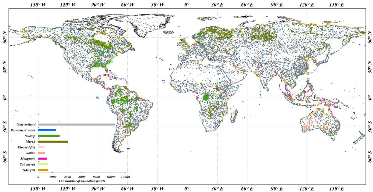
Figure 26. The spatial distribution of 18,701 25,709 global wetland validation samples using stratified sampling strategy.
