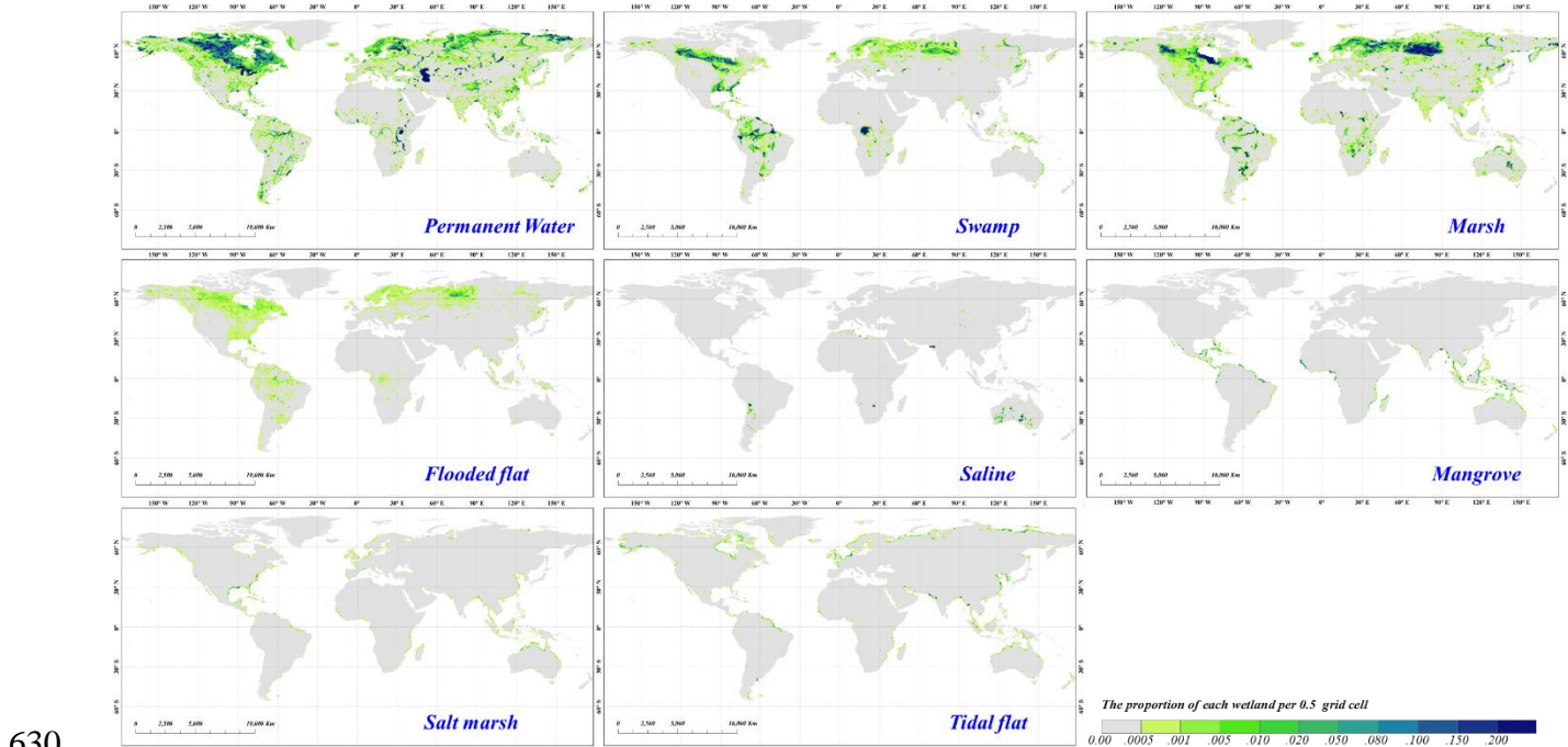
Figure 7.10. The spatial distributions of the seven eight wetland sub-categories after aggregating them to a resolution of 0.5^{\circ} \times 0.5^{\circ} .
