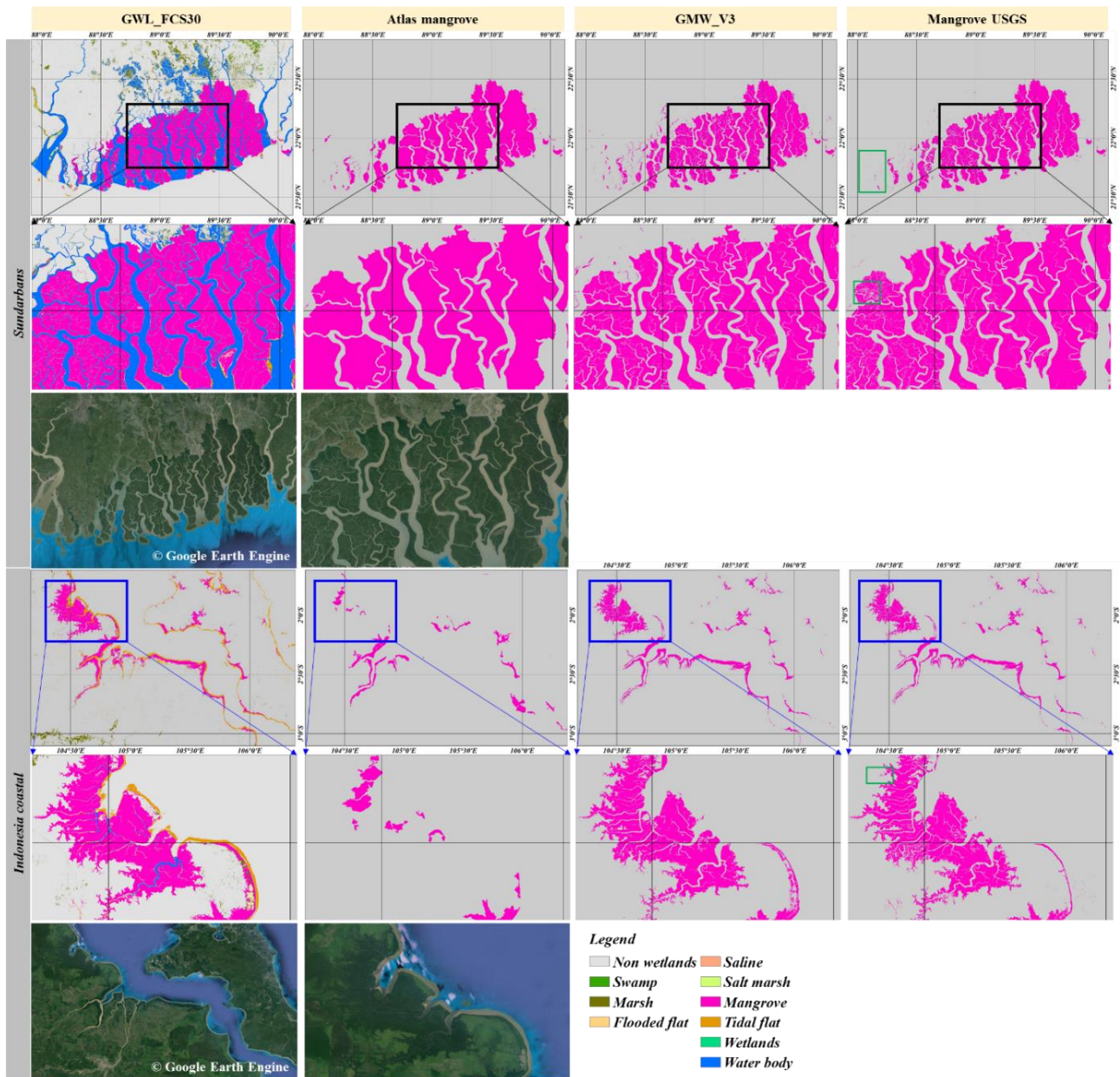
755 Figure 11.14. The cross-comparisons between our GWL_FCS30 wetland maps with three mangrove products (Atlas mangrove developed by Spalding (2010), GMW_V3 ( Global mangrove watch ) developed by Bunting et al. (2022) and Mangrove USGS developed by Giri et al. (2011)) in Sundarbans and coastal Indonesia. The high-resolution imagery came from the Google Earth Engine platform ( https://earthengine.google.com ; last access: 16 May 2022).
