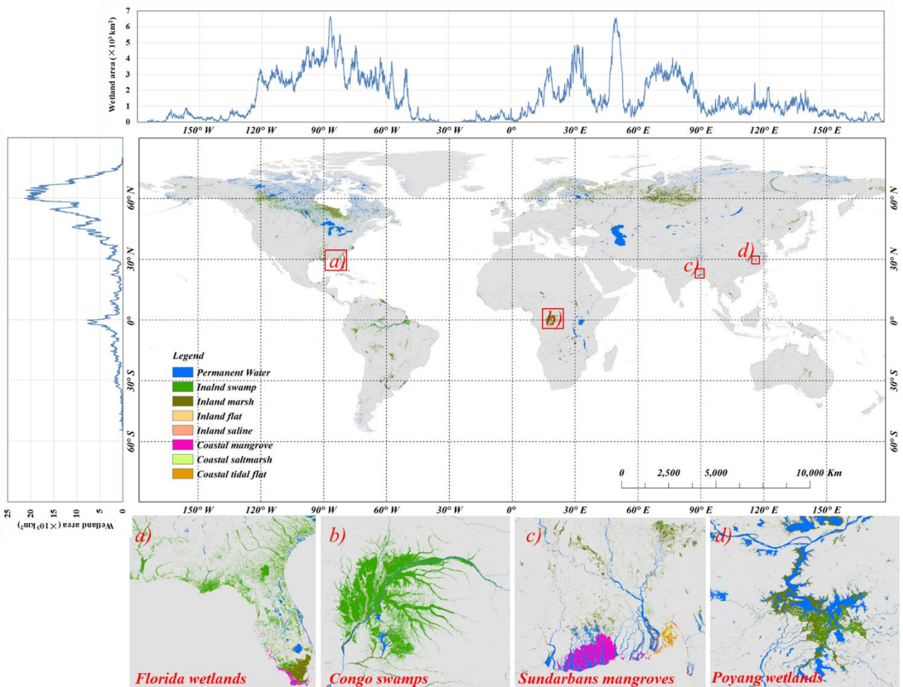
Figure 69. The overview of global 30-m fine wetland maps and their area statistics in latitudinal and longitudinal directions in 2020. Four local enlargements in (a) Florida, (b) Congo Basin, (c) Sundarbans, and (d) Poyang Lake were also illustrated.
