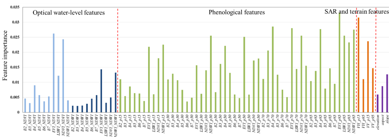
Figure 158. The importance of multi-sourced and multi-temporal features derived from the random forest classification model.
