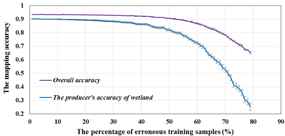
5. Figure 147. The relationship between mapping accuracies with the percentage of erroneous training samples with a step of 1%.
