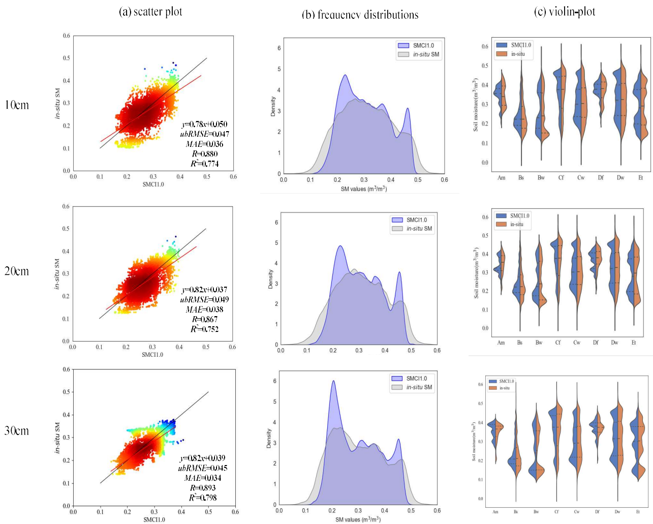
700 Figure 3: Same as Fig. 2 but for station-to-station estimating.
