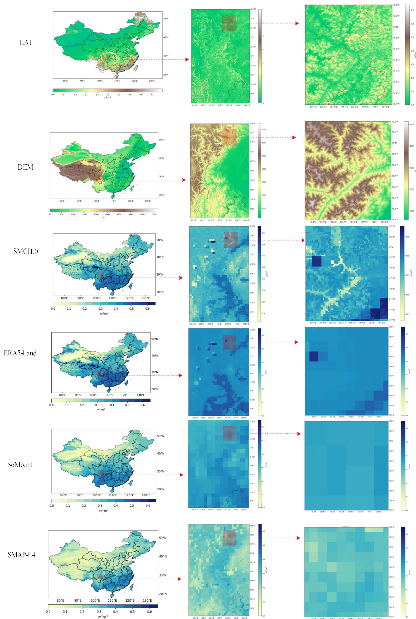
715 Figure 7: Soil moisture maps from different products on 1 st January 2016. The resolution is 1km for SMC1.0, 9km for ERA5-Land and SMAP-L4 and 0.25 degree for SoMo.ml.
