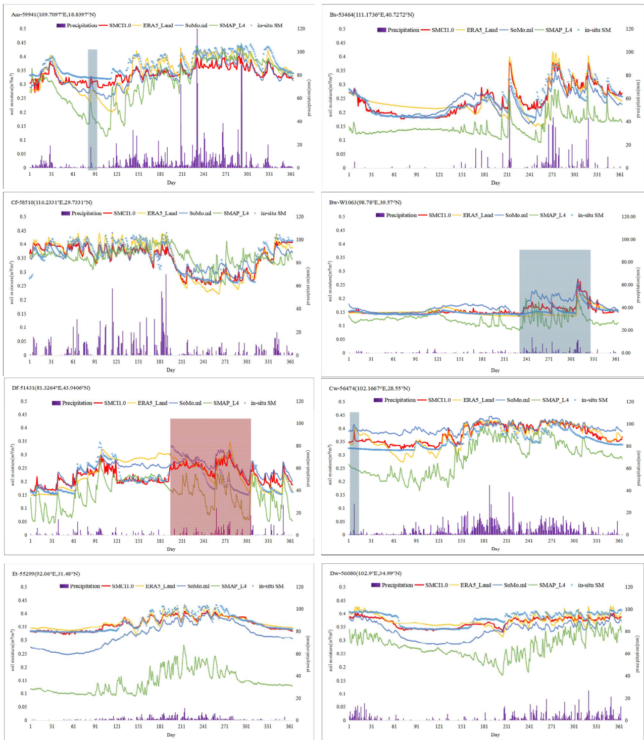
Figure 5: Time series of in-situ and estimated SM by RF model at 10 cm soil depth along with daily precipitation in different climatic zones.
