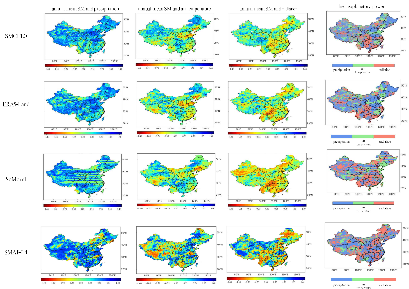
725 Figure 9: Partial correlation coefficients between annual mean SM and precipitation (the first column), air temperature (the second column), and radiation (the third column) for the different gridded SM products. The fourth column represents best explanatory power (highest absolute partial correlation) for the interannual variability in SM for the different gridded SM products.
