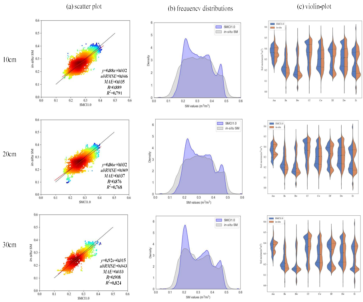
695 Figure 2: Comparisons between SMCI1.0 and in-situ SM from 10 to 30 cm soil depth in year-to-year experiment: comparison of (a) the scatter plot between the mean of SMCI1.0 and that of in-situ SM at each station, (b) the frequency distributions of all SM values in SMCI1.0 and that in in-situ measurements, (c) the violin-plot for the distribution of daily SM from stations for each climate type.
