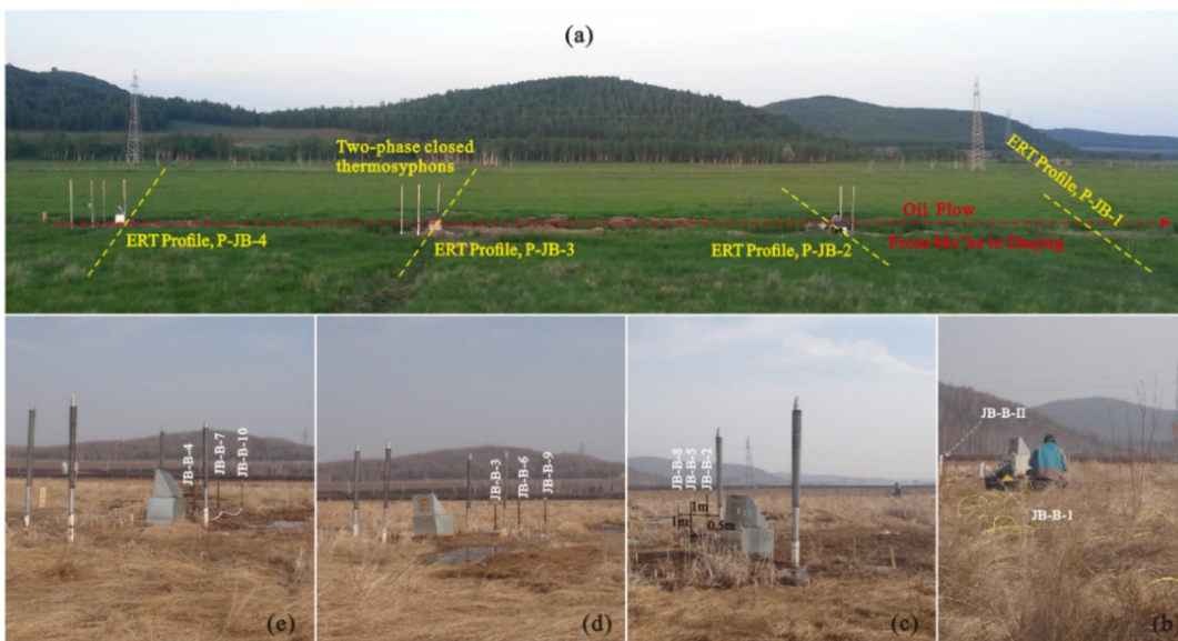
515 516 Figure C2. Position of boreholes drilled on and off the pipeline ROW and the ERT profile at the SL permafrost site. 517 Notes: (a). Photo was taken on 30 March 2018. The ground surface within the trench is completely covered with ice and 518 snow. (b) Miniature temperature data loggers were installed in August 2020. Photo was taken on 17 April 2021. The 519 surface vegetation was destroyed by a controlled burn.
