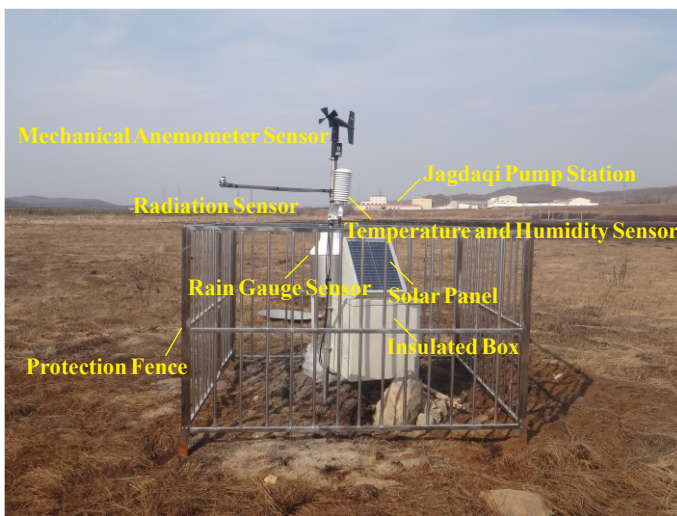
501 502 Figure B1. The automated weather station and instrumentations at the JB site along the China-Russia Crude Oil Pipelines 503 route in the northern Da Xing'anling Mountains, Northeast China. Notes: Photo was taken on April 2018. The rain gauge 504 sensor has been installed but is ineffective. The photo shows the location of the Jagdaqi pump station. The CR3000 data 505 logger, multiplexer, battery cell, solar charge controller, and wireless transmission module are placed in the white box 506 with a solar panel ( i.e. , insulated box). All monitoring devices are protected by an aluminum alloy fence.
