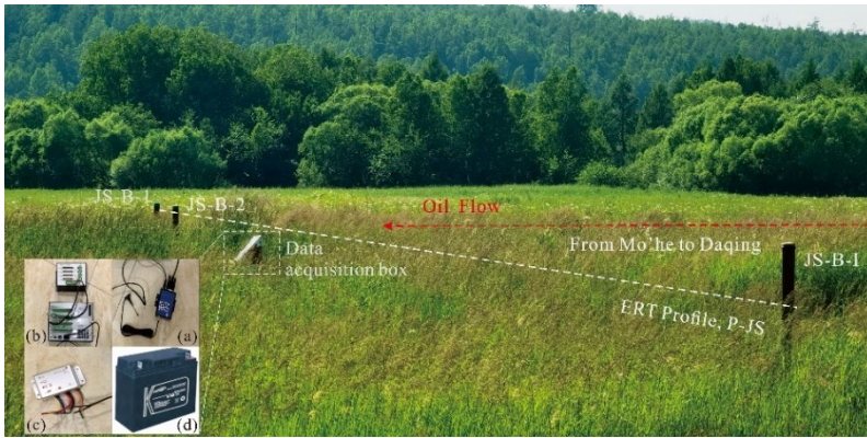
509 510 Figure C1. Position of boreholes drilled on and off the pipeline ROW and the ERT profile at the JS permafrost site. Photo 511 was taken on 29 June 2021. Ground temperatures are measured using thermistor chains connected to the CR3000 data 512 logger. Notes: (a) Wireless transmission module (HKT-DTU, Campbell Scientific, Inc., USA), (b) CR3000 data logger 513 with a TRM128 multiplexer, (c) Solar charge controller (Phocos ECO (10 A), Germany), (d) Battery cell, a part of the 514 power supply device.
