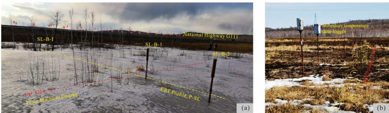
515 516 Figure C2. Position of boreholes drilled on and off the pipeline ROW and the ERT profile at the SL permafrost site. 517 Notes: (a). Photo was taken on 30 March 2018. The ground surface within the trench is completely covered with ice and 518 snow. (b) Miniature temperature data loggers were installed in August 2020. Photo was taken on 17 April 2021. The 519 surface vegetation was destroyed by a controlled burn.
