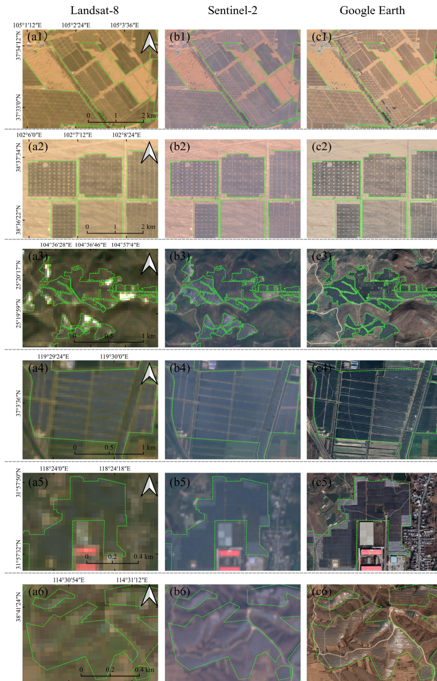
Figure 2. The visual interpretation examples (six sites) from (a) Landsat-8, (b) Sentinel-2, and (c) Google earth RGB true-color images. The green dashed line is the boundary of PV panels. © Google Earth 2021.
