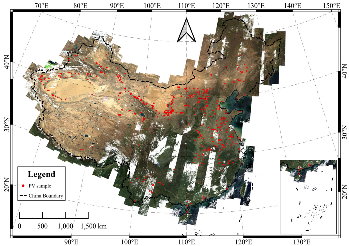
Figure 1. The composite image from Landsat-8 imagery during autumn 2020 (background) and PV samples of training and validation (red regions) in this study.
