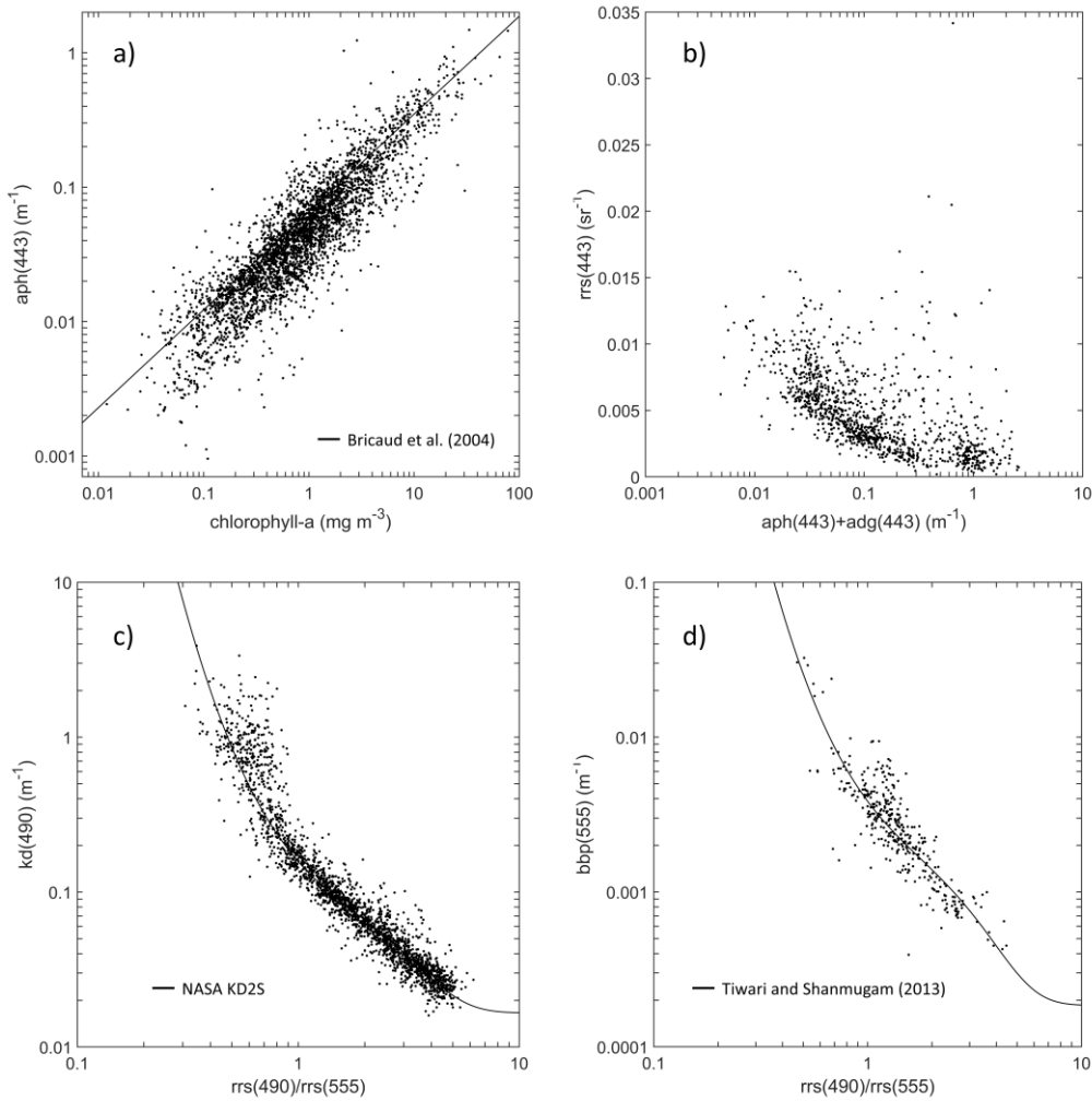
Figure 16. Examples of bio-optical relationships in the final merged table: (a) \text{aph}(443) versus chlorophyll-a. Total number of points ( 2,953,387 ) is divided between AWI ( 334,753 ), COASTCOLOUR (335), MERMAID (214), NOMAD (991), SeaBASS ( 124,139 ) and TPSS (955). For reference the solid line show the regression from Bricaud et al. (2004). (b) [\text{aph}(443) + \text{adg}(443)] versus \text{rrs}(443) . Total number of points (1,112) is divided between MERMAID (33) and NOMAD (1,079). (c) [\text{rrs}(490)/\text{rrs}(555)] versus \text{kd}(490) . The total number of points (2,280) is divided between MERMAID (62), NOMAD (2,117) and SeaBASS (101). For reference the solid line show the NASA KD2S standard algorithm ( http://oceancolor.gsfc.nasa.gov/cms/atbd/kd_490 ). (d) [\text{rrs}(490)/\text{rrs}(555)] versus \text{bbp}(555) . The total number of points (365) is divided between MERMAID (33), NOMAD (324), COASTCOLOUR ( 4 ) and SeaBASS (4). For reference the solid line show the relation proposed by Tiwari and Shanmugam (2013). A search window of 2 nm was used for (a) and (b), and a search window of 5 nm was used for (c) and (d) to include data at 560 nm when not available at 555 nm.
