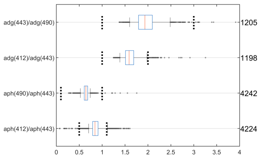
Figure 13. The distribution of absorption coefficients band ratios: adg(443)/adg(490), adg(412)/adg(443), aph(490)/aph(443) and aph(412)/aph(443). Data within 2 nm of the wavelengths were used. The graphical convention is identical to Fig. 2. The vertical dashed lines show the lower and upper thresholds used for quality control in the IOCCG report 5. The total number of points for “adg” ratios are divided between NOMAD (89%), COASTCOLOUR (7%), MERMAID (3%) and Seabass (1%). The total number of points for “aph” ratios are divided between NOMAD ( 3628 %), TPSS ( 2923 %), COASTCOLOUR (18%), AWI ( 1423 %), COASTCOLOUR (14%), SeaBASS (10%) and MERMAID (2%) and Seabass (1%).
