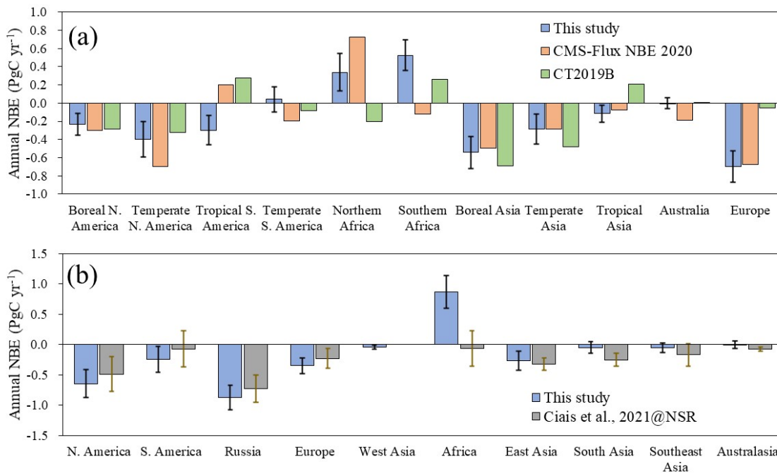
990 Figure 6: 2010-2019 averaged regional NBE in a) the TRANSCOM regions, and b) the RECCAP2 regions, both CMS-Flux NBE 2020 and CT2019B are averaged from 2010 to 2018, the result of Ciaia et al. (2021) is a bottom-up estimate, which is for the period of 2000-2009.
