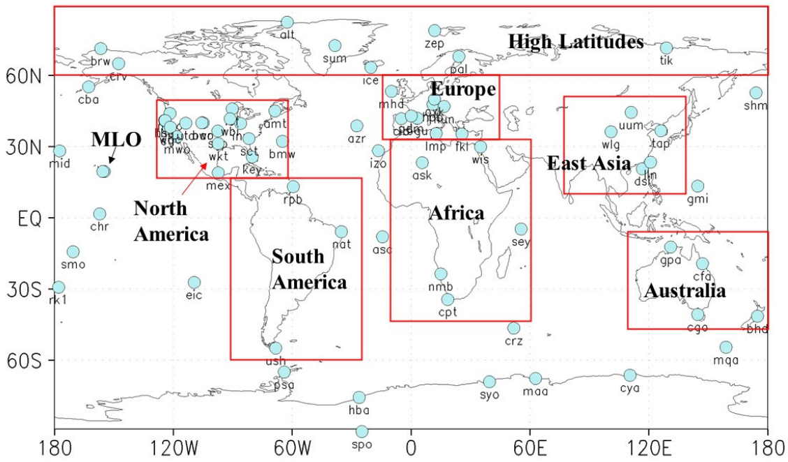
975 Figure 1: Distributions of the surface flask observation sites used in this study.
