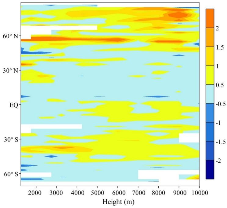
1015 Figure 13: BIAS at different latitudes and heights against the HIPPO observations.
