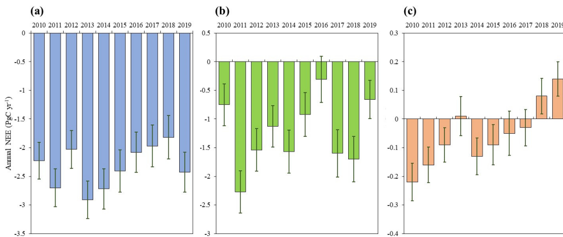
995 Figure 7: Interannual variations of annual NEE of different latitudes (a, northern mid-high latitudes (> 30° N); b, tropical latitudes (30° S ~ 30° N); c, southern middle latitudes (<30° S)).
