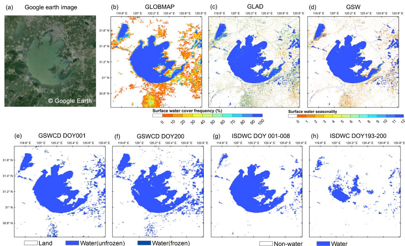
Figure 3. Comparison of surface water map of GLOBMAP SWF, GLAD, GSW, GSWCD and ISDWC in frequently cloud covered areas around Taihu Lake in eastern China ( 30.62^{\circ} N- 31.78^{\circ} N, 119.66^{\circ} E- 120.82^{\circ} E) in 2015. (a) Google Earth high-resolution image (from Google Earth); (b) GLOBMAP surface water cover frequency; (c) GLAD annual water percent; (d) GSW seasonality (Source: EC JRC/Google); surface water extent of GSWCD in (e) DOY001 and (f) DOY200 in 2015; surface water extent of ISDWC in (g) DOY001-008 and (h) DOY193-200 in 2015.
