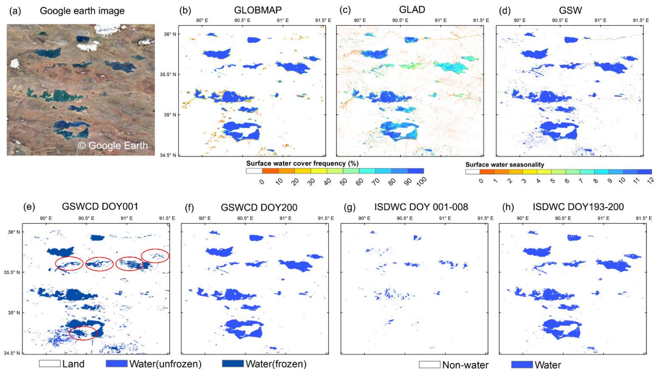
330 Figure 4. Comparison of surface water map of GLOBMAP SWF, GLAD, GSW, GSWCD and ISDWC for frozen lakes over bright surface in northeastern Tibetan Plateau (34.48° N-36.10° N, 89.71° E-91.53° E) in 2015. (a) Google Earth high-resolution image (from Google Earth); (b) GLOBMAP surface water cover frequency map; (c) GLAD annual water percent; (d) GSW seasonality (Source: EC JRC/Google); surface water extent of GSWCD in (e) DOY001 and (f) DOY200 in 2015; surface water extent of ISDWC in (g) 335 DOY001-008 and (h) DOY193-200 in 2015.
