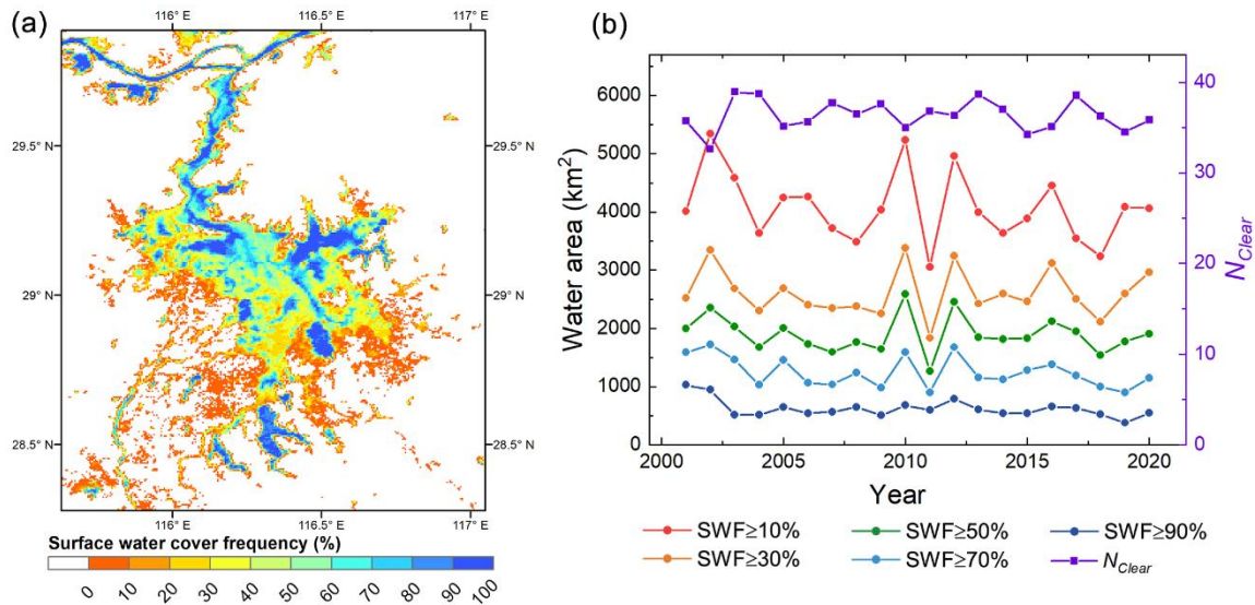
Figure 9. The seasonal variation and interannual change of surface water cover of Poyang Lake (28.28°N-29.89°N, 115.62°E-117.05°E). (a) The GLOBMAP SWF map in 2020; (b) The interannual variation of the area of Poyang Lake with different inundation frequency and average value of available clear-sky observations count ( N_{Clear} ) over the maximum surface water extent from 2001 to 2020.
