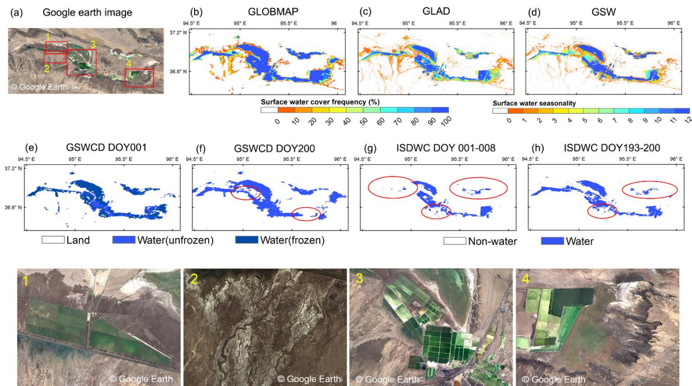
350 Figure 5. Comparison of surface water map of GLOBMAP SWF, GLAD, GSW, GSWCD and ISDWC for saline lake in Qarhan Salt Lake in the southern Qaidam Basin in northwestern China ( 36.56^{\circ} N- 37.24^{\circ} N, 94.48^{\circ} E- 96.08^{\circ} E) in 2015. (a) Google Earth high-resolution image (from Google Earth); (b) GLOBMAP surface water cover frequency; (c) GLAD annual water percent; (d) GSW seasonality (Source: EC JRC/Google); surface water extent of GSWCD in (e) DOY001 and (f) DOY200 in 2015; surface water extent of ISDWC in (g) DOY001-008 and (h) DOY193-200 in 2015. The last row shows the Google Earth high-resolution images for the four subregions shown with the red circles in Fig. 6a (from Google Earth).
