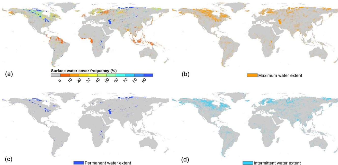
290 Figure 2. Global distribution of surface water cover frequency in 2020. (a) global SWF map; (b) the maximum surface water extent, (c) the permanent surface water extent and (d) the intermittent surface water extent. The SWF was aggregated to 10×10 km grids by averaging the valid SWF in each grid for visualization.
