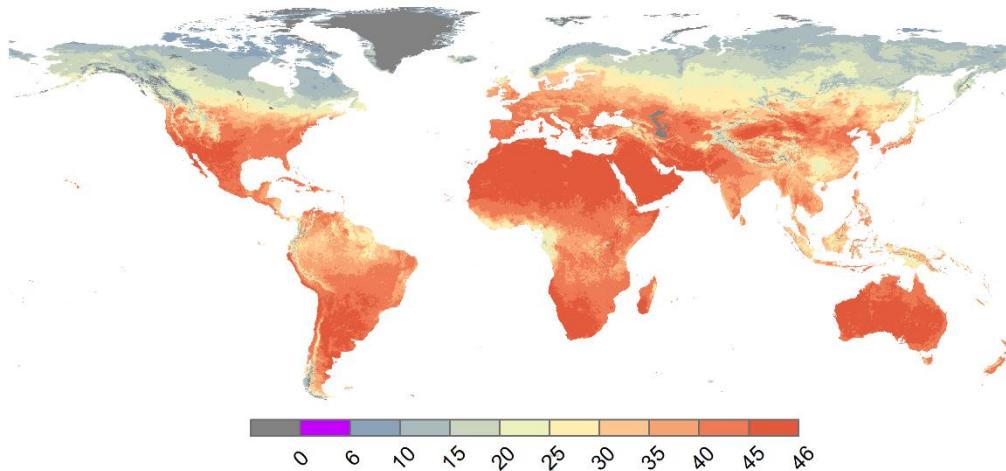
Figure 10. Global map of the number of clear-sky snow/ice-free MOD09A1 observation in 2020
