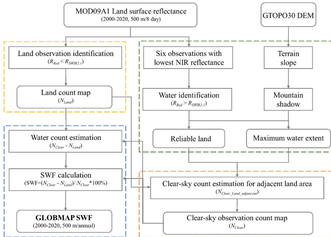
Figure 1. Workflow of the method for generating GLOBMAP surface water cover frequency dataset.
