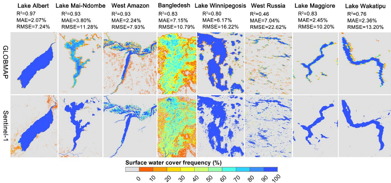
395 Figure 6. Comparison of GLOBMAP SWF against SWF maps derived from Sentinel-1 in four-eight regions. These include Lake Albert in the Democratic Republic of the Congo and Uganda (30.98° E, 1.74° N), Lake Mai-Ndombe in western Democratic Republic of the Congo (18.32° E, 2.07° S), River Amazon and River Taparus in western Amazon in Brazil (54.87° W, 2.16° S), and-wetland in western Bangladesh (91.12° E, 24.65° N), Lake Winnipegosis in Canada (99.91° W, 52.61° N), lakes in western Russia (31.00° E, 64.10° N), Lake Maggiore in Italy (8.65° E, 45.90° N), and Lake Wakatipu in New Zealand (168.55° E, 45.10° S). The linear regression results are 400 presented in the top of the figure.
