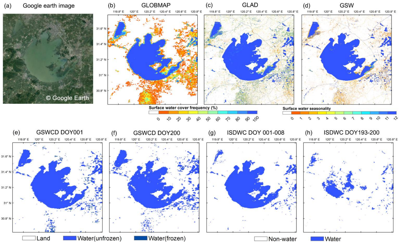
Figure 3. Comparison of surface water map of GLOBMAP SWF, GLAD , GSW , GSWCD and ISDWC in frequently cloud covered areas around Taihu Lake in eastern China (30.62° N-31.78° N, 119.66° E-120.82° E) in 2015 . (a) Google Earth high-resolution image (from Google Earth); (b) GLOBMAP surface water cover frequency in 2016 ; (c) GlobeLand30-GLAD annual water percent; aggregated 500 m-resolution water cover fraction in 2020 (d) GSW seasonality (Source: EC JRC/Google) ; surface water extent of GSWCD in (de) DOY001 and (ef) DOY200 in 2016 2015 ; surface water extent of ISDWC in (fg) DOY001-008 and (gh) DOY193-200 in 2015 16 .
