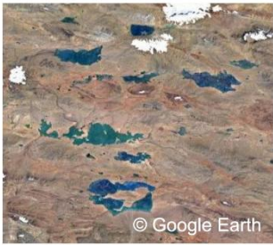
(a) Google earth image
