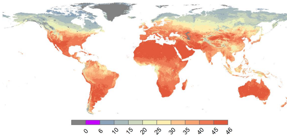
585 Figure 10. Global map of the number of clear-sky snow/ice-free MOD09A1 observation in 2020
