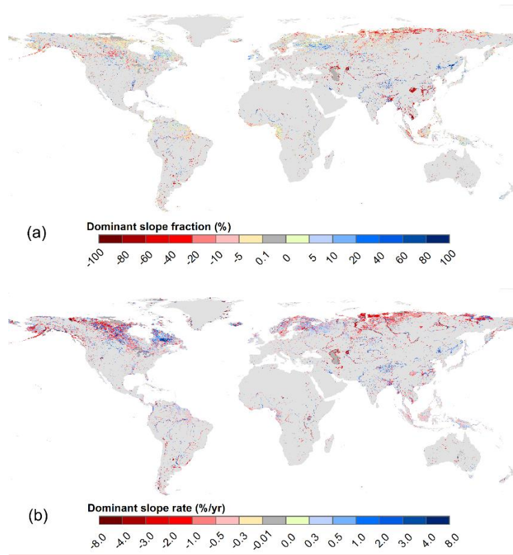
Figure 8. Linear trend of surface water cover frequency ( \%/yr ) during 2001 and 2020. The trend maps were aggregated to 10 km resolution for visualization. Percentage of pixels with (a) Dominant SWF slope fraction (%). The positive (negative) fraction means that the fraction of pixels with increasing (decreasing) SWF ( p < 0.05 ) in each 10 km grid, indicating whether the inundation frequency is dominantly increasing (decreasing). positive and (b) Dominant SWF change rate (%/yr). The positive (negative) slope rate means that the mean linear slope rate of pixels with increasing (decreasing) SWF ( p < 0.05 ) in each 10 km grid, whichever is faster, indicating whether the inundation frequency is increasing (decreasing) rapidly. negative slopes ( p < 0.05 ) in each 10 \times 10 km grid; Mean value of (c) positive and (d) negative slopes ( p < 0.05 ) in each 10 \times 10 km grid. The positive (negative) slope of Fig. 8c and 8d indicates whether the inundation frequency is increasing (decreasing). The light grey refers to non-water covered areas.
