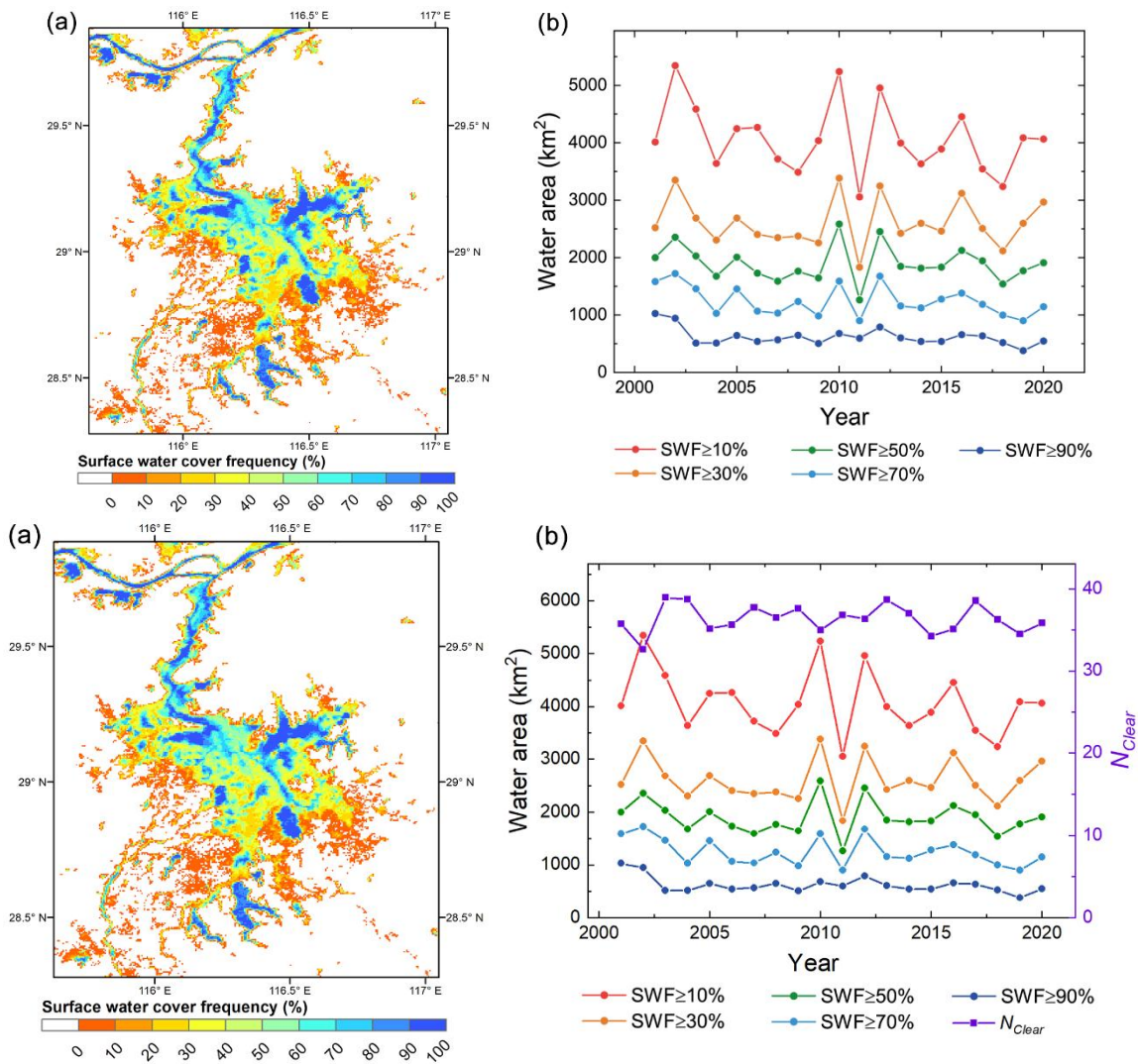
Figure 9. The seasonal variation and interannual change of surface water cover of Poyang Lake (28.28°N-29.89°N, 115.62°E-117.05°E). (a) The GLOBMAP SWF map in 2020; (b) The interannual variation of the area of Poyang Lake with different inundation frequency and average value of available clear-sky observations count ( N_{clear} ) over the maximum surface water extent from 2001 to 2020.
