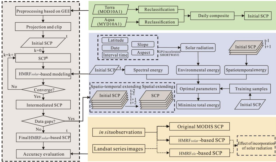
Figure 3: Overall flowchart of the \text{HMRF}_{\text{solar}} -based framework. (SCP stands for snow cover products)
