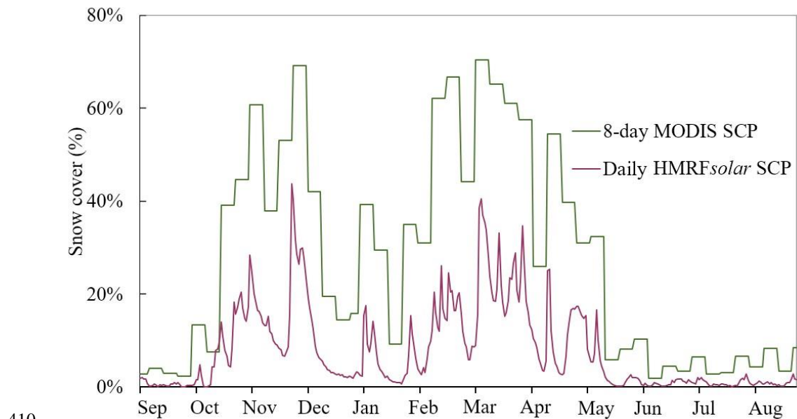
410 Figure 9: Snow cover percentage for daily HMRF solar -based snow cover products and 8-day composite MODIS snow products in a sample area during the 2017 snow season of the TP. (SCP stands for snow cover products.)
