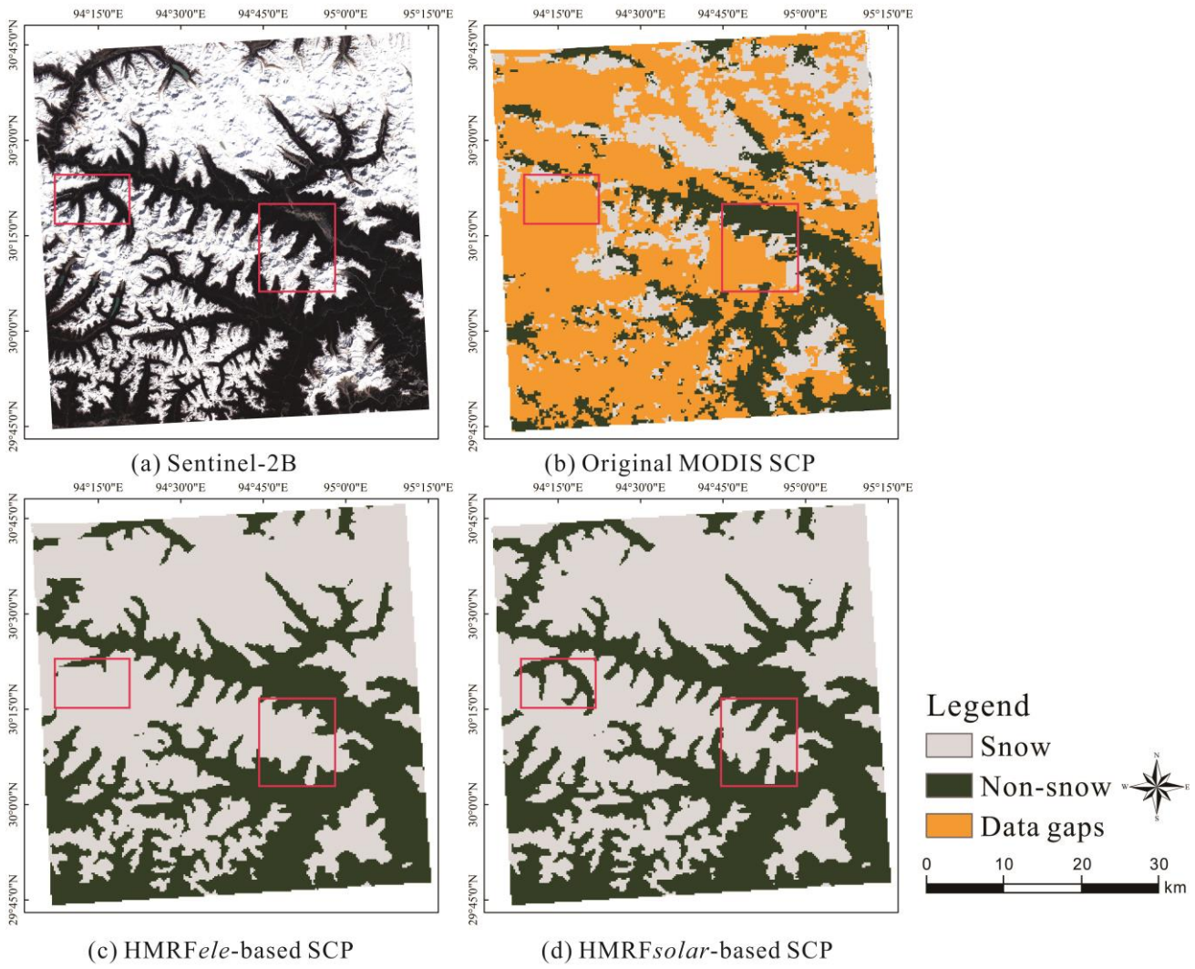
Figure 8: Comparison between true-color Sentinel-2B imagery and (a), original MODIS snow products (b), HMRFele-based snow products (c) and HMRFsolar-based snow products (d).
