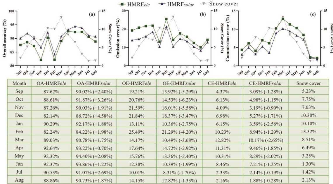
Figure 4: Temporal variations in OA (a), OE (b), and CE (c) of \text{HMRF}_{ele} - and \text{HMRF}_{solar} -based snow products from 2002–2021.
