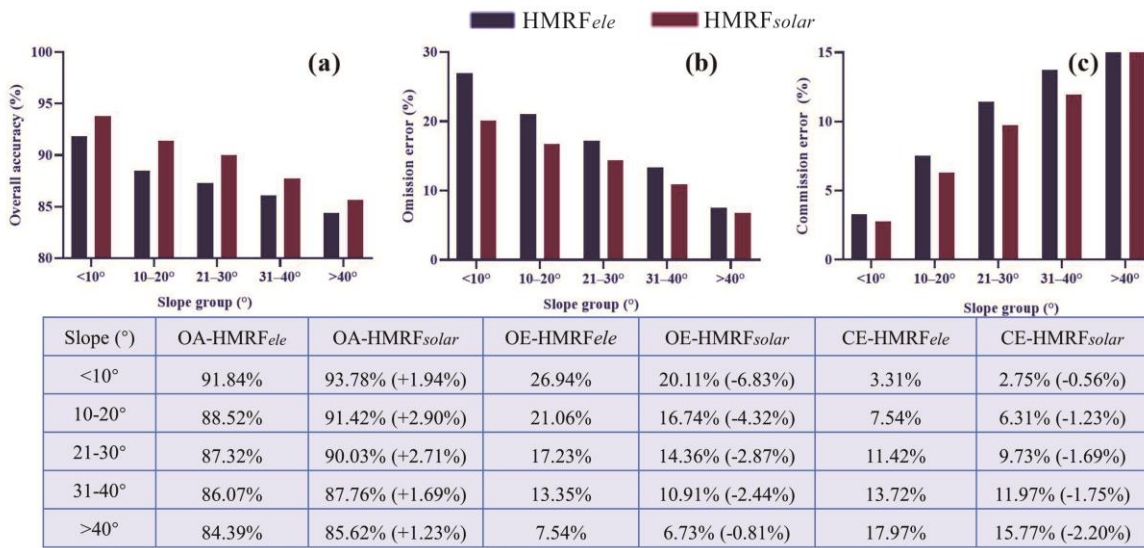
355 Figure 6: Effect of slope on OA (a), OE (b), and CE (c) of HMRFele- and HMRFsolar-based snow products from 2002–2021.
