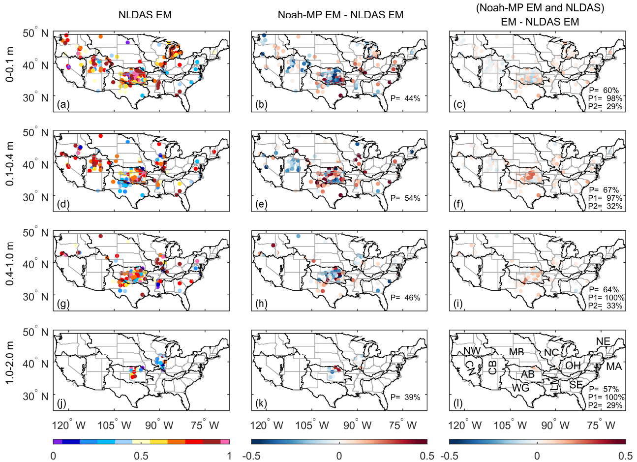
Figure 5. The first column shows the TSS of the NLDAS ensemble mean in simulating the annual cycle of soil moisture at different depths (0–0.1 m, 0.1–0.4 m, 0.4–1 m, 1–2 m). The second column presents the difference in TSS between the Noah-MP ensemble mean and the NLDAS ensemble mean. The third column depicts the TSS difference between the arithmetic average of the Noah-MP ensemble mean and the NLDAS models to the NLDAS three-model mean. P is the percentage of sites at which a higher TSS appears relative to the NLDAS ensemble mean. P1 ( P2 ) is the percentage of sites at which a higher TSS appear given that the Noah-MP ensemble mean outperforms (underperforms) the NLDAS ensemble mean. The evaluation period is 1996–2013.
