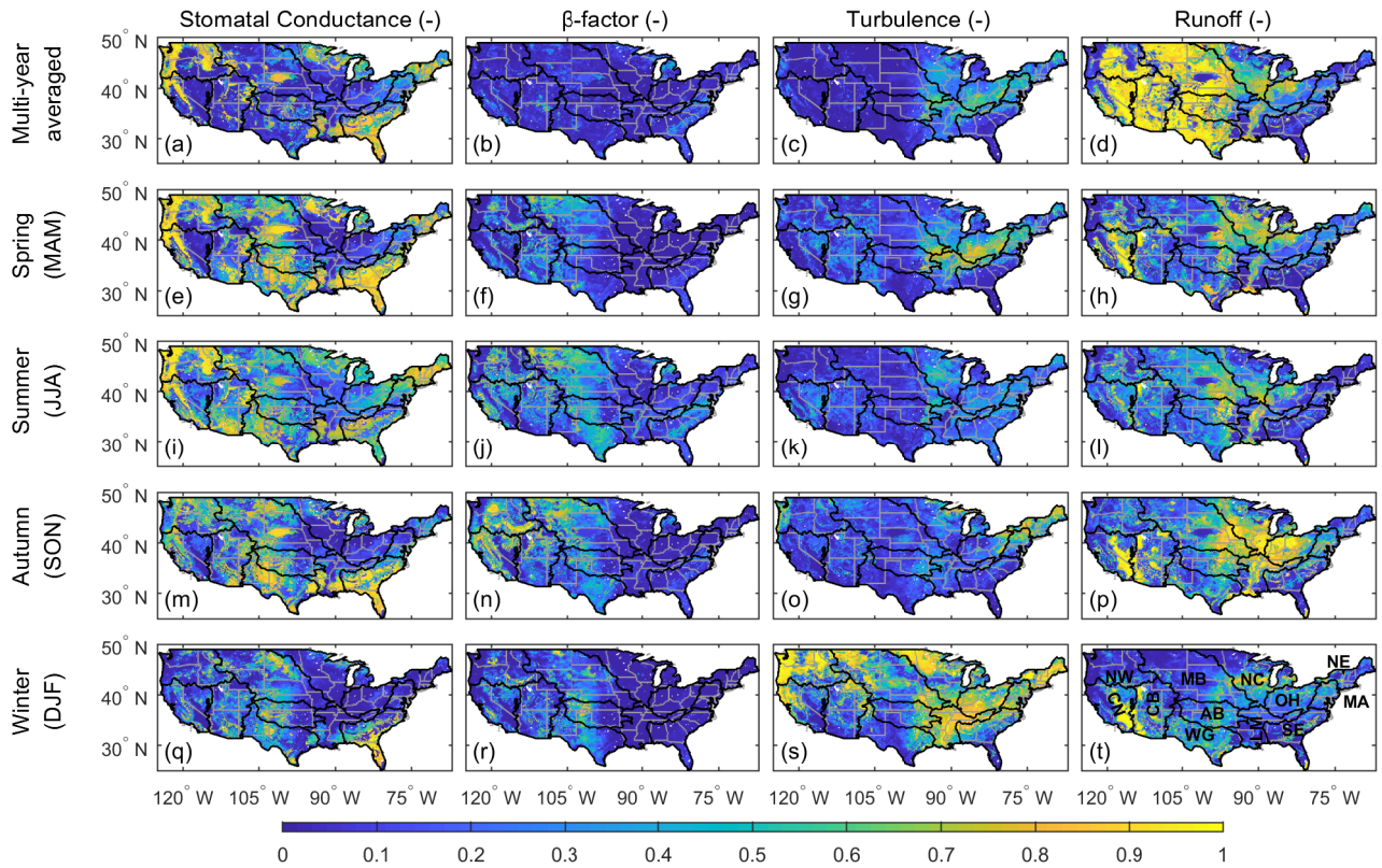
Figure 14. The Sobol' total sensitivity of the multi-year-averaged and seasonal (spring—MAM, summer—JJA, autumn—SON, winter—DJF) ET to the four parameterizations: stomatal conductance, soil moisture limitation to transpiration ( \beta -factor), turbulence, and runoff. Higher values indicate higher sensitivities.
