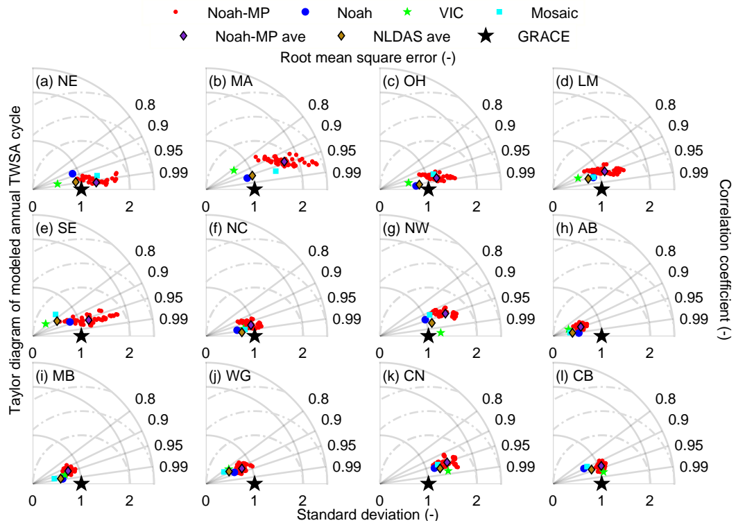
Figure 2. Taylor diagram of TWSA's annual cycle for the 48 Noah-MP configurations (red dots) and three NLDAS models (blue dots for Noah, green stars for VIC, and cyan square for Mosaic) at the twelve RFCs. Black stars denote the observations. The ensemble mean of Noah-MP and NLDAS is presented by purple and dark golden diamonds, respectively. The distance between the model and observation presents the nuRMSE. The radial lines show the correlation coefficient, while the distance to the origin along the line denotes the normalized variability.
