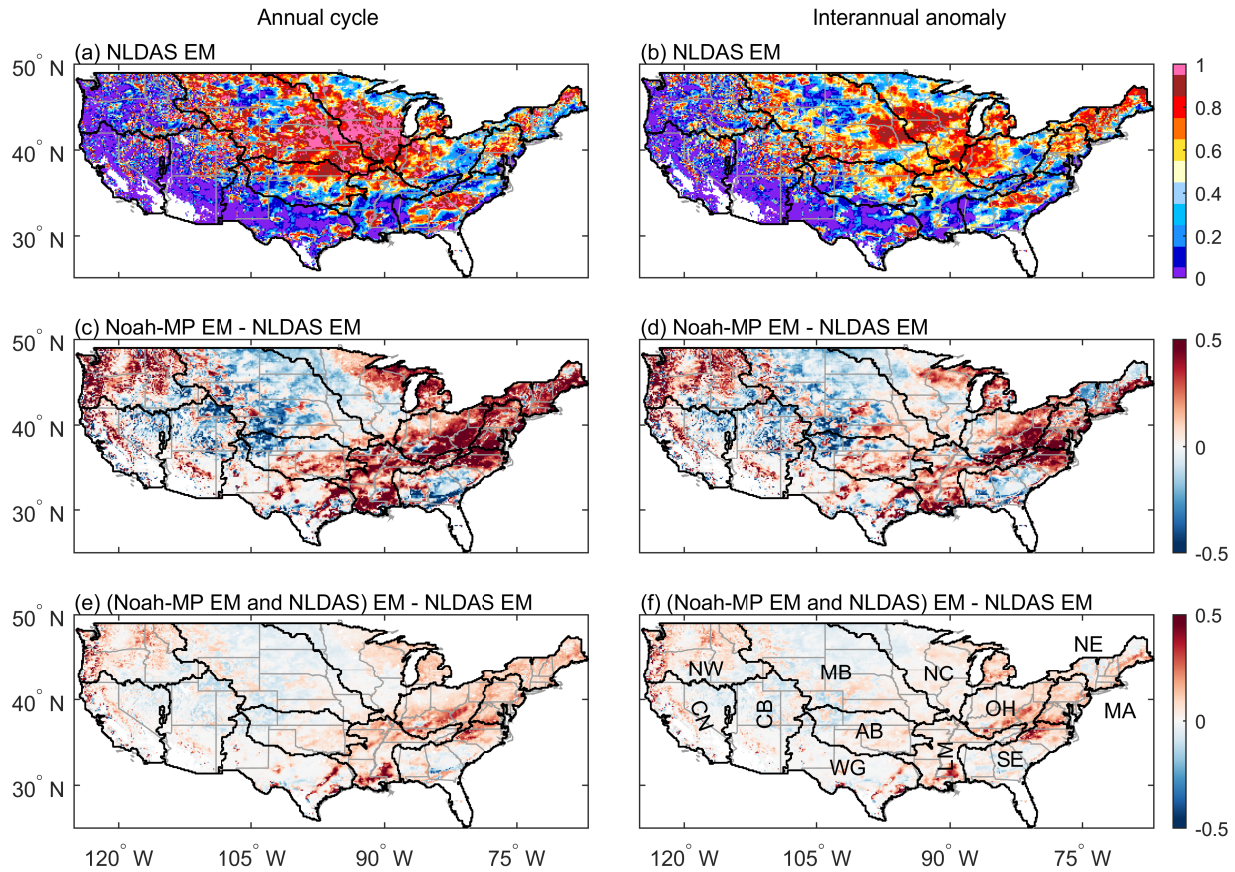
Figure 9. TSS of the ensemble means in simulating the annual cycle (left column) and interannual anomaly (right column) of SWE. (a) and (b) TSS of the NLDAS ensemble mean. (c) and (d) the difference in TSS between the Noah-MP ensemble mean and the NLDAS ensemble mean. (e) and (f) the difference between the arithmetic average of the Noah-MP ensemble mean and three NLDAS models to the NLDAS ensemble mean. The evaluation period is 2004–2015.
