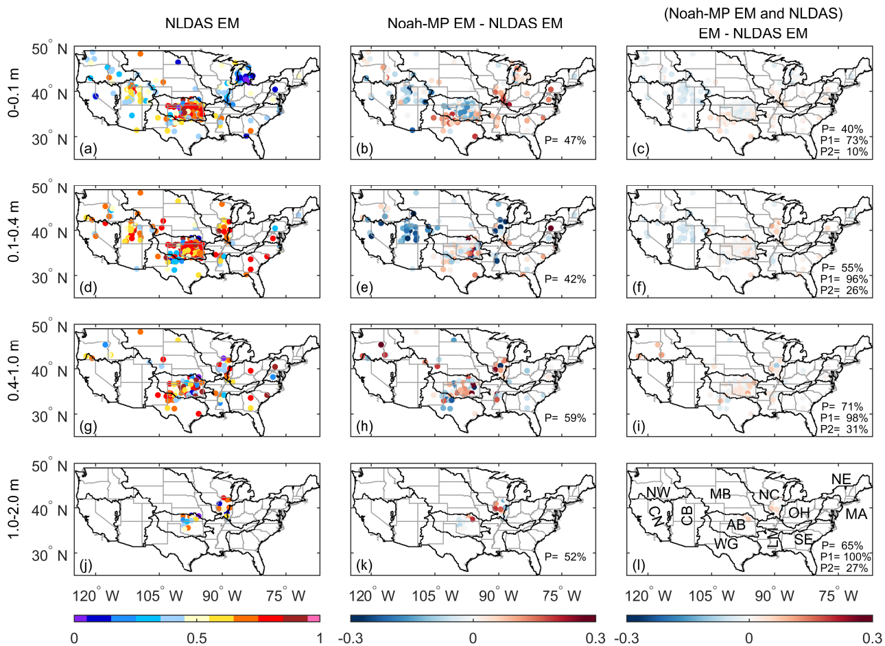
Figure 6. As in Figure 5, but for interannual anomaly.
