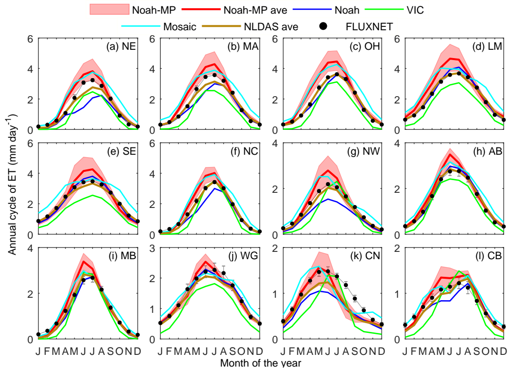
Figure 10. As in Figure 1, but for ET in the period of 1982–2011.
