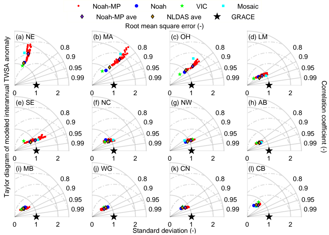
Figure 3. As in Figure 2, but for the interannual anomaly of TWSA.
