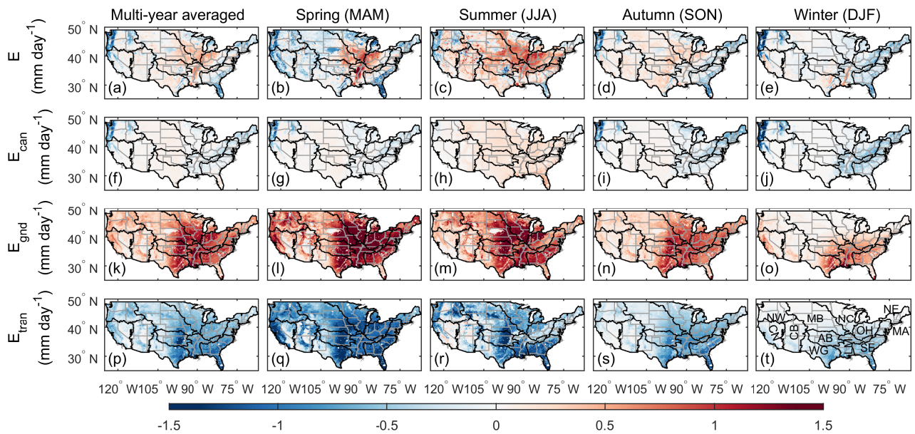
Figure 11. Differences between the Noah-MP ensemble mean and GLEAM in total ET ( E ), canopy evaporation ( E_{can} ), ground evaporation ( E_{gnd} ), and transpiration ( E_{tran} ). The units are \text{mm day}^{-1} .
