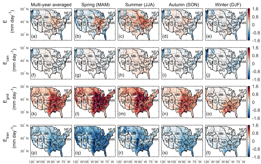
Figure 11. Differences between the Noah-MP ensemble mean and GLEAM in total ET ( E ), canopy evaporation ( E_{can} ), ground evaporation ( E_{gnd} ), and transpiration ( E_{tran} ). The units are \text{mm day}^{-1} .
