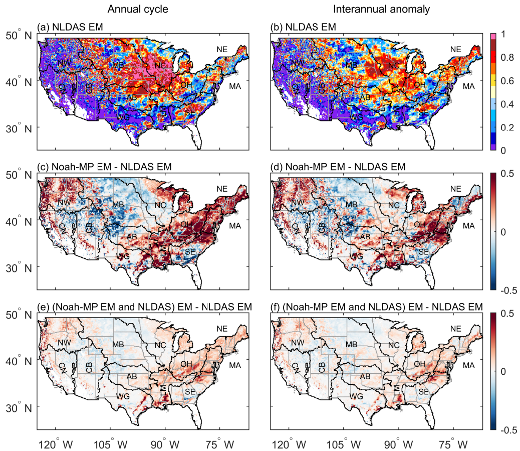
Figure 9. TSS of the ensemble means in simulating the annual cycle (left column) and interannual anomaly (right column) of SWE. (a) and (b) TSS of the NLDAS ensemble mean. (c) and (d) the difference in TSS between the Noah-MP ensemble mean and the NLDAS ensemble mean. (e) and (f) the difference between the arithmetic average of the Noah-MP ensemble mean and three NLDAS models to the NLDAS ensemble mean. The evaluation period is 2004–2015.
