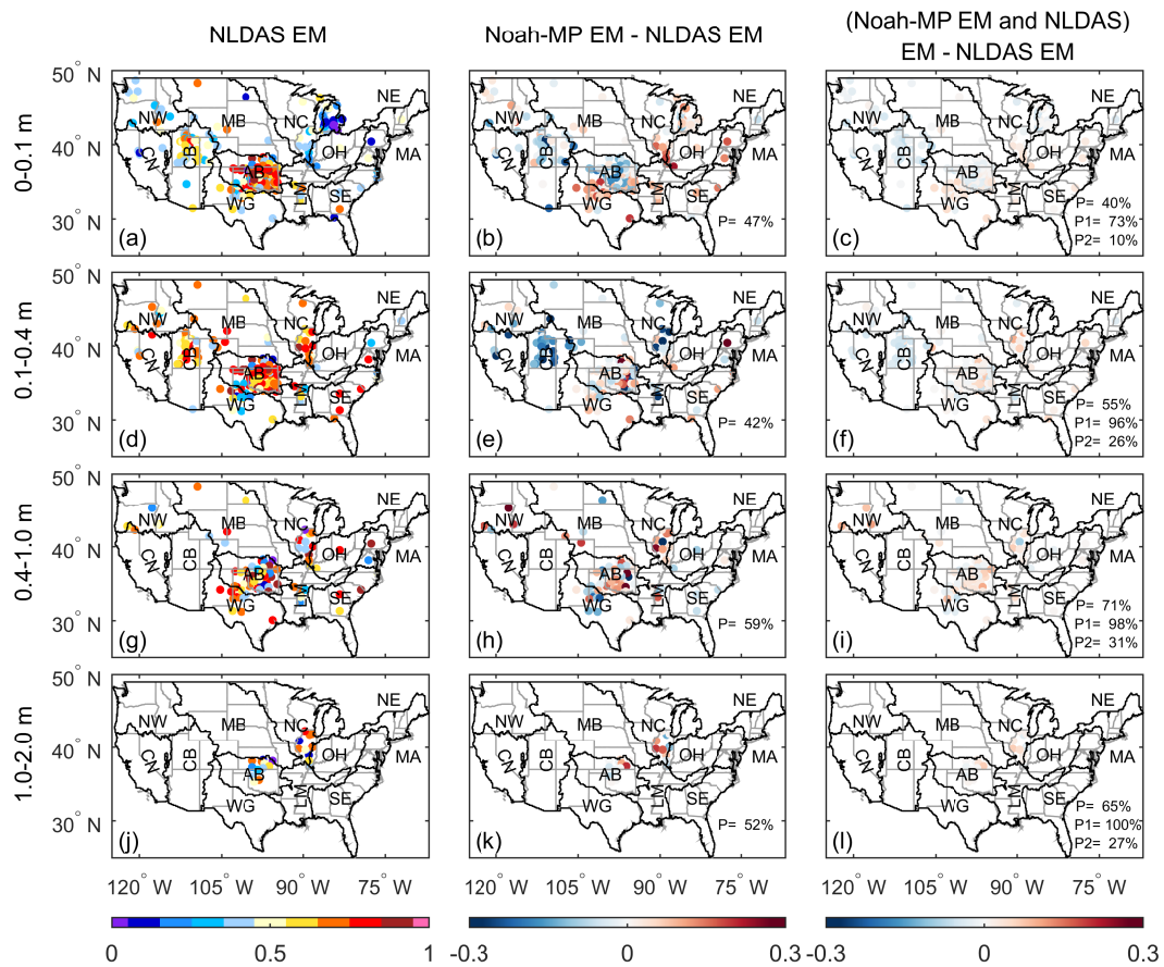
Figure 6. As in Figure 5, but for interannual anomaly.
