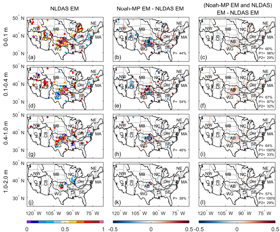
Figure 5. The first column shows the TSS of the NLDAS ensemble mean in simulating the annual cycle of soil moisture at different depths (0–0.1 m, 0.1–0.4 m, 0.4–1 m, 1–2 m). The second column presents the difference in TSS between the Noah-MP ensemble mean and the NLDAS ensemble mean. The third column depicts the TSS difference between the arithmetic average of the Noah-MP ensemble mean and the NLDAS models to the NLDAS three-model mean. P is the percentage of sites at which a higher TSS appears relative to the NLDAS ensemble mean. P1 ( P2 ) is the percentage of sites at which a higher TSS appear given that the Noah-MP ensemble mean outperforms (underperforms) the NLDAS ensemble mean. The evaluation period is 1996–2013.
