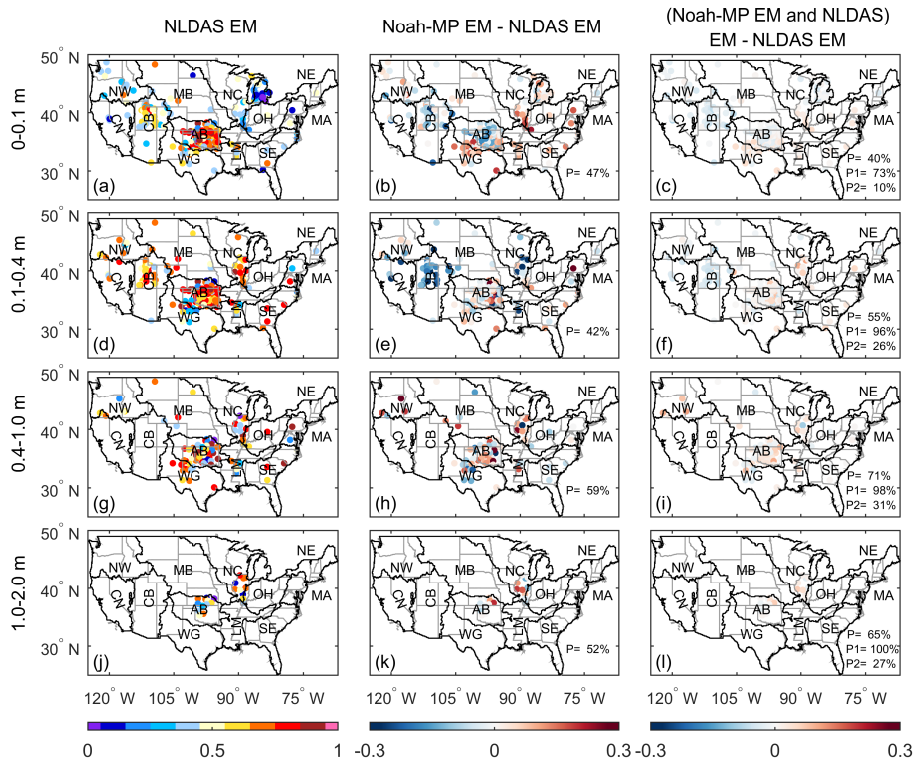
Figure 6. As in Figure 5, but for interannual anomaly.
