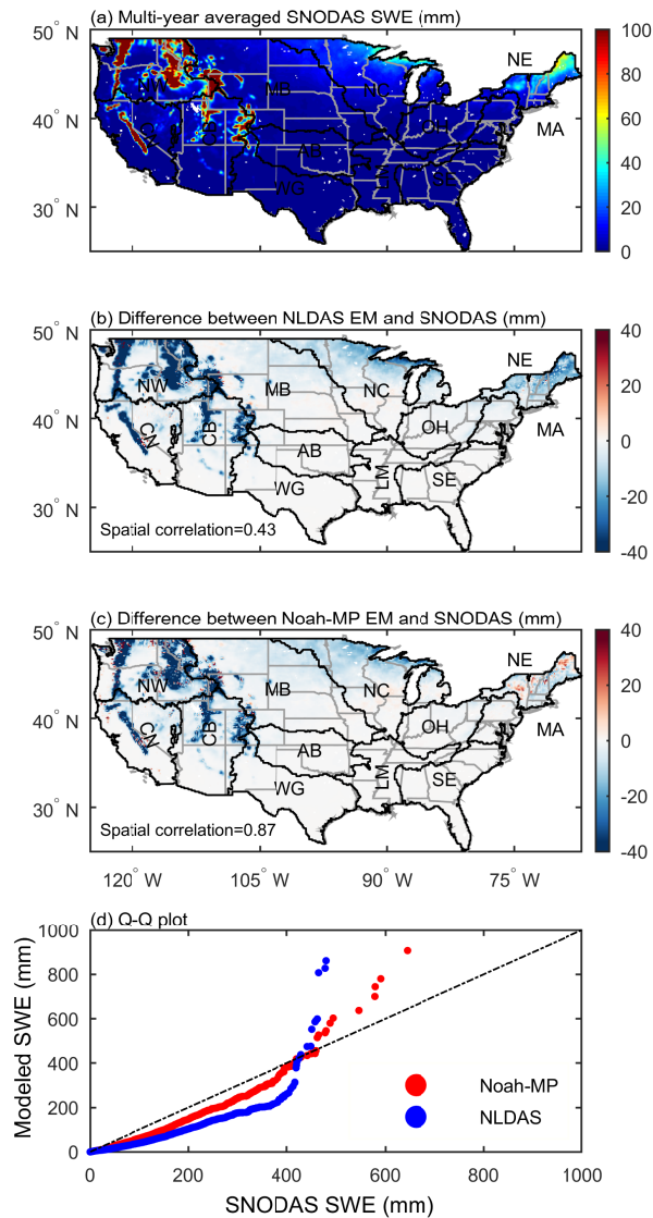
Figure 7. (a) Spatial distribution of the 11-year-averaged (September 2004 to August 2015) SWE from SNODAS. (b) Difference between the NLDAS ensemble mean and SNODAS. (c) Difference between the Noah-MP ensemble mean and SNODAS. The spatial correlation coefficients between the NLDAS/Noah-MP ensemble mean and SNODAS are also presented.
