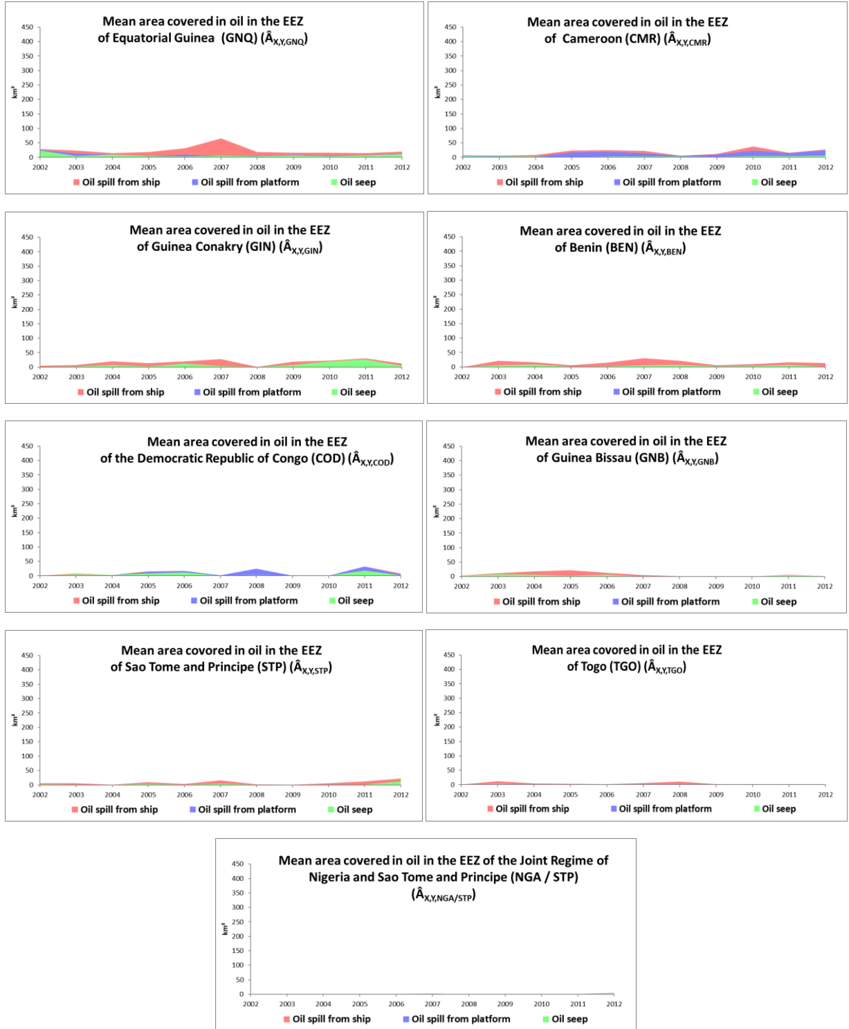
fig. 17 - Mean area covered in oil by EEZ of countries per year ( \hat{A}_{X,Y,EEZ} ).
