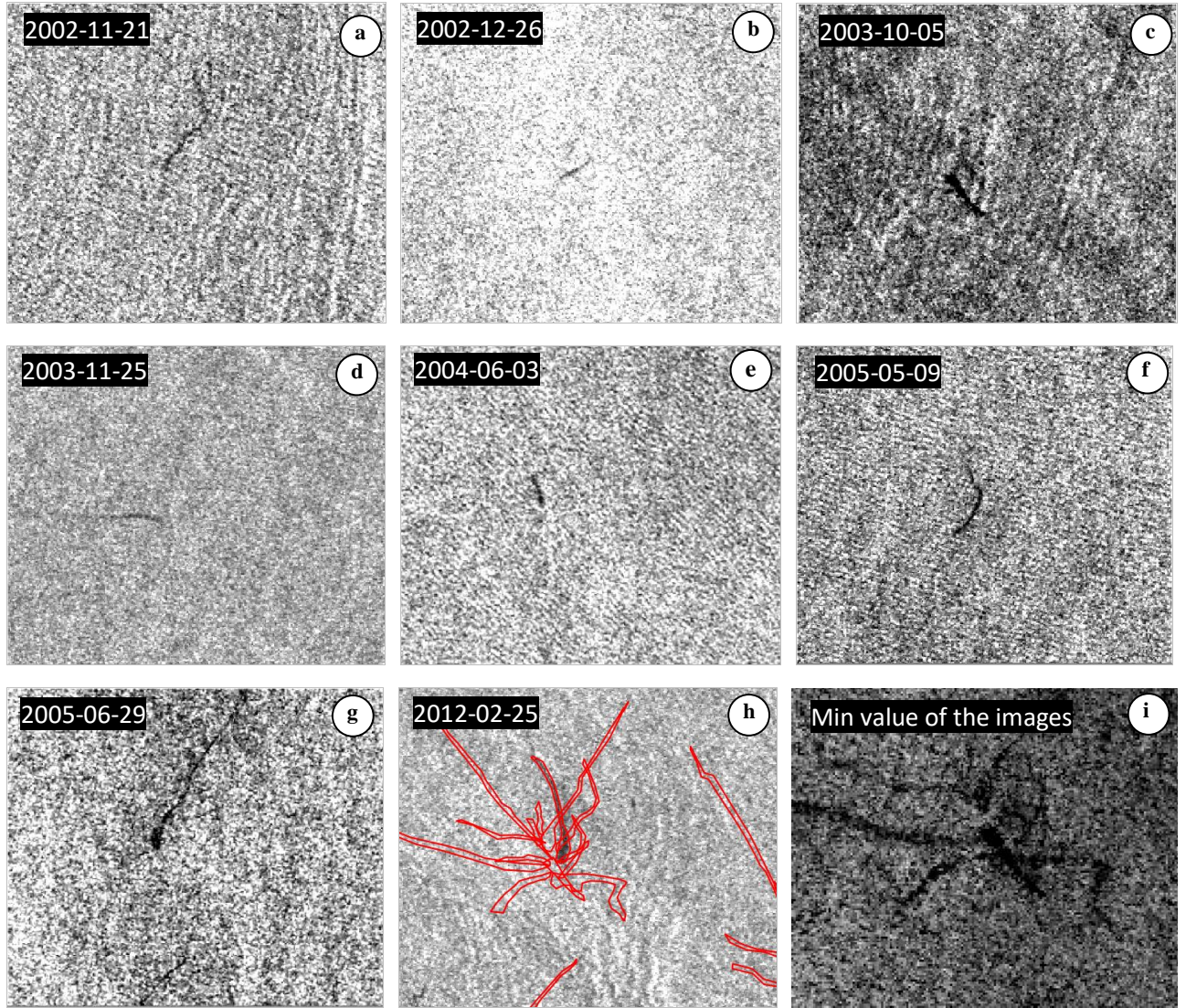
fig. 10 - Example of multitemporal analysis with astroseeps structure observed in the Lower Congo basin. Images a, b, c, d, e, f and g are Envisat ASAR images acquired at different dates with observed seeps. Image h shows an Envisat ASAR image with interpreted seeps. Image i shows the Envisat ASAR minimum image (i.e. each pixel is the minimum observed for the 7 dates) with an “astroseep” structure.
