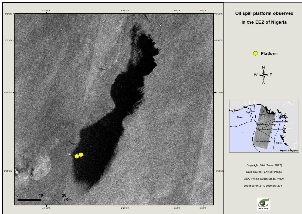
fig. 5 - Oil spill from platform observed in the EEZ of Nigeria (21/12/2011). The platforms are represented by the yellow dots (see hyperlook http://visioterra.org/ViWeb/hyperlook/504c7208cc184c12b42ed036bc9912f3 ).
