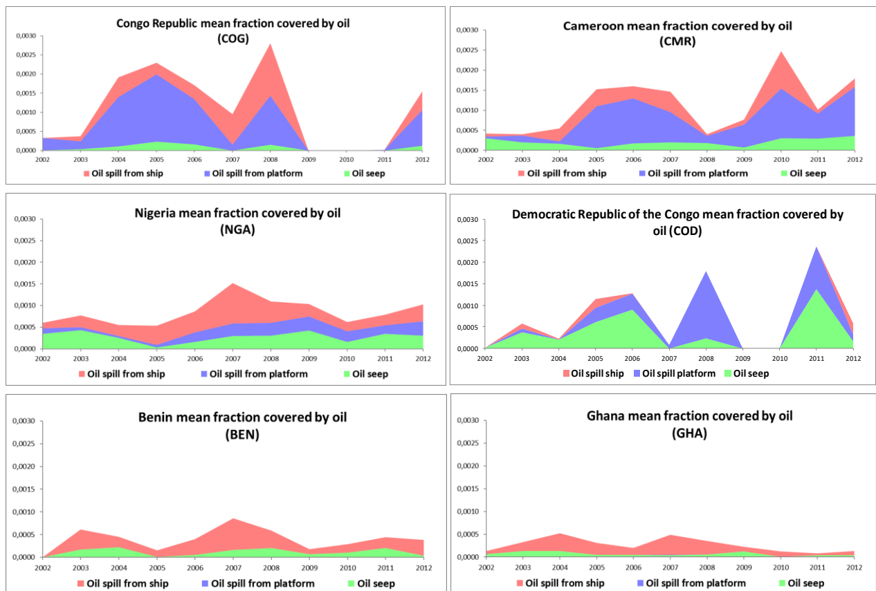
fig. 18 - Mean fraction covered by spilled oil by EEZ between 2002 and 2012.
