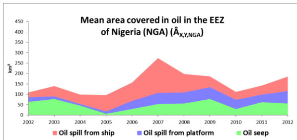
fig. 16 - Mean area covered in oil by EEZ of country ( \hat{A}_{X,Y} ) between 2002 and 2012.
