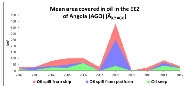
fig. 16 - Mean area covered in oil by EEZ of country ( \hat{A}_{X,Y} ) between 2002 and 2012.
