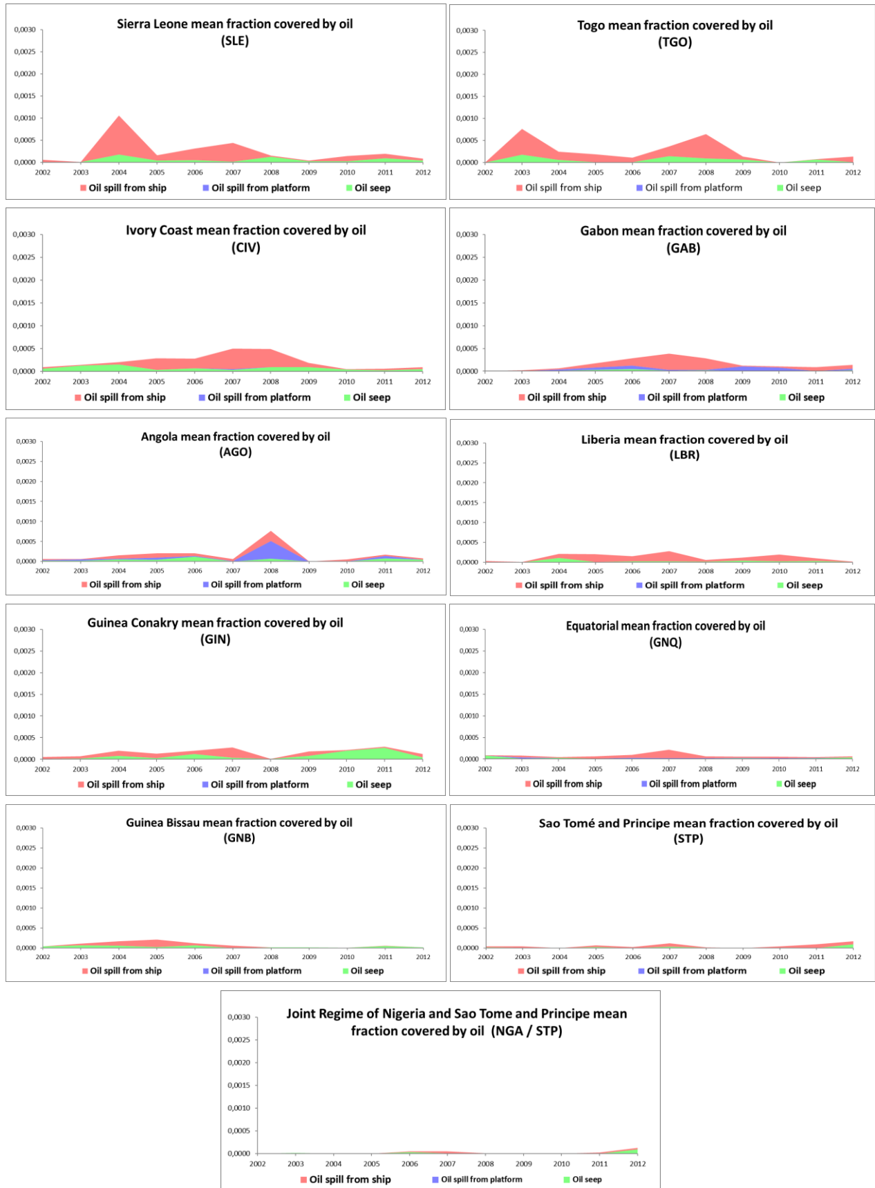
fig. 19 - Mean fraction covered by oil by EEZ by year.
