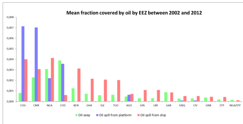
fig. 18 - Mean fraction covered by spilled oil by EEZ between 2002 and 2012.
