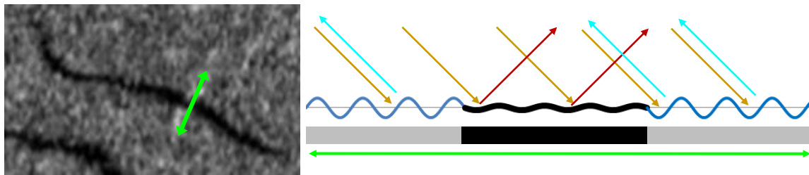
fig. 2 - Backscattering of the radar signal in the presence and absence of oil (Najoui, 2017).
