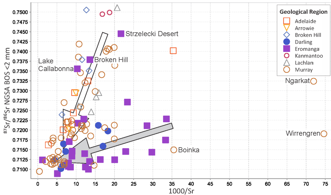
Figure 6: Scatterplot of ^{87}\text{Sr}/^{86}\text{Sr} vs 1000/\text{Sr} in the NGSa BOS <2 mm samples from the Darling-Curnamona-Delamerian (DCD) Sr isotope study area, grouped by main geological region each catchment is draining.
