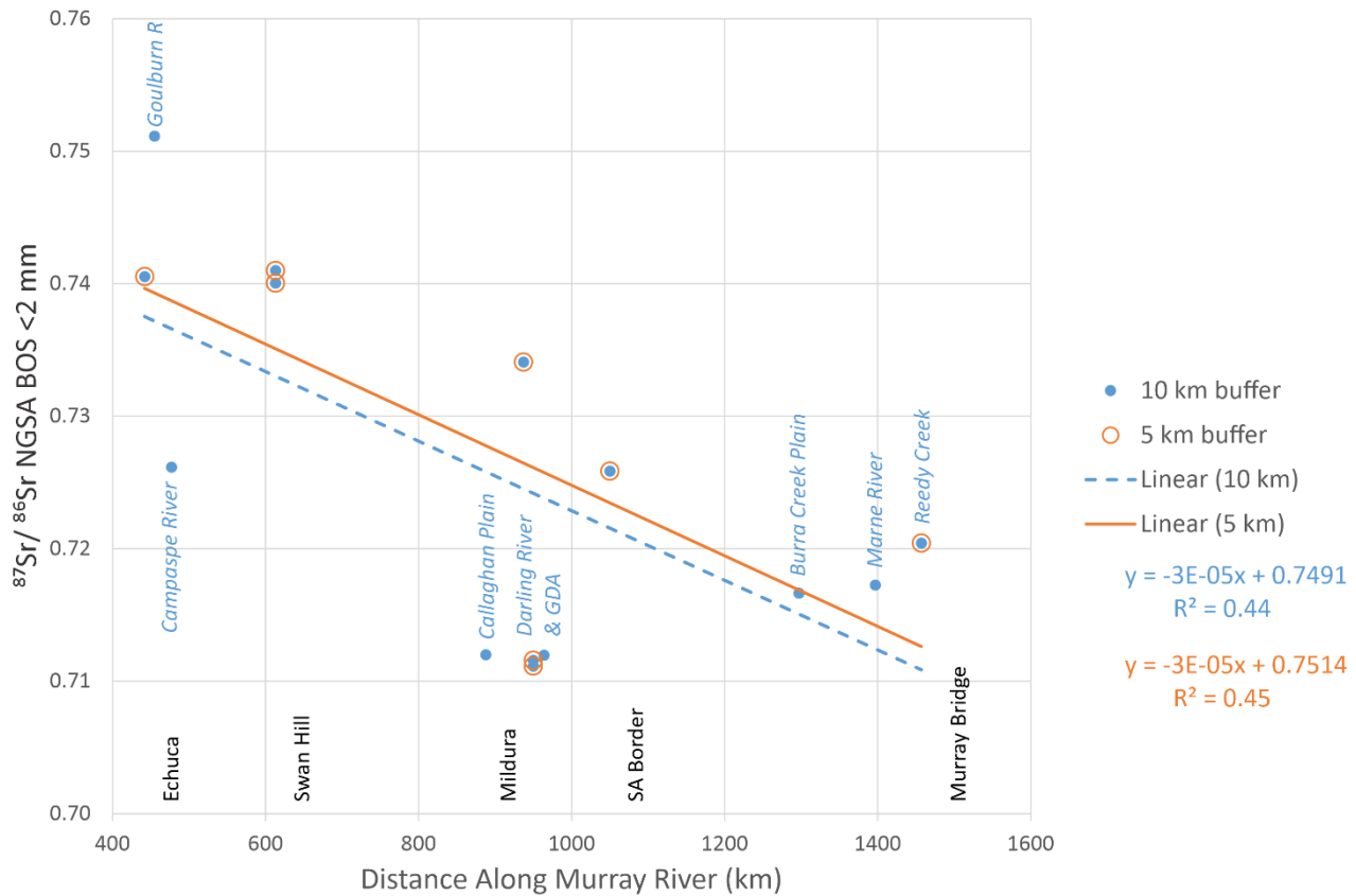
310 Figure 5: ^{87}\text{Sr}/^{86}\text{Sr} profile of NGSa catchment sediment at sampling sites located within 5 km and 10 km buffers of the Murray River (open and closed circles, respectively) vs downstream distance along the Murray River (east to west). Sites not directly sampling a Murray River catchment are labelled (in italics) with the name of the tributary (R = River; GDA = Great Darling Anabranch) or geomorphic entity. Least squares regression lines for the 5 km and 10 km buffers are shown as solid and dashed lines, respectively, and equations are given. Township and South Australia (SA) border positions are shown on the X-axis.
