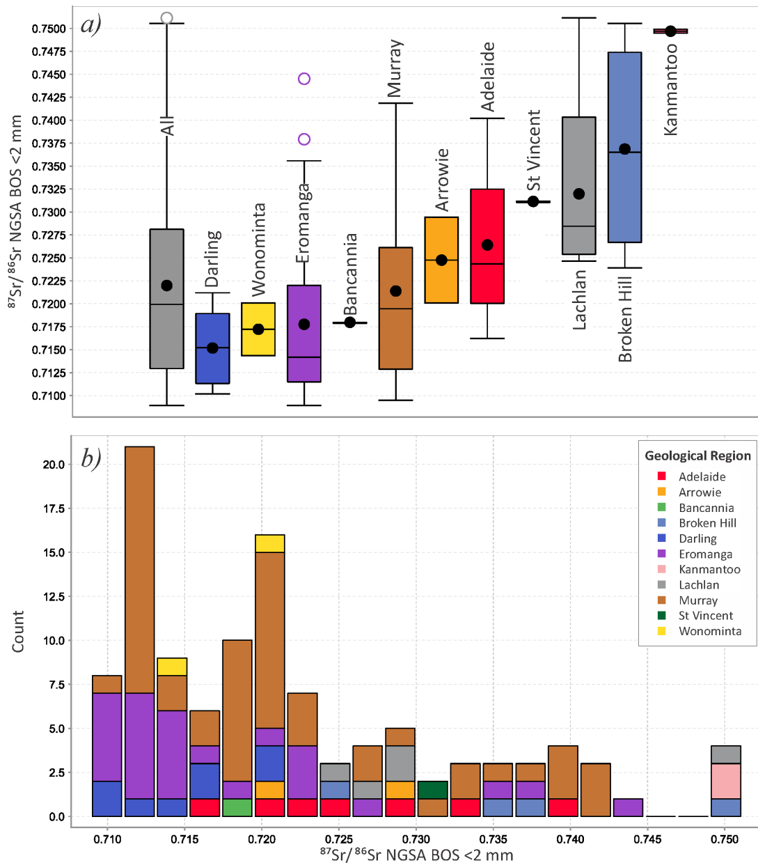
375 Figure 7: Univariate distribution representations of the ^{87}\text{Sr}/^{86}\text{Sr} data from the Darling-Curnamona-Delamerian (DCD) Sr isotope study area by geological region: (a) Tukey boxplots of, left to right, the whole dataset first (grey; n = 112 ), then sorted by increasing median (Darling, n = 8 ; Wonominta, n = 2 ; Eromanga, n = 26 ; Bancannia, n = 1 ; Murray, n = 54 ; Arrowie, n = 2 ; Adelaide, n = 7 ; St Vincent, n = 1 ; Lachlan, n = 5 ; Broken Hill, n = 4 ; and Kanmantoo, n = 2 , geological regions); (b) histogram by the above subgroups.
