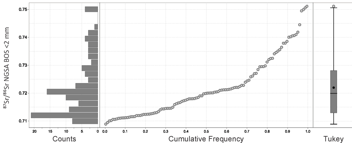
195 Figure 3: Univariate distribution of the ^{87}\text{Sr}/^{86}\text{Sr} data from the Darling-Curnamona-Delamerian (DCD) Sr isotope study area: (left) histogram (20 bins 0.002 wide); (middle) cumulative frequency plot; and (right) Tukey boxplot (mean = black dot).
