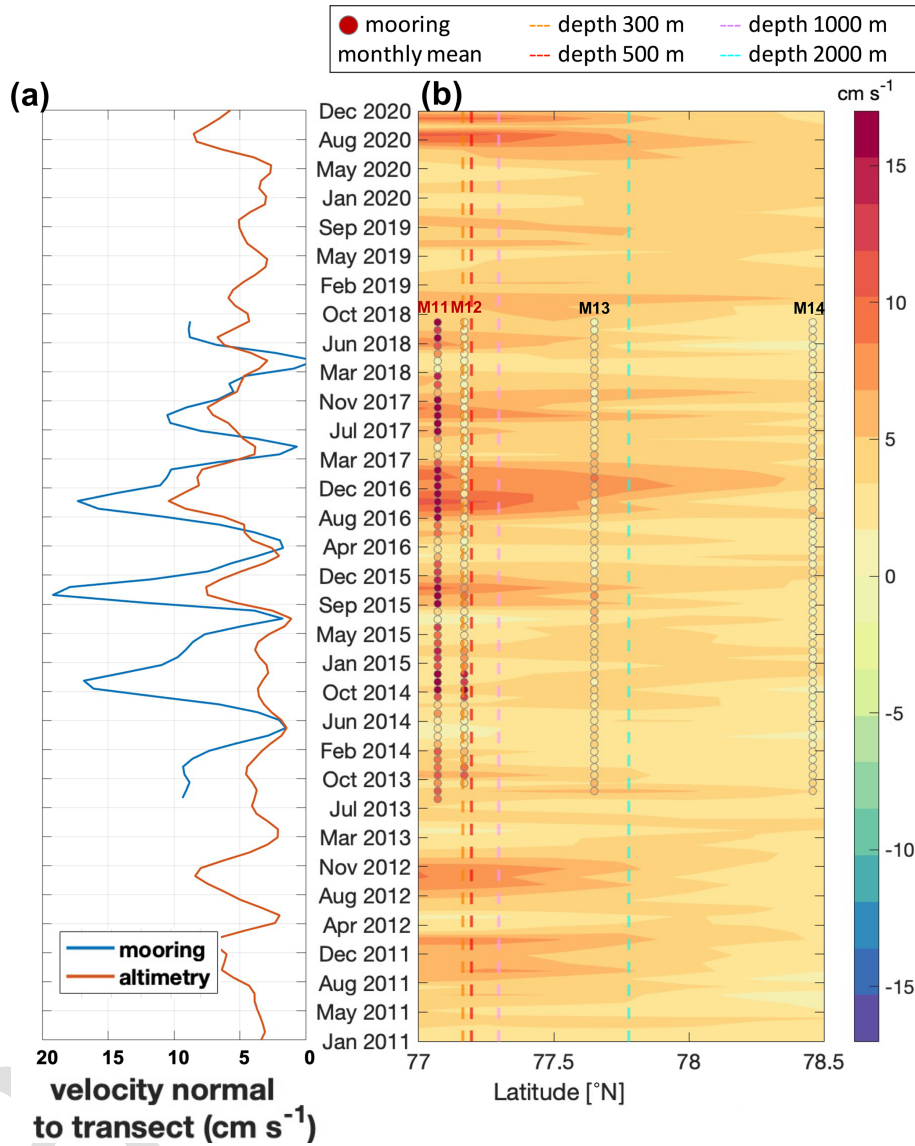
Figure 12. As in Fig. 11 but for velocities at the Laptev Sea continental slope, along longitude 126° 50' E (see Fig. 1). The component of the velocity normal to the transect is positive eastward. The time series in panel (a) correspond to test 4 (see text).
