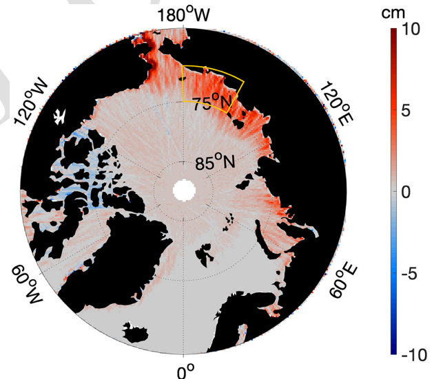
Figure B1. The along-track improvement in DAC correction, with respect to IB, in removing \eta' high-frequency variability. Colors indicate the difference between the standard deviation of along-track \eta' corrected with IB and corrected with DAC. The yellow square indicates the region of the East Siberian Sea where the frequency analysis was performed.
