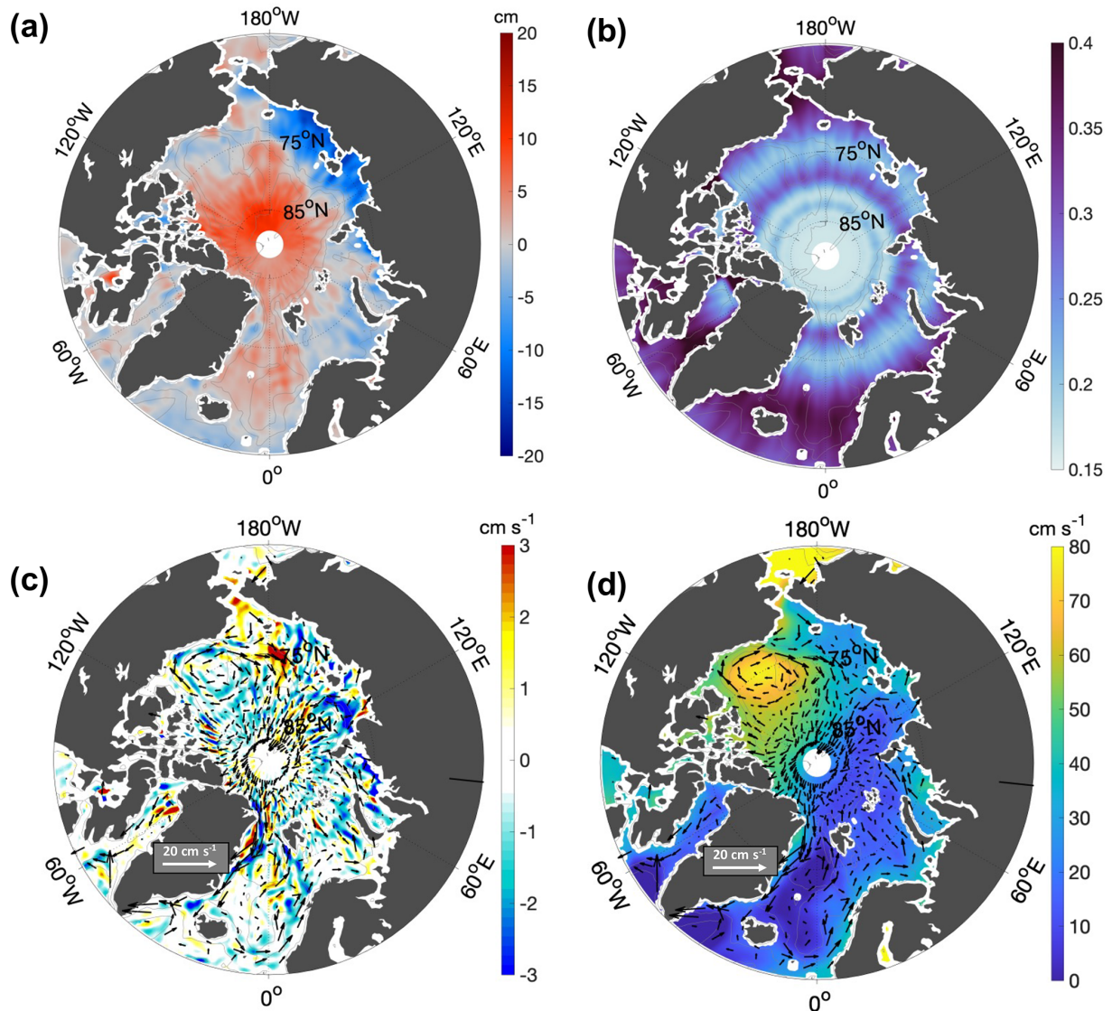
Figure 6. Example of monthly gridded fields included in the final data product for the month of July 2015. (a) The \eta' field above the 2011–2020 background field. (b) Relative error field on the interpolated \eta' , given as a fraction of the variance of the background field. (c) (u_g, v_g) field. Arrows in panel (c) represent the absolute (u_g, v_g) field for the month of July 2015, whereas color highlights the anomaly of the monthly geostrophic speed ( V_g = \sqrt{u_g^2 + v_g^2} ) with respect to the mean geostrophic speed over the period 2011–2020. (d) Dynamic ocean topography ( \eta , background color) and the associated geostrophic velocity field (as in panel (c) ). Bathymetry contours are drawn at 100, 1000 and 2500 m depths.
