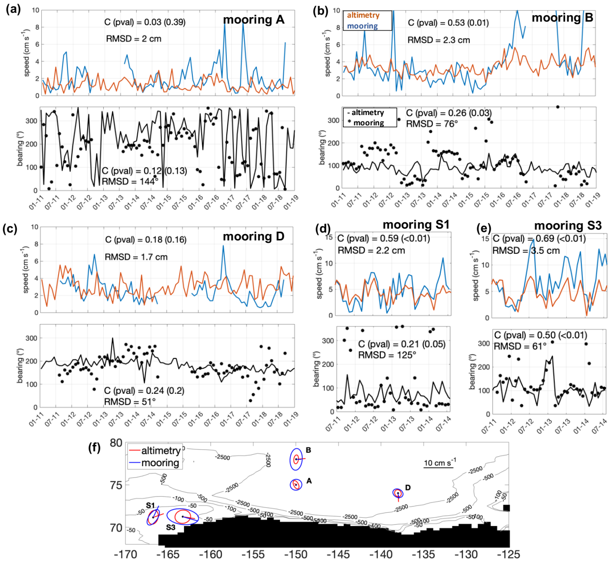
Figure 13. The altimetry-derived currents speed and bearing are shown against the in-situ measured ones at moorings A (panel a), B (panel b) and D (panel c) in the Beaufort Sea, and moorings S1 (panel d) and S3 (panel e) in the Chukchi Sea (see Fig. 1). (f) Mean currents and variance ellipses at each location.
