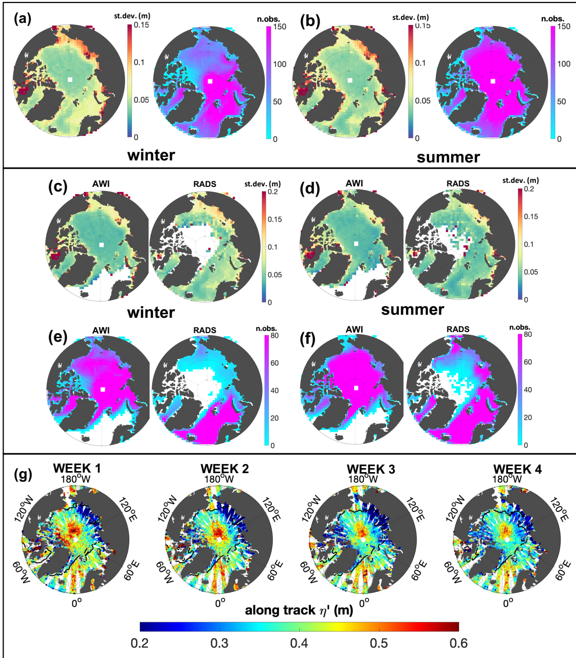
Figure 3. Average monthly statistics of the along-track \eta' dataset over the ice-covered and ice-free Arctic Ocean, in the period 2011-2020 (per 100 km 2 ). Standard deviation (panels a-left, b-left, c, d) and number of observations (panels a-right, b-right, e, f) for the merged dataset (a,b), and separately the AWI and RADS datasets (c,d,e,f) are shown for the winter (October to April) and summer (May to September) seasons. (g) Example of weekly along-track data in the month of July 2015; the black solid line indicates the 15% sea ice concentration as derived from the OSI SAF ice concentration products. Note the different color scales of panels a and b with respect to panels c-d-e-f.
