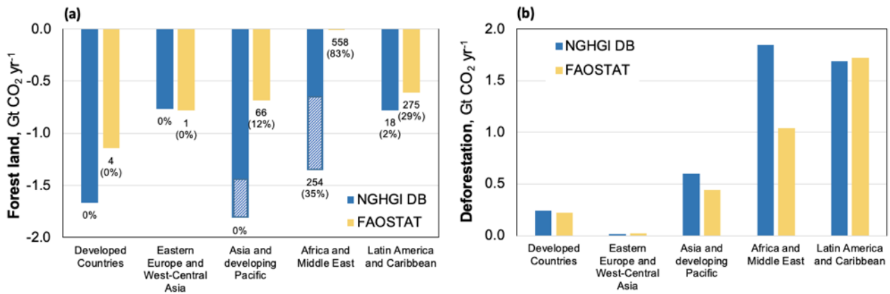
1145 Figure 6. CO 2 fluxes (average 2000-2020) in the five macro-regions from our NGHGI DB and FAOSTAT, for Forest land (a) and Deforestation (b, net deforestation in FAOSTAT). The numbers next to each column in panel a indicate the areas (in Mha, and % relative to the respective regional forest area) where no or zero carbon flux is estimated for FL or for FL-FL. In panel a, the dashed blue areas indicate the carbon fluxes that we consider implausible in the NGHGI DB (see Methods).
