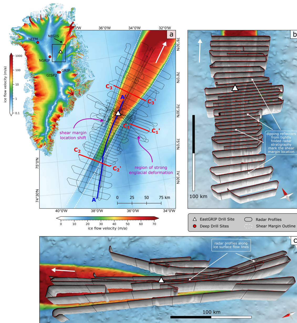
Figure 1. Location of the EGRPI-NOR-2018 survey area in Northeast Greenland with the MEaSUREs ice surface velocity from Joughin et al. (2017) in the background. (a) The radar survey lines are centred at the EastGRIP drill site (white triangle) and extend up to 150 km upstream and downstream of the NEGIS. The locations of one along-flow radar section (Figure 2; blue) and three cross-flow radar sections (Figure 3; red) are shown in panel (a). The ice flow direction of the ice stream is indicated with a white arrow. 3D images of the cross-flow profiles and along-flow profiles are shown in (b) and (c), respectively. The radar sections are shown with a vertical exaggeration factor of z = 10 . The ice surface velocity (Joughin et al., 2017) is shown on a logarithmic scale ( \log_{10} ) for entire Greenland (upper left image) and on a linear scale for panels (a), (b) and (c). For panel (b) and (c) the ice surface velocity is projected on top of the bed topography model from Franke et al. (2020). The projection for all maps is: WGS 84 / NSIDC Sea Ice Polar Stereographic North (EPSG:3413).
