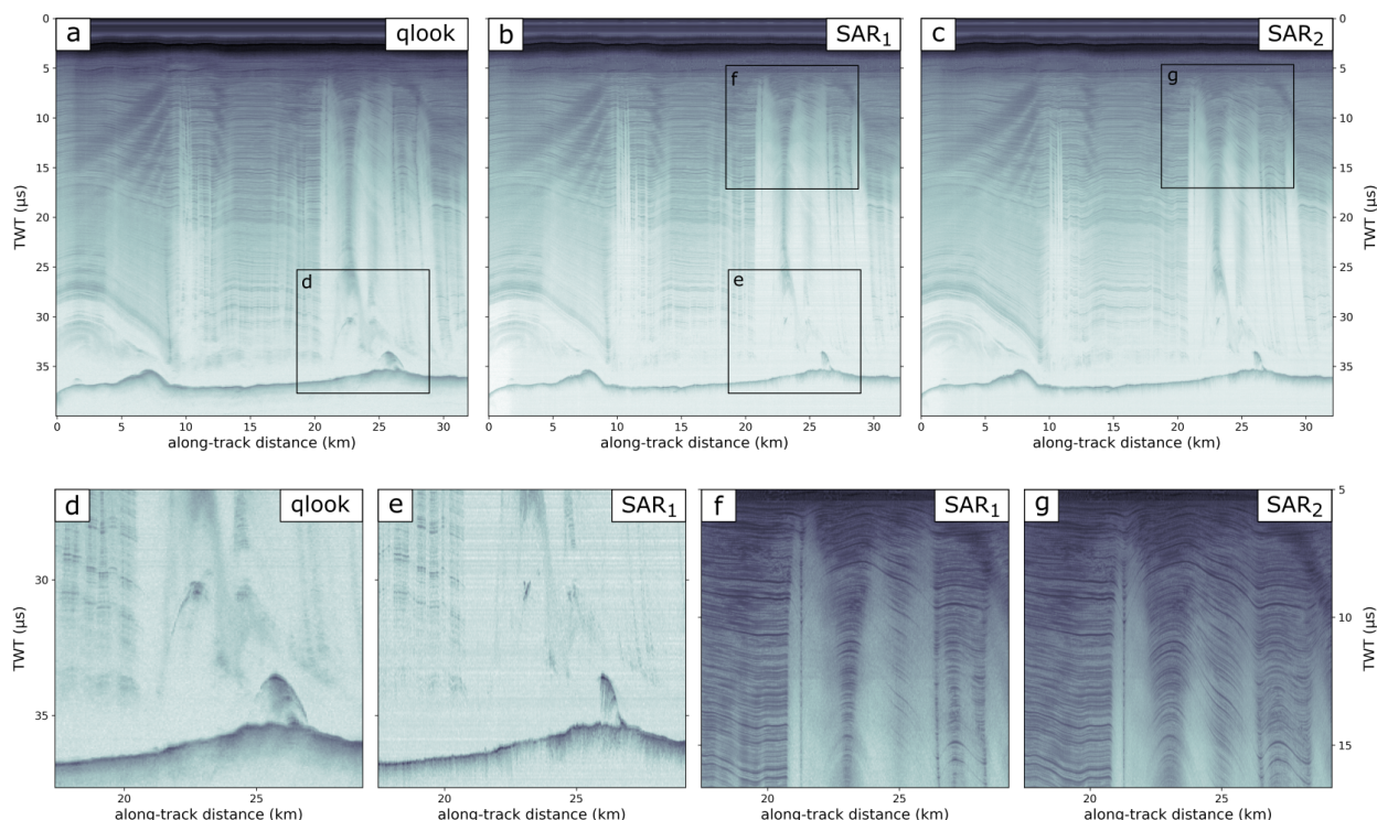
Figure 4. Radargrams of a flow-perpendicular radar profile showing the three different data products: (a) quick-look (qlook) processed, (b) SAR focused ( SAR_1 ) and (c) SAR focused with a larger aperture ( SAR_2 ). The main difference between qlook and SAR_1 is the focusing of signals via fk migration (panel d and e). In contrast do the default SAR focusing (panel f) a larger aperture enables a better resolution of steeply inclined internal layers (panel g).
