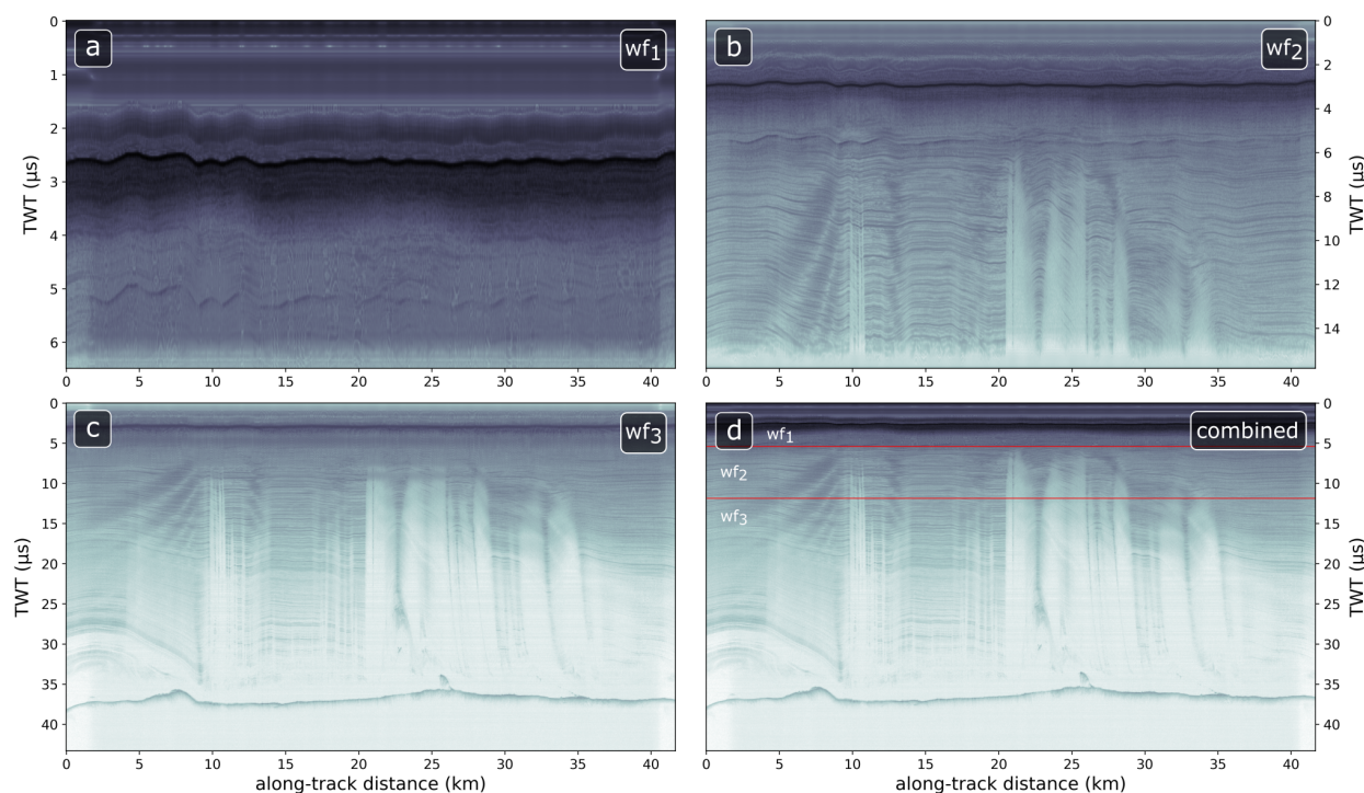
Figure 5. Radargrams of the frame 20180517_01_008 subdivided into (a) waveform 1, (b) waveform 2, (c) waveform 3 and (d) the radargram composed of all three waveforms in combination. The locations, where the different waveforms are concatenated, are indicated with red lines in (d). Waveform 1 and 2 are plotted at full range. Note the different resolution of the near-surface stratigraphy in waveforms 1 to 3.
