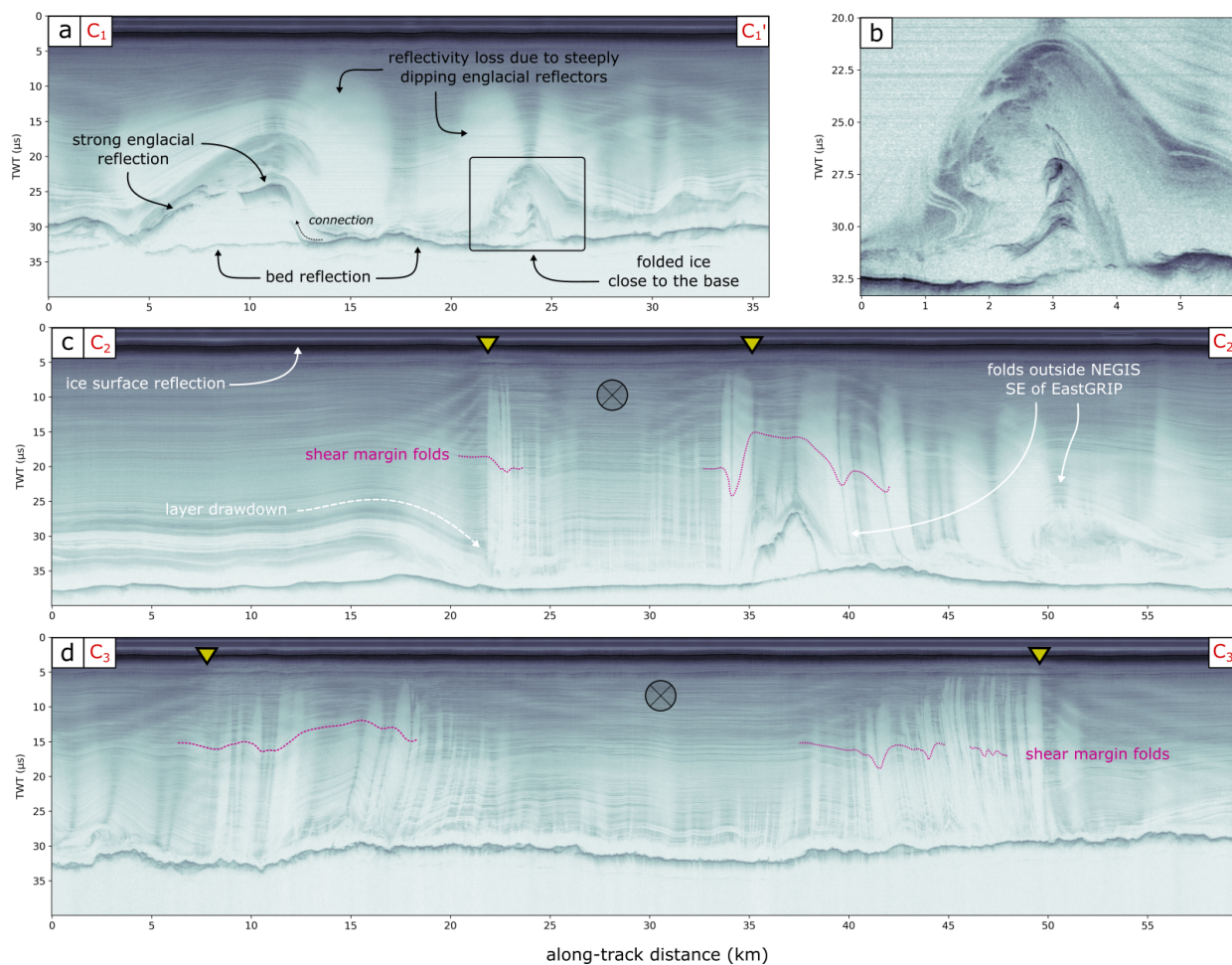
Figure 3. Radar profiles C_{1,2,3} (frames 20180508_06_003, 20180511_01_007 and 20180514_01_011-012, respectively). The corresponding locations are shown in Figure 1a. Panel (a) shows a profile located outside of the NEGIS, SE of EastGRIP. A close up of an anticline and other patterns of deformation are shown in panel (b), resembling the skeleton of a dead penguin. A slice through the ice stream in the upstream region is shown in panel (c) and a radar section further downstream in (d). The position of the shear margins (the maximum in the surface velocity gradient) are indicated with a yellow triangle and the folds in the shear margin areas with purple lines. The ice flow direction is out of the page.
