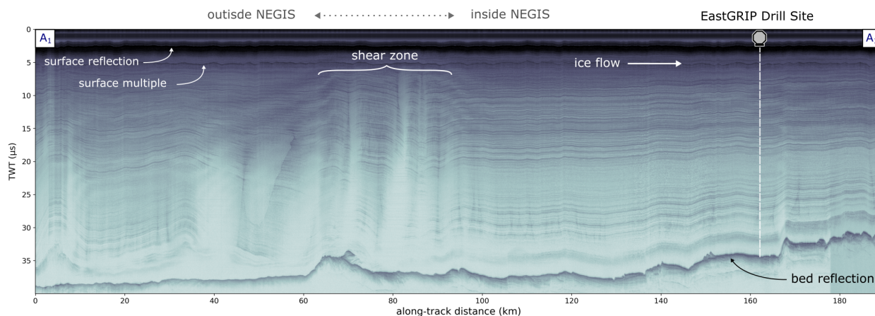
Figure 2. Flow-parallel radar profile A composed of three frames: 20180512_01_001-004. The location is indicated in Figure 1a and covers the area outside of the ice stream, the shear zone and the ice stream's trunk. The position of the EastGRIP drill site is labeled and indicated with a white dashed vertical line.
