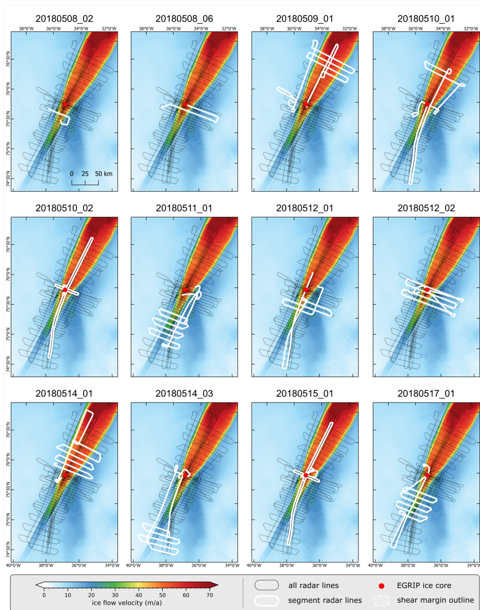
Figure A1. Radar profiles locations of the 12 segments shown in Table A1 of the EGRIP-NOR-2018 data set. The respective segments are highlighted with a white line and the radar profiles of the complete survey with a finer black line. The background map represents ice surface velocity from Joughin et al. (2017). The shear margin is indicated with a white dashed outline and the location of EastGRIP with a red dot.
