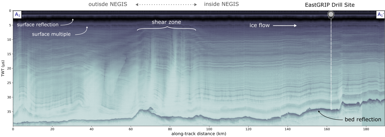
Figure 2. Flow-parallel radar profile A composed of three frames: 20180512_01_001-004. The location is indicated in Figure 1a and covers the area outside of the ice stream, the shear zone and the ice stream’s trunk. The position of the EastGRIP drill site is labeled and indicated with a white dashed vertical line.
