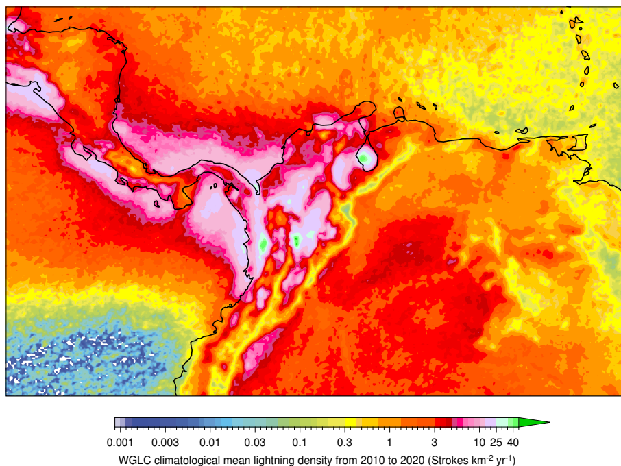
Figure 5. High resolution (5 arc-minute) climatological mean annual lightning stroke density over northwestern South America and Central America.
