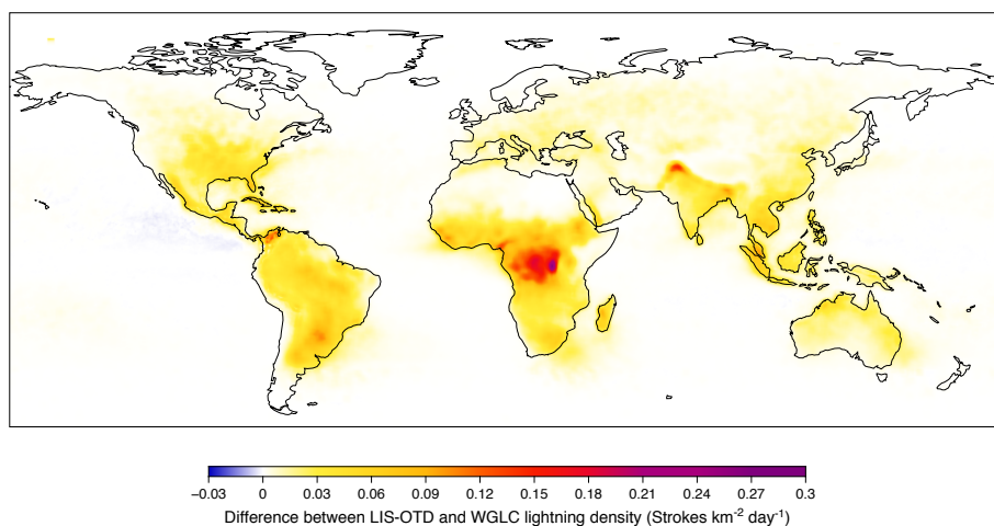
Figure 15. Difference between climatological annual mean lightning density in LIS/OTD (1995-2014) and WGLC (2010-2019).
