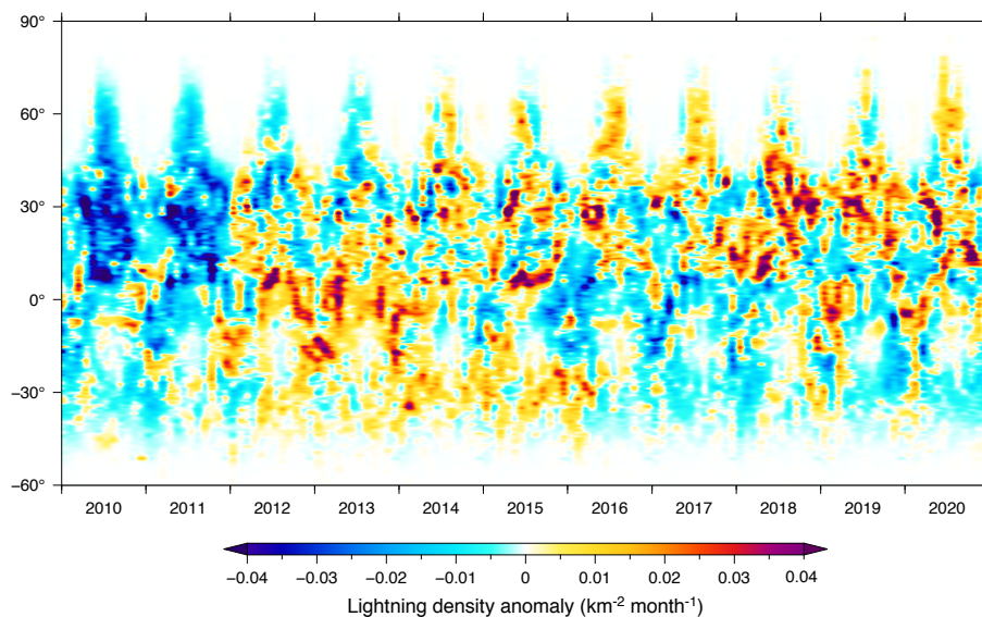
Figure 8. Zonal mean lightning stroke density anomalies (monthly value relative to the climatological monthly mean from 2010-2020).
