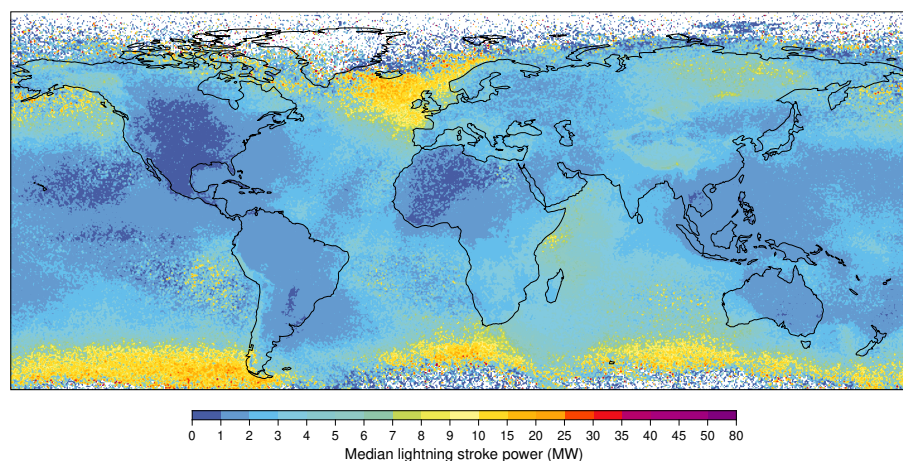
Figure 9. Climatological annual mean of the median lightning power-per-stroke.
