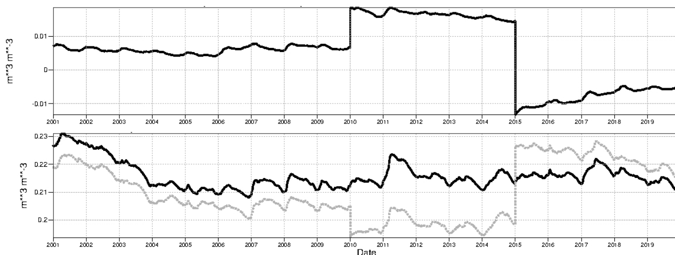
Figure 3. Top: Mean differences between ERA5-Land and ERA5 soil moisture time series for the fourth soil layer of the CHTESSEL land surface model (100-289 cm), averaged for the latitudes 60 S - 20 S. The temporal resolution is 12 hours. Bottom: Raw time series of ERA5 (dashed light grey curve) and ERA5-Land (dark curve).
