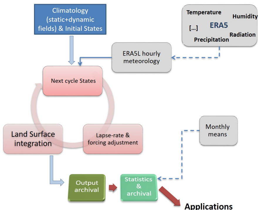
Figure 2. Diagram of the algorithm used in the production of ERA5-Land. The land surface model is integrated in 24 h cycles, using short-forecast meteorological forcing fields from ERA5.
