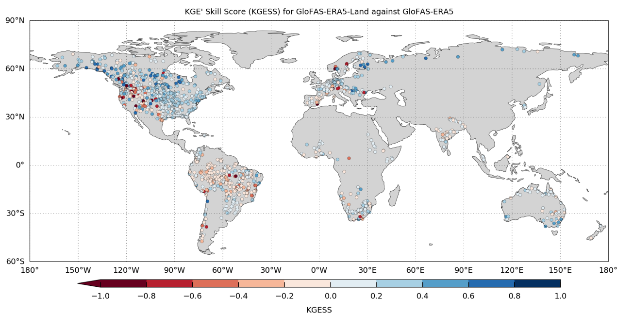
Figure 14. Modified Kling-Gupta Efficiency Skill Score ( KGE SS ) for GloFAS-ERA5-Land river discharge reanalysis against the GloFAS-ERA5 benchmark across 1285 observation stations. Optimum value of KGE SS is 1. Blue (red) dots show catchments with positive (negative) skill.
