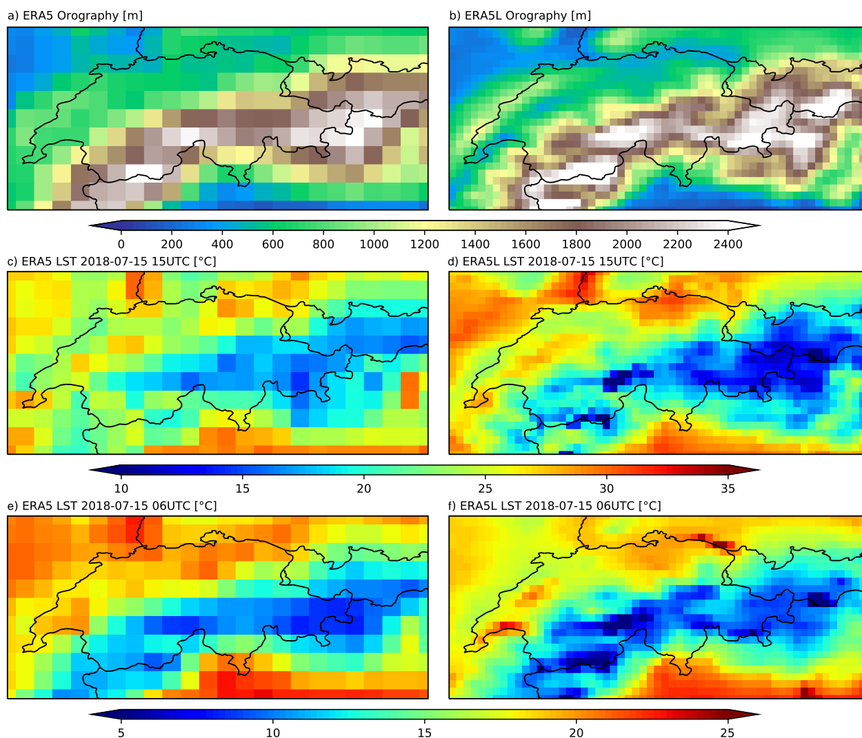
Figure 4. ERA5 (left column) and ERA5-Land (right column) orography (top row) of the Alpine region around Switzerland. The middle and bottom rows show the land surface temperature on 15 July 2018 at 15UTC (middle) and 06UTC (bottom), respectively.
