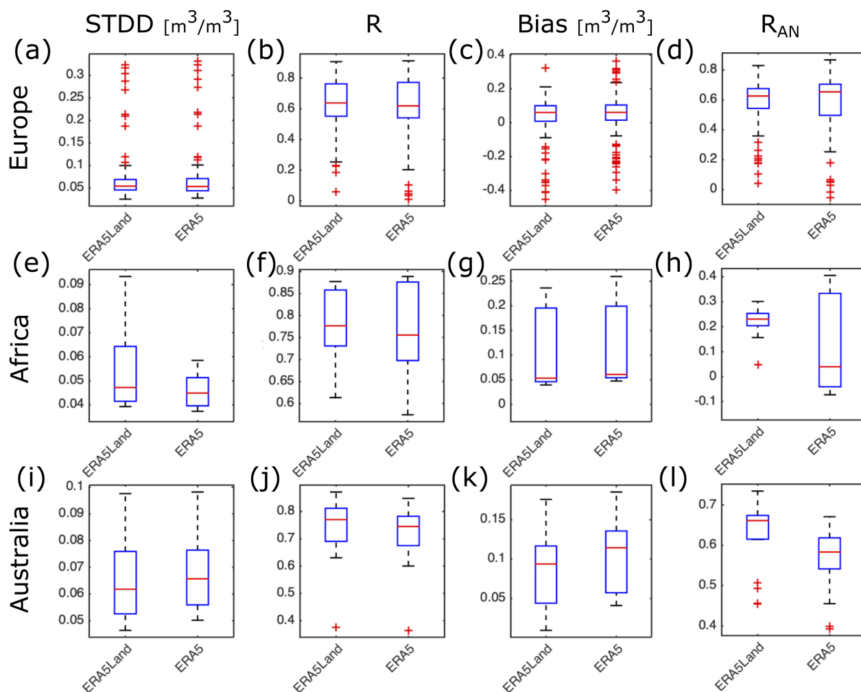
Figure 6. Box plots showing the evaluation of ERA5-Land and ERA5 top layer soil moisture against in situ measurements at 5 cm for sites in Europe (top row), Africa (middle row) and Australia (lower row). The first column of panels (left) shows the standard deviation of the difference (STDD), the second column is the Pearson correlation coefficient (R), the third column is the bias and the fourth column is the Pearson correlation of the anomalies time series ( R_{AN} ). On each box, the central mark indicates the median, and the bottom and top edges of the box indicate the 25th ( q_{25} ) and 75th ( q_{75} ) percentiles, respectively. The whiskers extend to the most extreme data points not considered outliers.
