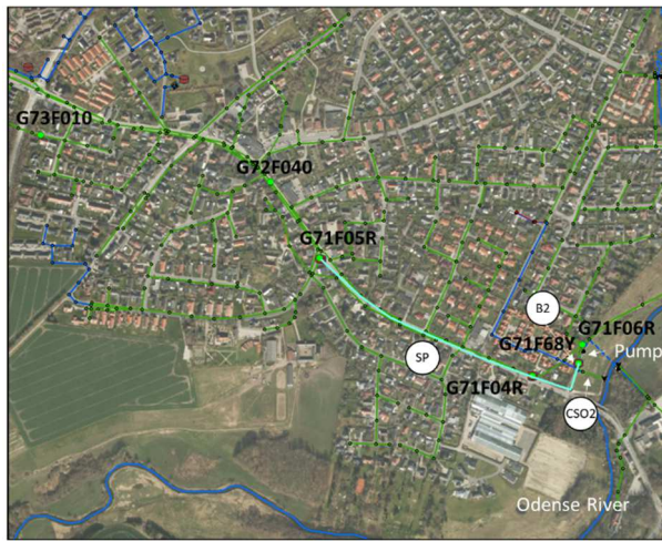
180 Figure 6: Location of the sensors in Bellinge. The storage-pipe (SP) and basin B2 are highlighted (cyan) and the location of CSO 2 is indicated. Background maps provided by DADSE (2020).
