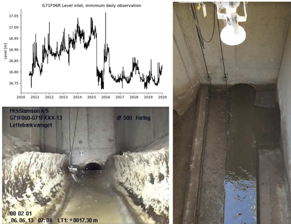
260 Figure 8: Anomaly in level data and possible causes. The minimum daily water level in G71F06R (upper left corner) along with a CCTV image (lower left corner) of G71F06R from June 2013 and a photo of the same location from 2019 (right) showing also the location of the level sensor (radar). Videos and additional photos can be found in the data set (Pedersen et al., 2021a). A large anomaly in data occurs May 11 th , 2015, which is possibly due to retrofitting of the banquettes in the structure at this date. Pictures by (VCS Denmark, 2020)
