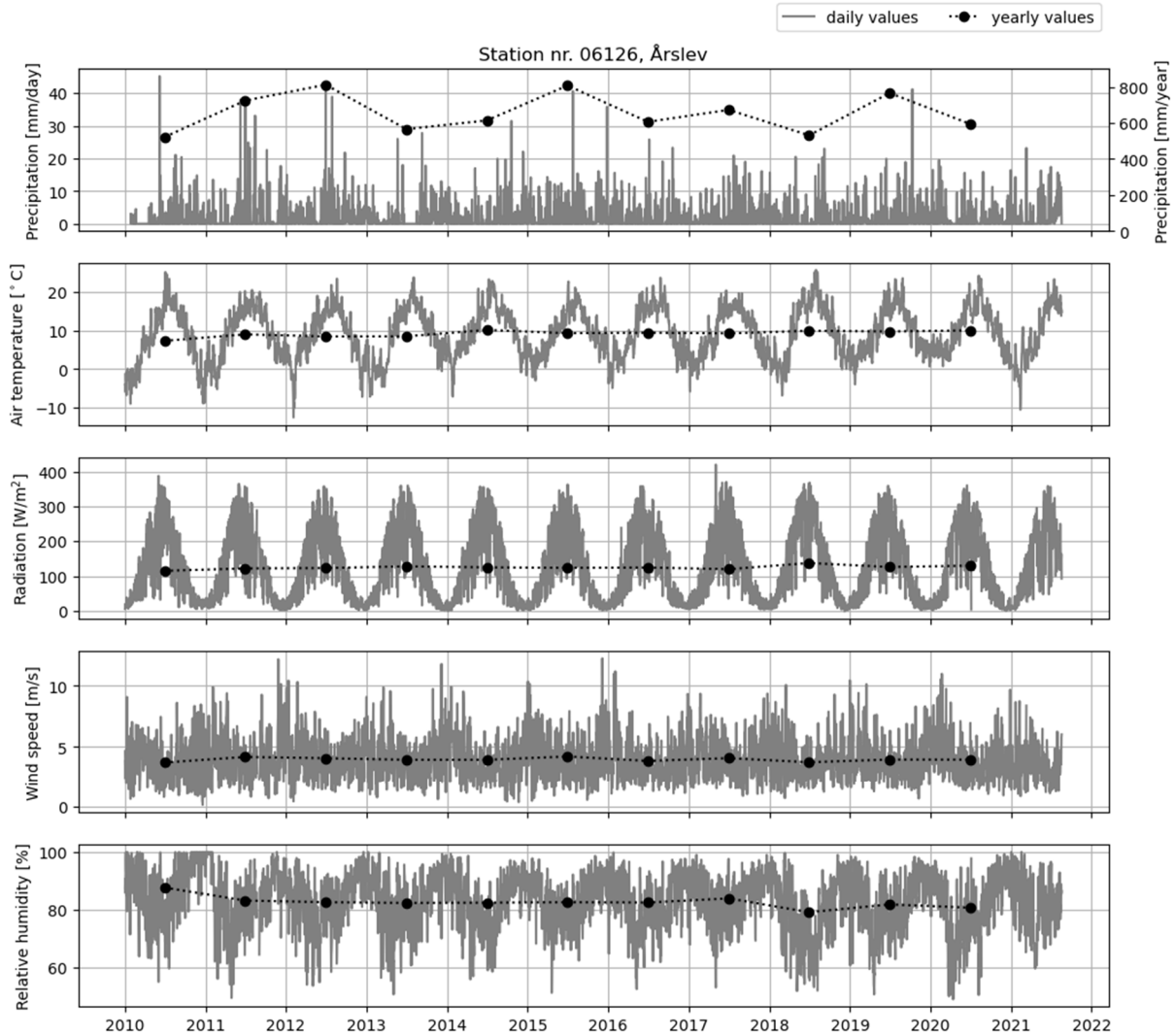
135 Figure 2: Meteorological data from a weather station in Årslev app. 10 km east of the case area. Bins on the horizontal axis refer to the beginning of each year. Precipitation data is extracted in 10 min resolution and summed to daily and yearly values. Air temperature, radiation, wind speed and relative humidity are given as daily and yearly means. Based on open hydrological data from (DMI, 2020) where more parameters can be extracted.
