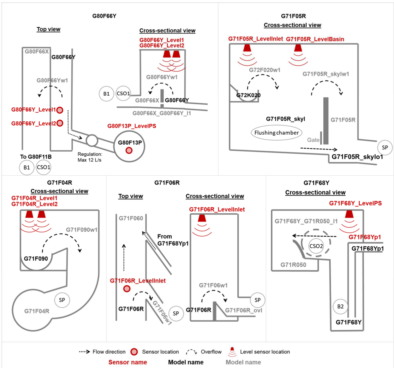
155 Figure 4: Illustration of the most complex hydraulic structures with relevant names referring to nodes in the models (black text, see also Figure 1 and Figure 3) and sensors (red text, see further details in Section 3). The grey texts are names of additional model locations.
