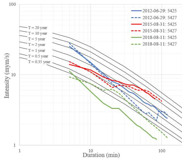
410 Figure 10: Intensity-duration-frequency (IDF) characteristics for the three selected rain events (2012, 2015 and 2018) measured at two different rain gauges (gauge 5425 and 5427), plotted on top of national regional IDF curves for Odense (Gregersen et al. (2014)). T indicates return periods, corresponding to the reciprocal of the frequency.
