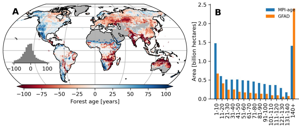
69 Figure S4 Difference between the forest age estimates derived from the MPI-BGC forest age product adjusted with 70 MODIS fire and the GFAD product. Differences were computed using a weighted from fraction of the decadal age 71 classes within each 0.5 degree grid cell resolution
