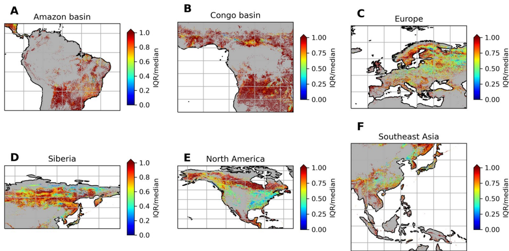
58 Figure S3 Interquartile range divided by the median of the forest age estimates for the classified non-old growth 59 forests.
