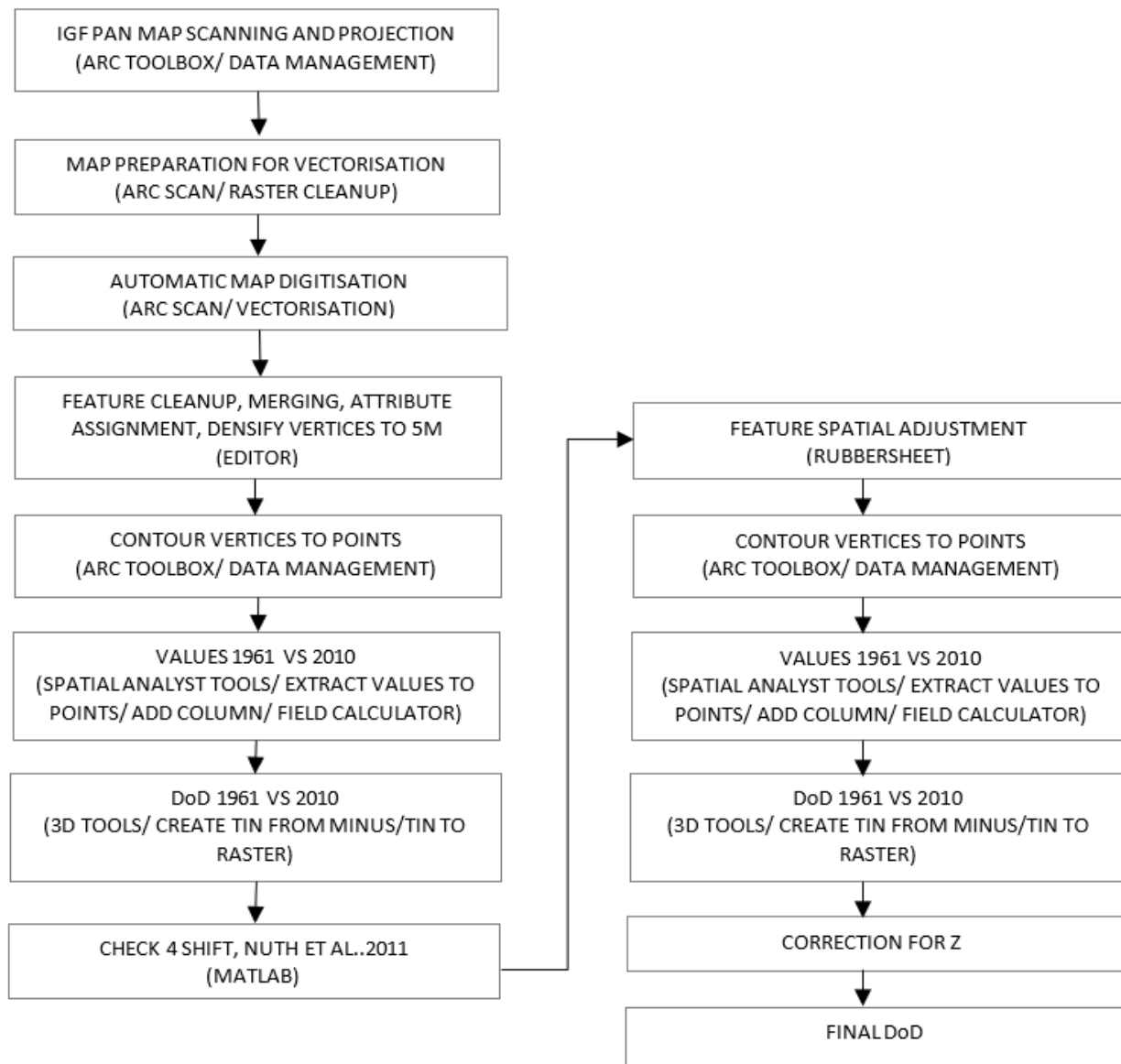
Figure 8. Work flow for processing IGF PAN map sheets.
