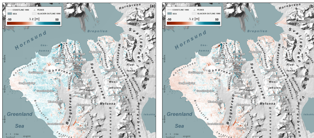
Figure 7. Elevation differences between the 1990 DEM and the 2010 DEM generated by NPI (2014) (a) before applying correction (b) after correcting for shift vector as proposed by Nuth and Käab (2011).
