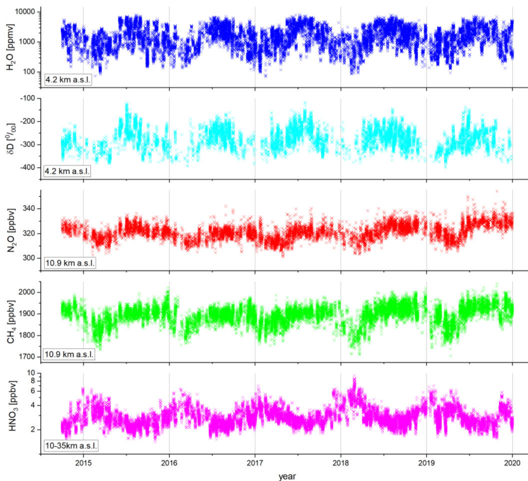
Figure 14. Time series of MUSICA IASI trace gas products at selected altitudes above Karlsruhe (48–49°N; 8–9°E): 4.2 km a.s.l. for H 2 O and \delta D , 10.9 km a.s.l. for N 2 O and CH 4 , and 10–35 km a.s.l. for HNO 3 . Data have been filtered according to the setting given in Table 4.
