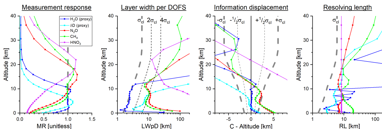
Figure 11. Profiles with averaging kernel metrics for the 30. Aug. 2008 example observation over Lindenberg used for Fig. 9. The thick grey dashed lines indicate for orientation the 100% value (for the panel showing the measurement response) and the a priori assumed vertical correlation length (for the panels showing the layer width per DOFS, information displacement, and resolving length).
