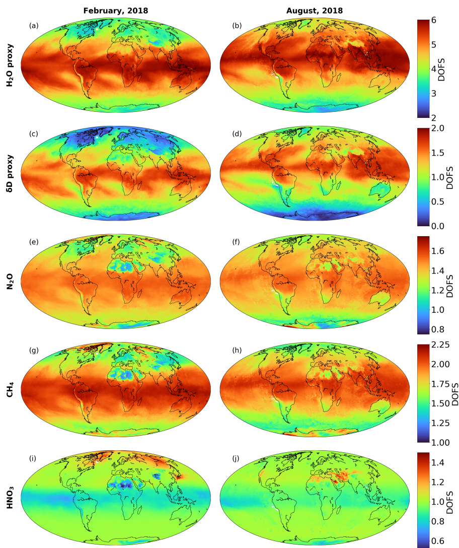
Figure 10. Monthly averaged maps of degree of freedom for signal (DOFS) values for February and August 2018 for all targeted atmospheric species: H 2 O, δD, N 2 O, CH 4 , and HNO 3 .
