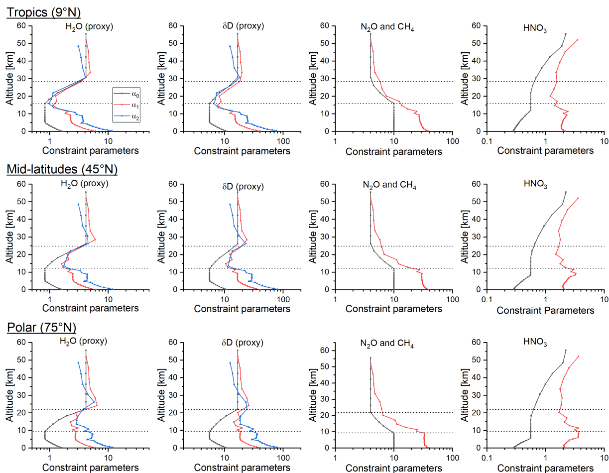
Figure 6. Vertical profiles of the constraint parameter \alpha_0 , \alpha_1 , and \alpha_2 for the retrieval of all targeted atmospheric species (H 2 O, δD, N 2 O, CH 4 , and HNO 3 ). The parameters are latitudinal and time dependent. Shown are examples for 8. July 2018 for the tropics (9°N), mid-latitudes (45°), and polar regions (75°). The area between the dotted lines indicates the transition between troposphere and stratosphere.
