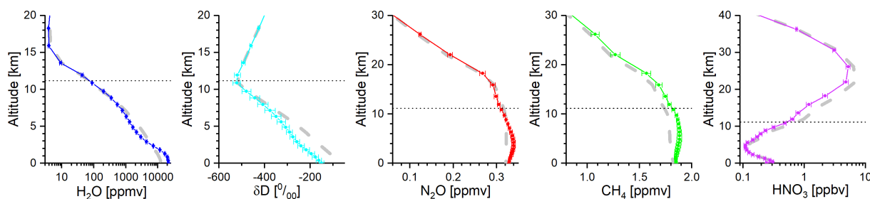
Figure 7. Example of vertical profiles of the targeted atmospheric trace gas products ( \text{H}_2\text{O} , \delta\text{D} , \text{N}_2\text{O} , \text{CH}_4 , and \text{HNO}_3 ): thick grey dashed lines represent the a priori assumption and the coloured line with symbols and error bars are the retrieved values and the root-square-sum of the fit noise error and the estimated temperature error. The data are for the 30. Aug. 2008 example observation over Lindenberg ( 53^\circ\text{N} ) used for Fig. 4.
