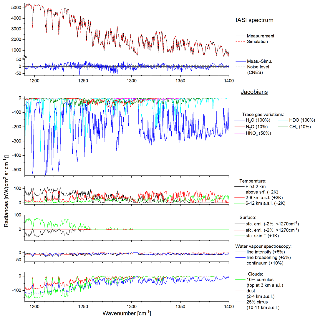
Figure 4. Example for a spectrum, residual (difference between measured and simulated spectrum) and different spectral responses (Jacobians) for an observation over the mid-latitudinal site of Lindenberg on 30. Aug. 2008 (satellite nadir angle: 43.7^\circ ; surface skin temperature: 292.3 K; precipitable water vapour: 31.8 mm).
