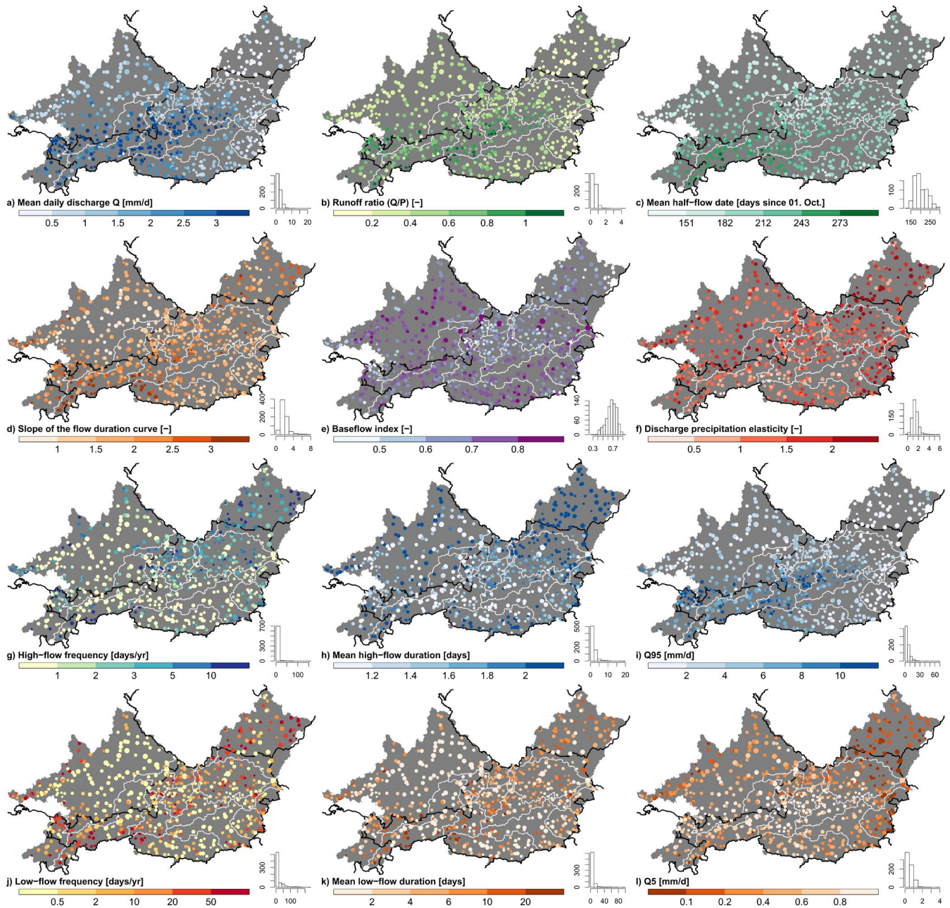
Fig. 7: Spatial distribution of hydrological signatures. Only gauges are plotted, which cover the period 1 October 1989 to 30 September 2009. The histograms indicate the number of gauges (out of 717) in each category. The size of the circles is proportional to the catchment area. © EuroGeographics for the administrative boundaries.
