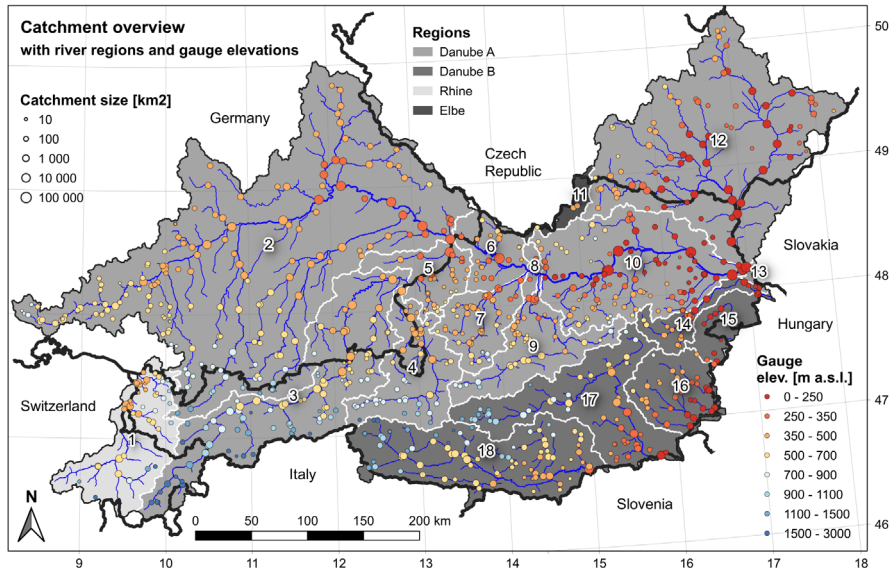
Fig. 1: Overview of the area covered in LamaH (grey tones), and the runoff gauges with gauge elevation (circle color) and catchment area (circle size). LamaH is divided into different river regions, which are bordered by the white lines. The black numbers are abbreviations for the individual regions, which are indicated in Table B1. The national borders are shown as thick black lines. Source of stream network: HydroATLAS (Linke et al., 2019). © EuroGeographics for the administrative boundaries.
