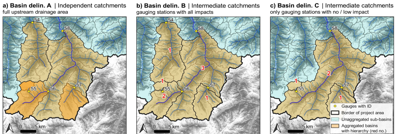
140 Fig. 2: Types of basin delineations in LamaH shown with an example. Plot a) Basin delineation A (similar to the well-known CAMELS datasets): The aggregation area corresponds to the topographic catchment area of a gauge. In plot a), the aggregation area of gauges 56 and 57 overlaps with that of gauge 58, and the aggregation area of gauge 55 overlaps with that of gauges 56 and 58 (indicated by the different color tones). Plot b) Basin delineation B: The aggregation areas in this method considers the difference
