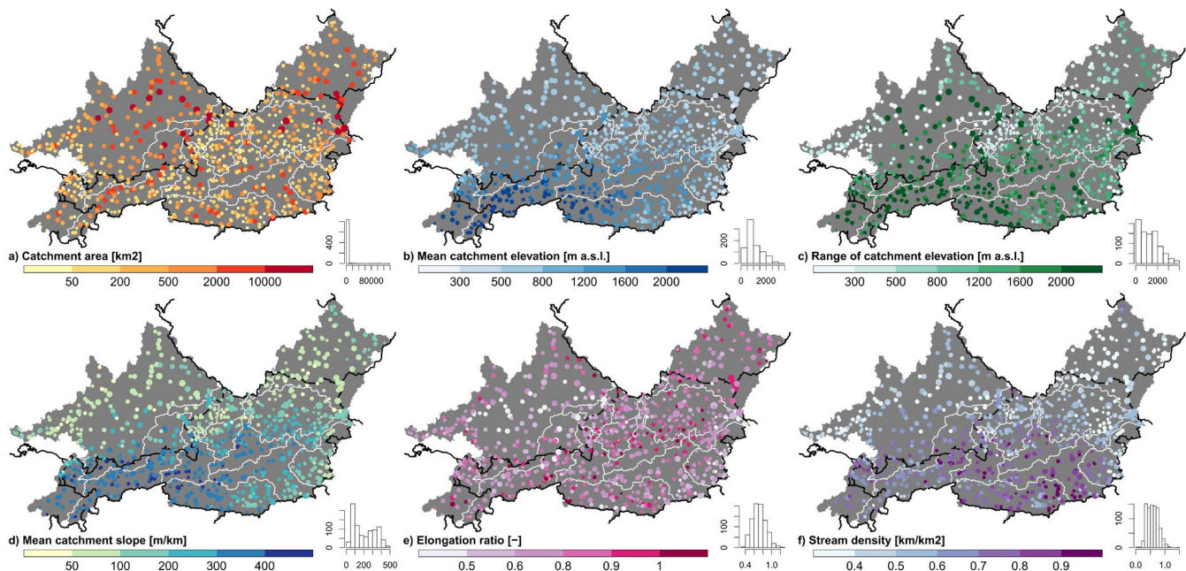
315 Fig. 5: Spatial distribution of a selection of topographic attributes representing the characteristics of the entire topographic catchment (basin delineation A, Fig. 2a). The histograms indicate the number of basins (out of 859) in each category. The size of the circles is proportional to the catchment area. © EuroGeographics for the administrative boundaries.
