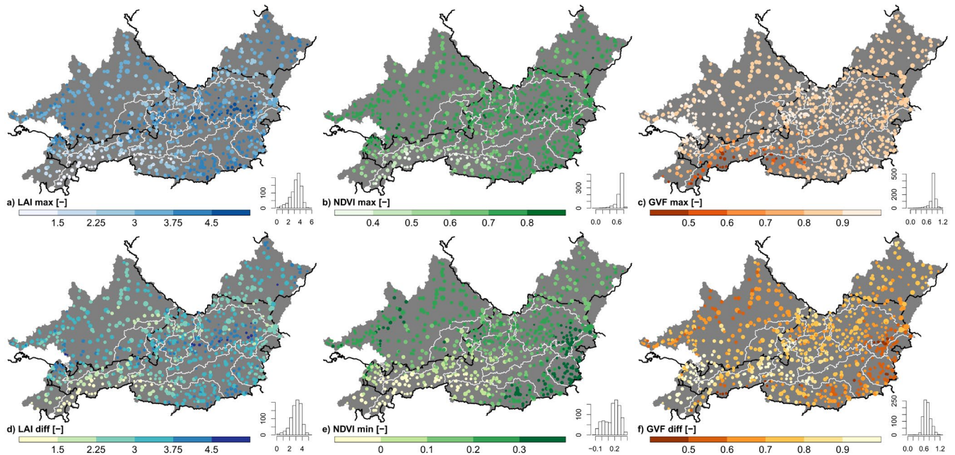
Fig. 9: Spatial distribution of vegetation indices representing the characteristics of the entire topographic catchment (basin delineation A, Fig. 2a). The histograms indicate the number of basins (out of 859) in each category. The size of the circles is proportional to the catchment area. © EuroGeographics for the administrative boundaries.
