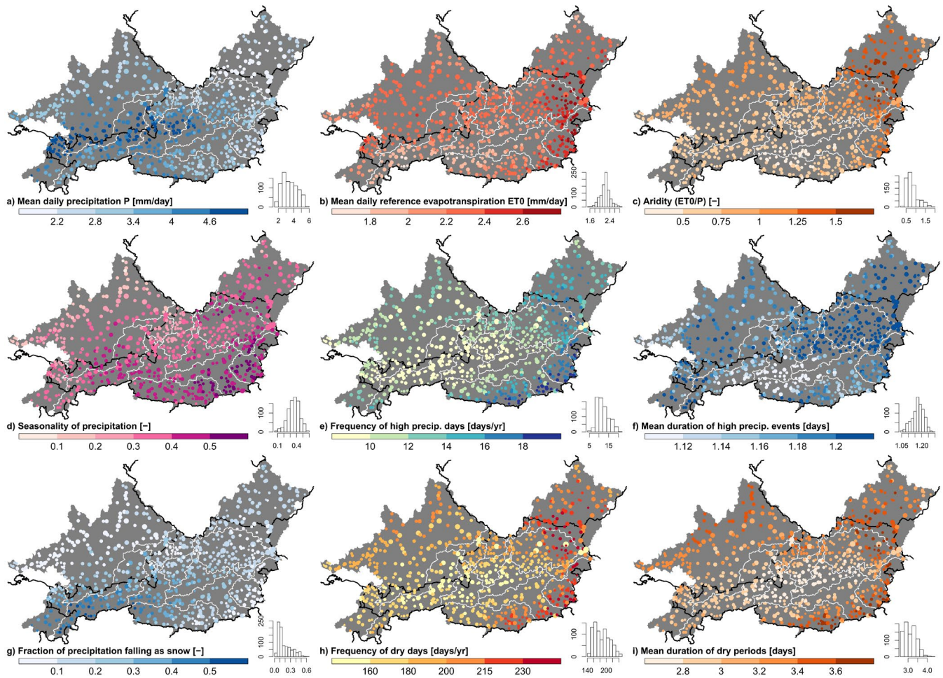
Fig. 6: Spatial distribution of a selection of climate indices representing the characteristics of the entire topographic catchment (basin delineation A, Fig. 2a). The histograms indicate the number of basins (out of 859) in each category. The size of the circles is proportional to the catchment area. © EuroGeographics for the administrative boundaries.
