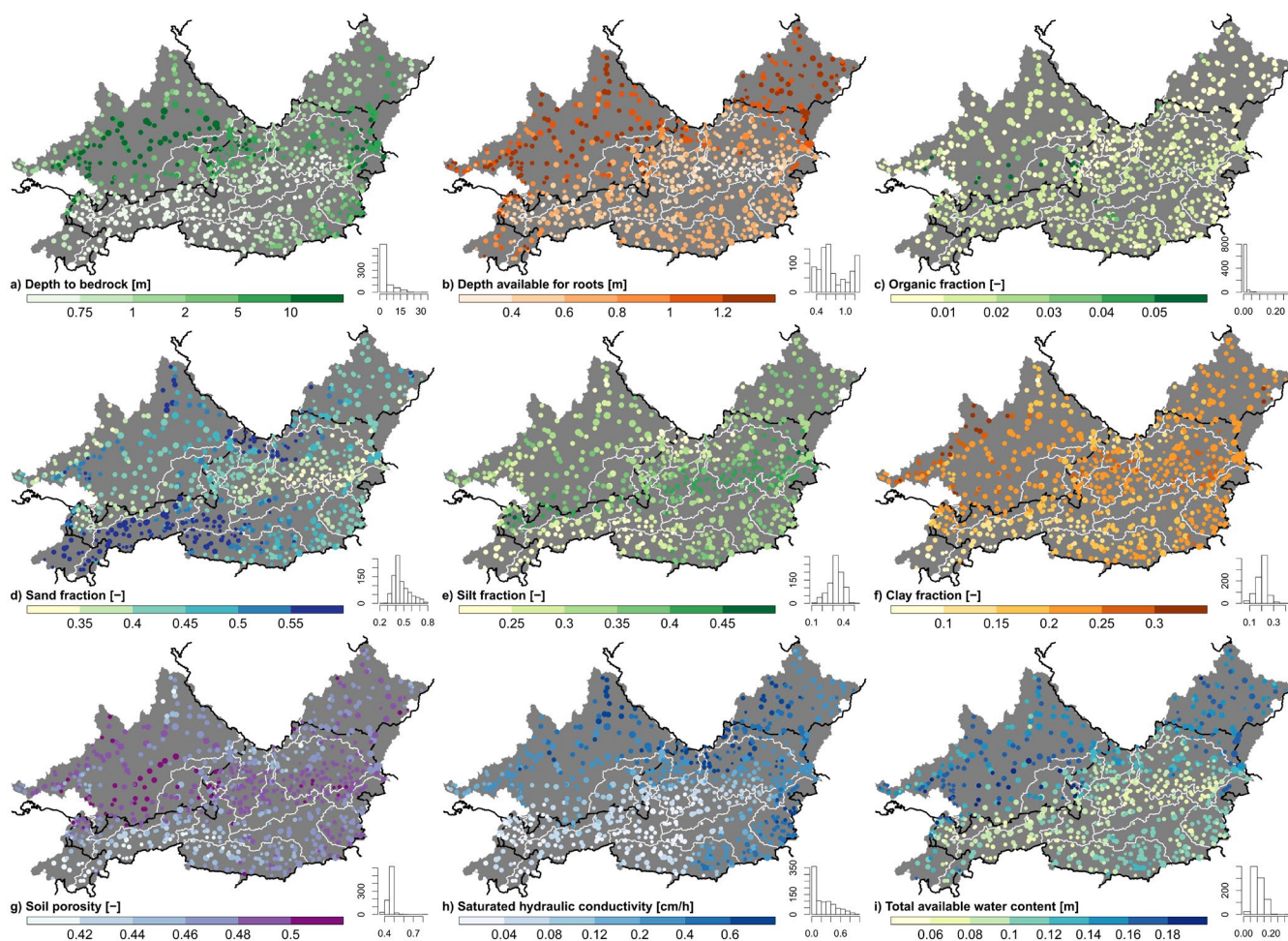
505 Fig. 10: Spatial distribution of soil attributes representing the characteristics of the entire topographic catchment (basin delineation A, Fig. 2a). The histograms indicate the number of basins (out of 859) in each category. The size of the circles is proportional to the catchment area. © EuroGeographics for the administrative boundaries.
