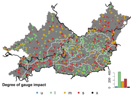
Fig. 12: Degree of (anthropogenic) impact on gauges / catchments. The histogram indicates the number of gauges (out of 882) in each category. The size of the circles is proportional to the catchment area. Classes: u – no influence, l – low influence, m – moderate influence, s – strong influence, x – not considered in basin delineation. © EuroGeographics for the administrative boundaries.
