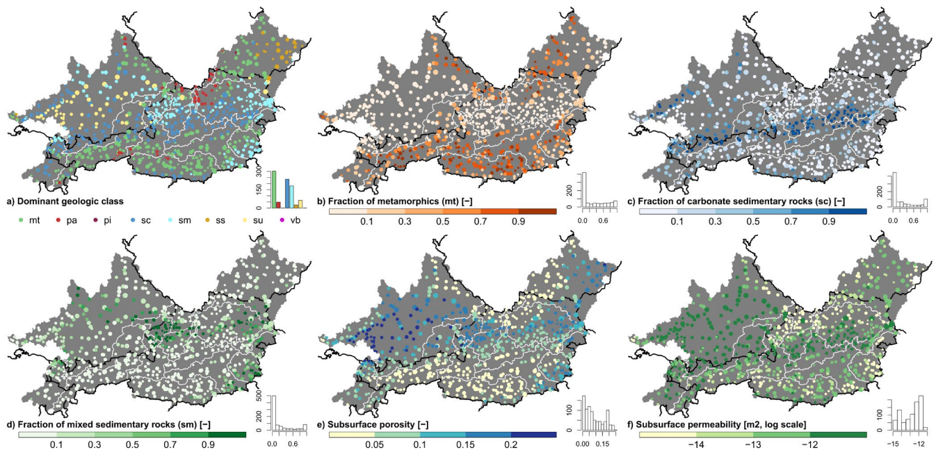
535 Fig. 11: Spatial distribution of geological attributes representing the characteristics of the entire topographic catchment (basin delineation A, Fig. 2a). The histograms indicate the number of basins (out of 859) in each category. The size of the circles is proportional to the catchment area. Classes in plot a): mt – Metamorphites, pa – Acid plutonic rocks, pi – Intermediate plutonic rocks, sc – Carbonate sedimentary rocks, sm – Mixed sedimentary rocks, ss – Siliciclastic sedimentary rocks, su – Unconsolidated sediments, vb – Basic volcanic rocks. © EuroGeographics for the administrative boundaries.
