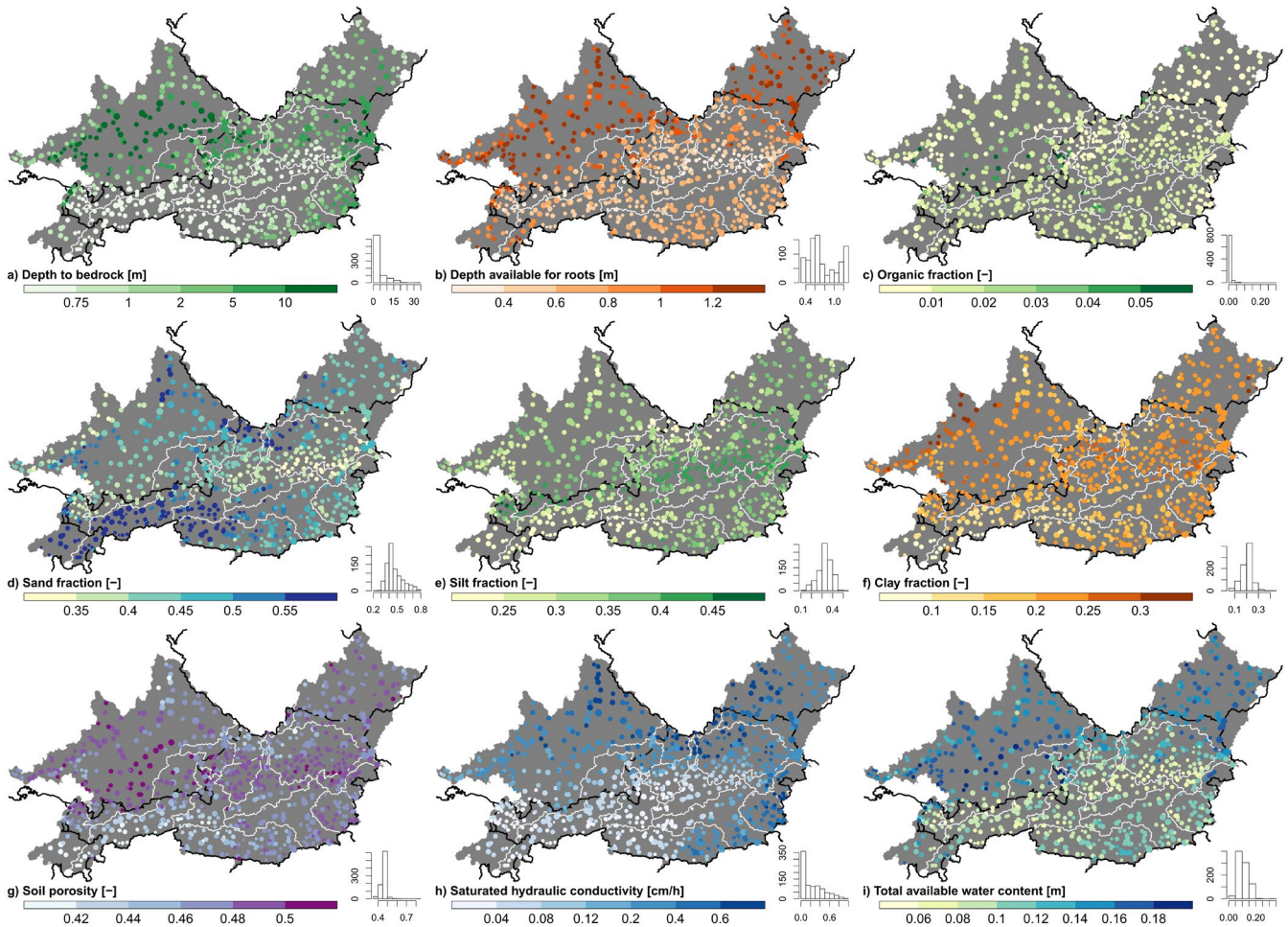
Fig. 10: Spatial distribution of soil attributes representing the characteristics of the entire topographic catchment (basin delineation A, Fig. 2a). The histograms indicate the number of basins (out of 859) in each category. The size of the circles is proportional to the catchment area. © EuroGeographics for the administrative boundaries.
