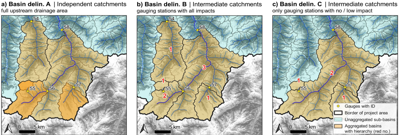
Fig. 2: Types of basin delineations in LamaH shown with an example. Plot a) Basin delineation A (similar to the well-known CAMELS datasets): The aggregation area corresponds to the topographic catchment area of a gauge. In plot a), the aggregation area of gauges 56 and 57 overlaps with that of gauge 58, and the aggregation area of gauge 55 overlaps with that of gauges 56 and 58 (indicated by the different color tones). Plot b) Basin delineation B: The aggregation areas in this method considers the difference
