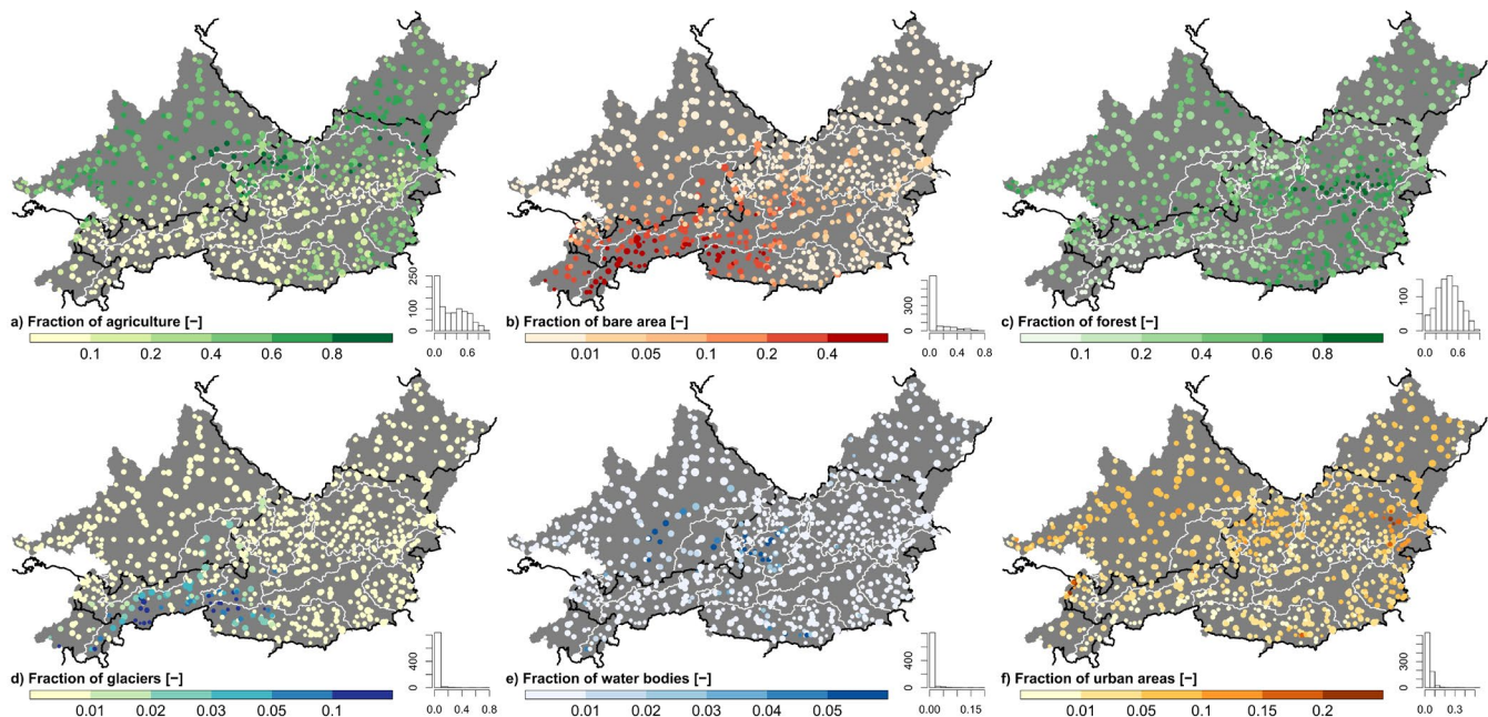
Fig. 8: Spatial distribution of land class fractions representing the characteristics of the entire topographic catchment (basin delineation A, Fig. 2a). The histograms indicate the number of basins (out of 859) in each category. The size of the circles is proportional to the catchment area. © EuroGeographics for the administrative boundaries.
