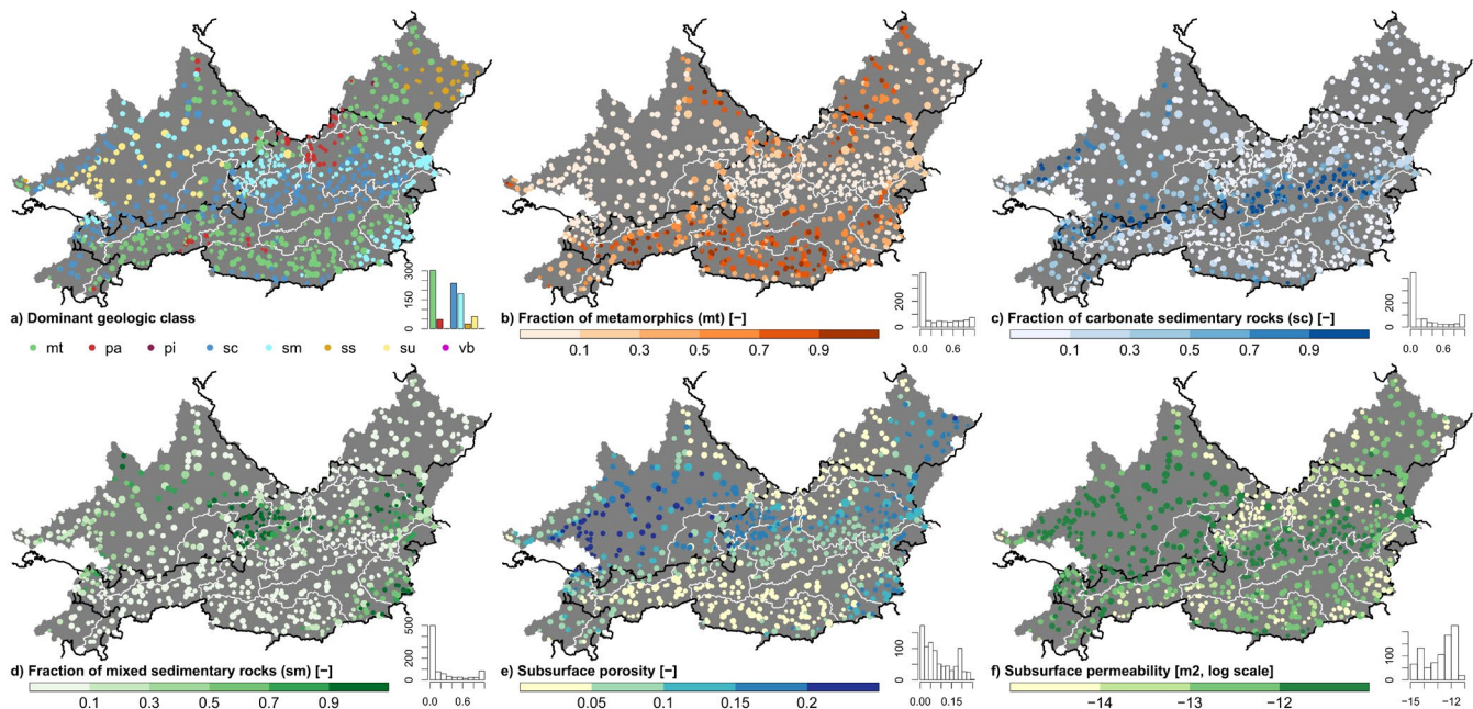
Fig. 11: Spatial distribution of geological attributes representing the characteristics of the entire topographic catchment (basin delineation A, Fig. 2a). The histograms indicate the number of basins (out of 859) in each category. The size of the circles is proportional to the catchment area. Classes in plot a): mt – Metamorphites, pa – Acid plutonic rocks, pi – Intermediate plutonic rocks, sc – Carbonate sedimentary rocks, sm – Mixed sedimentary rocks, ss – Siliciclastic sedimentary rocks, su – Unconsolidated sediments, vb – Basic volcanic rocks. © EuroGeographics for the administrative boundaries.
