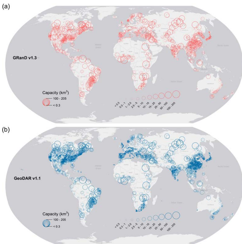
Figure 12. Global distribution of reservoir storage capacities of georeferenced dams. (a) GRanD v1.3 and (b) GeoDAR v1.1. Displayed Shown on the maps are 7,312 out of the 7,320 dams in GRanD v1.3 and 24,347 24,174 out of the 24,978 24,783 dams in GeoDAR v1.1 with documented or estimated reservoir storage capacities.
