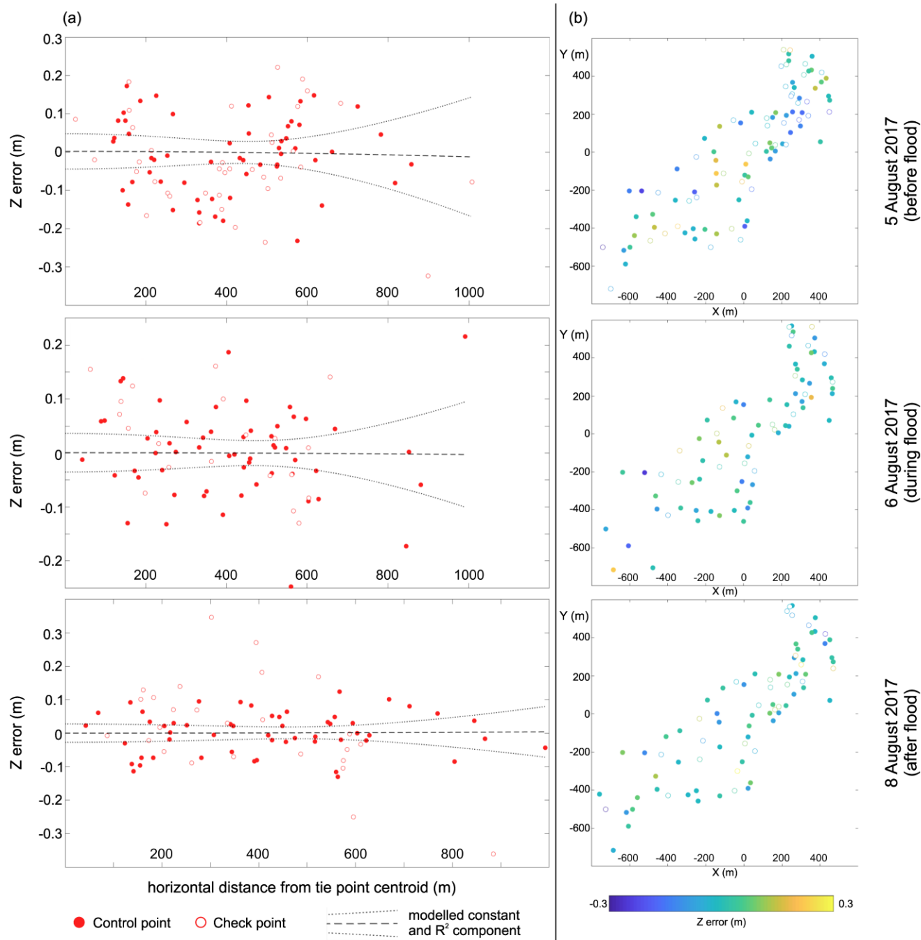
Figure 5: Spatial distribution of errors on control and check points: (a) Z-error against radial distance from the tie point centroid; (b) Z-error by colour in plan view (X, Y are distanced from tie points centroid).
