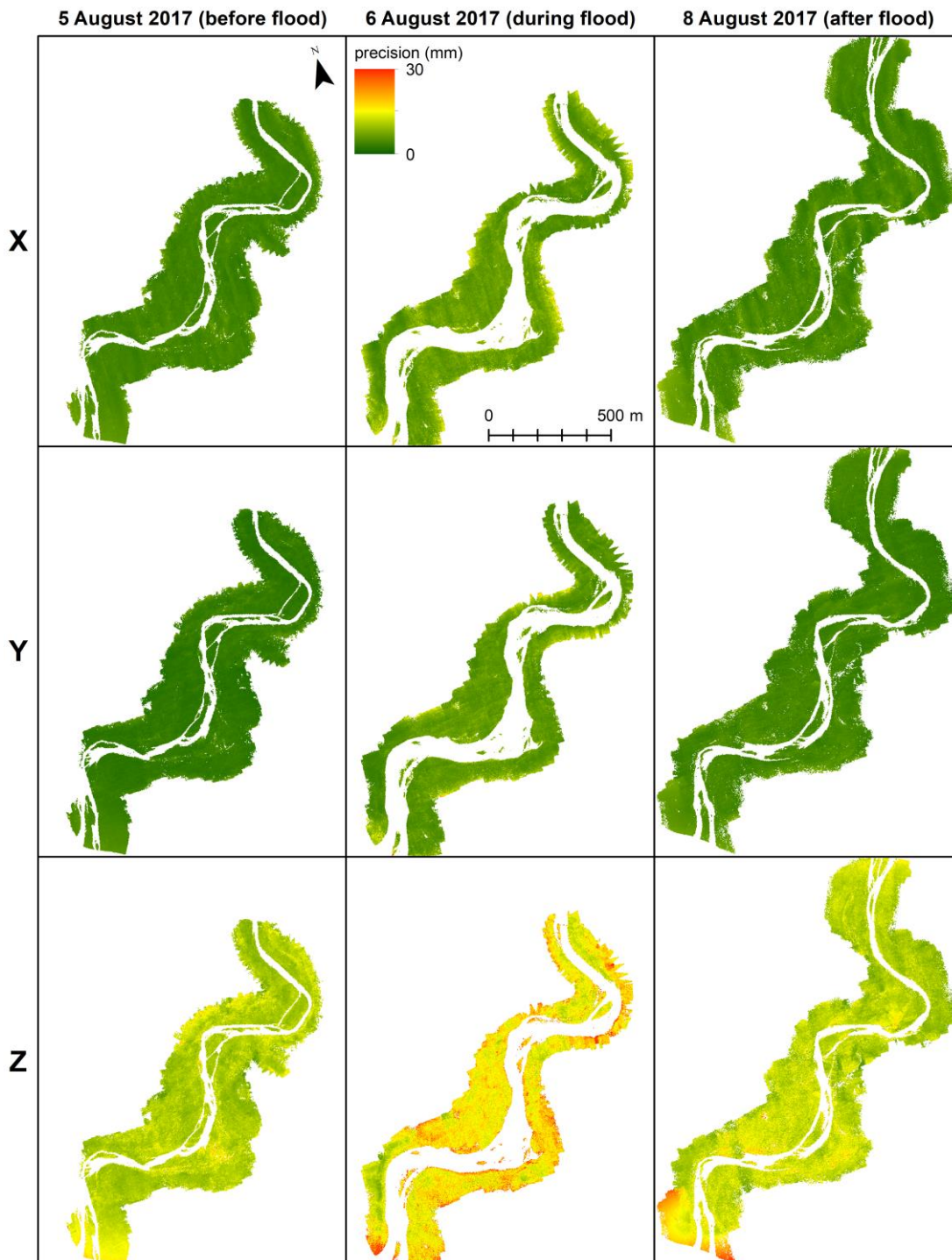
Figure 4: Precision estimates for X, Y, Z coordinates of tie points
