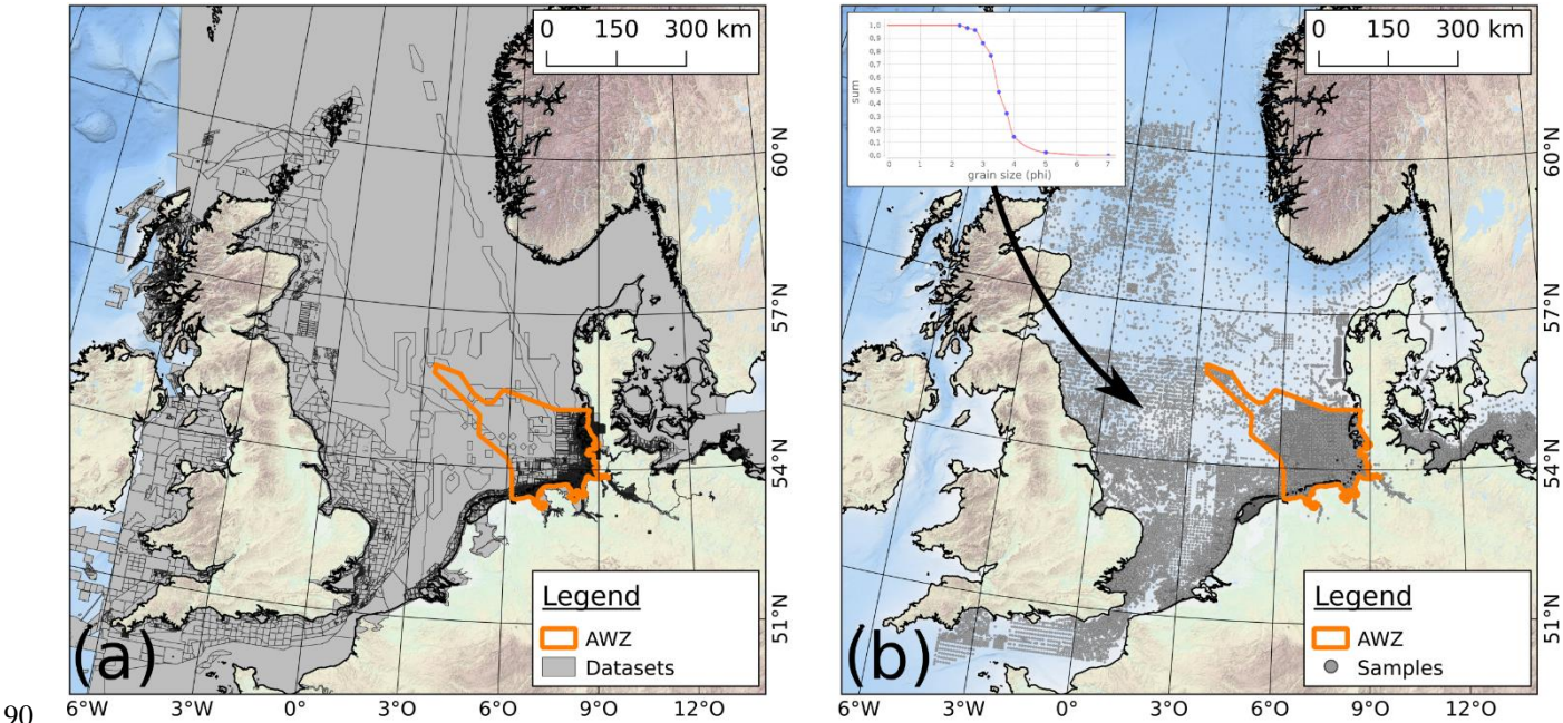
Figure 2: Spatial extent of FSM database, (a) overlapping bathymetric datasets, (b) surface sedimentological datasets represented by continuous GSD functions.
