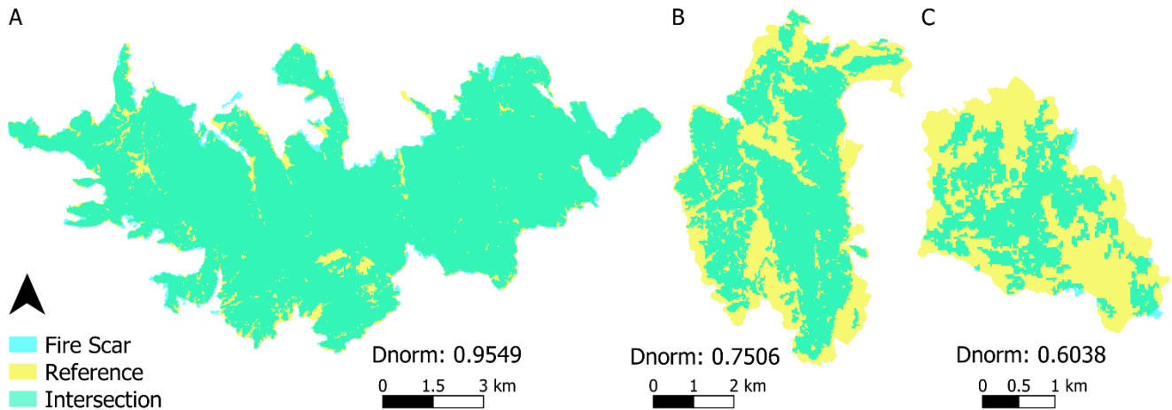
Figure 4: Evaluation of the fire scars. Shown are three examples comparing CONAF's fire scars with the images reconstructed using our Landscape Fire Scars Database methodology. See 2.3 Fire scar evaluation section for detailed description of Dnorm.
