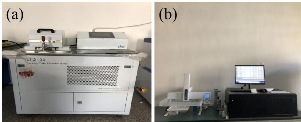
Figure. C3 Analytical instruments. (a) Li-2100 Automatic Vacuum Condensation Extraction instrument, (b) LWIA-24D Liquid water isotope Analyzer.
