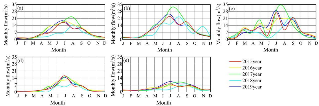
210 Figure 3 Changes in the monthly average flow of five hydrological stations in the Shiyang River Basin, (a) Miscellaneous wood temple, (b) JTL, (c) CQQ, (d) Nanying Reservoir, (e) Huangyang River Reservoir
