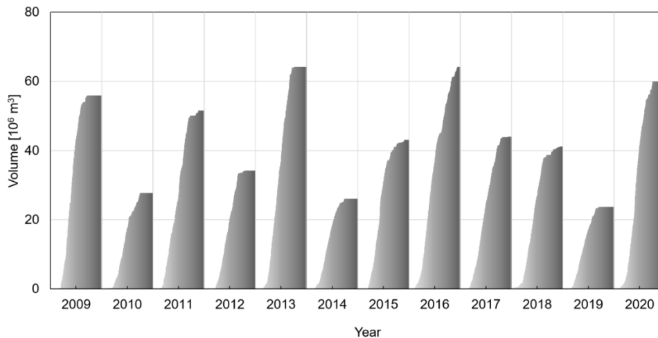
285 Figure 7: Cumulative ablation [ 10^6 \text{ m}^3 ] in May – November (2009 – 2020) for Werenskioldbreen.
