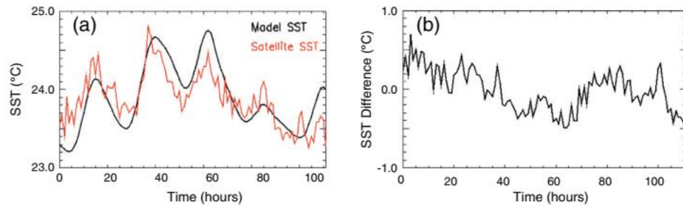
Fig. 2. Example of model first-guess and original SST SEVIRI data over a point in the Mediterranean Sea. (a) Model (black curve) and SEVIRI (red curve) SST time series. (b) Difference between the SEVIRI and model SST.
