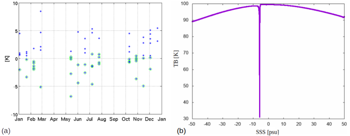
Figure 3. (a) Difference of SMOS and modeled TB (blue stars) for ascending orbits in 2013 for the following acquisition conditions: ( \varphi = 56^\circ , \lambda = 19^\circ , Ascending , x = 0\text{km} , \theta = 42.5^\circ ). Green circles indicate those measurements for which a valid SSS is retrieved. (b) Half first Stokes modeled TB (MW model) versus raw SSS for \theta = 40^\circ and T_s = 0^\circ\text{C} . Note that negative SSS values do not have any physical meaning. They only reflect the presence of instrumental biases that need to be corrected.
