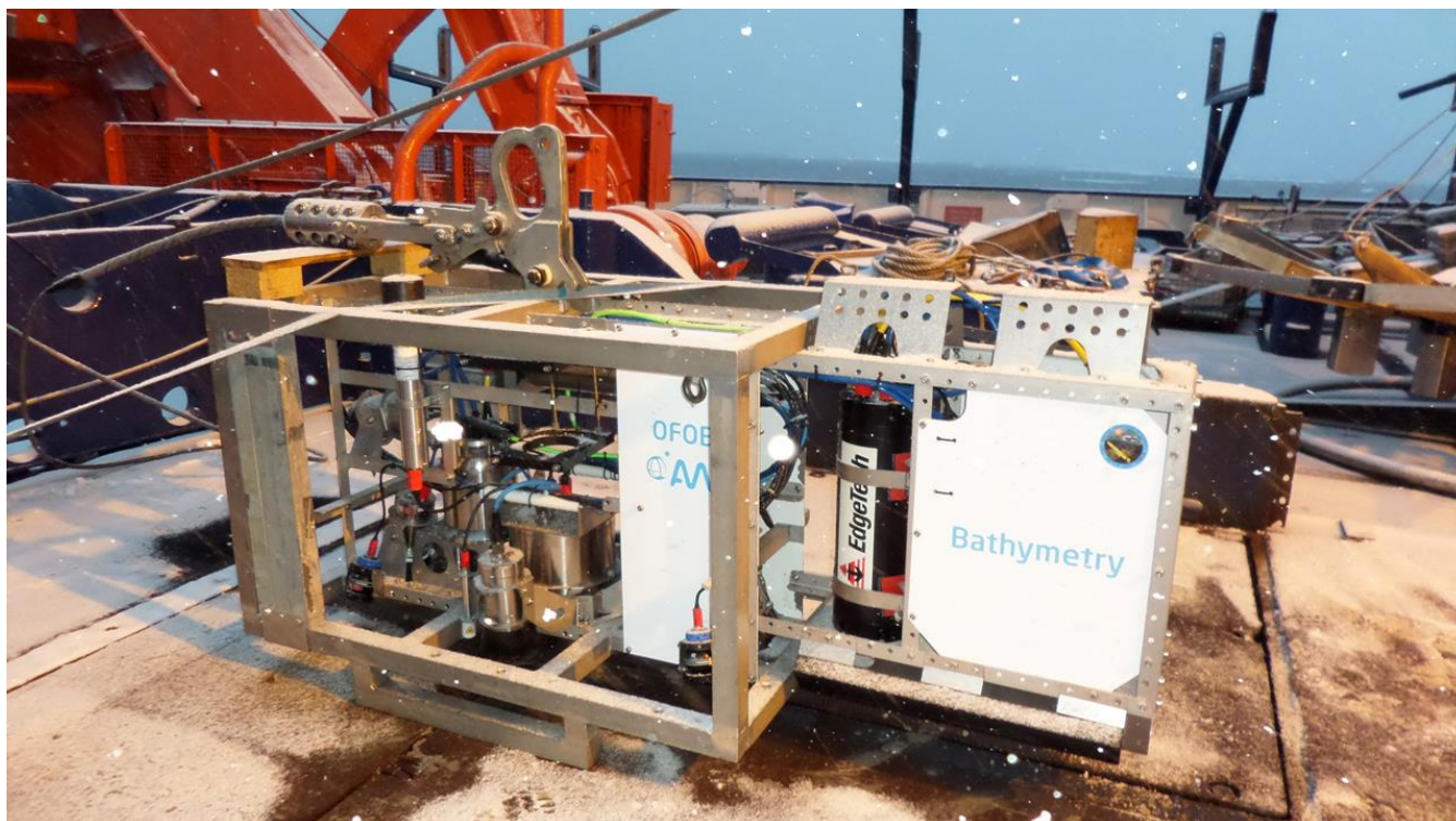
350 Figure 1: The Ocean Floor Observation and Bathymetry System (OFOBS) of the Alfred Wegener Institute (AWI), Helmholtz Centre for Polar and Marine Research, on deck awaiting deployment during the PS124 expedition to the southern Weddell Sea (February-March 2021).
