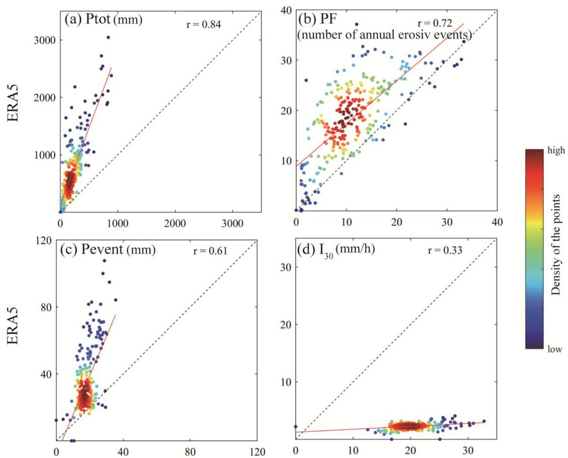
Figure 4. Scatterplots of the station-based multi-year average (a) annual erosive precipitation amount (Ptot), (b) annual erosive precipitation frequency (PF), (c) mean erosive event precipitation amount (Pevent), (d) mean I_{30} for erosive events ( I_{30} ) vs those derived from ERA5 data at the corresponding grid cells in 2013–2020.
