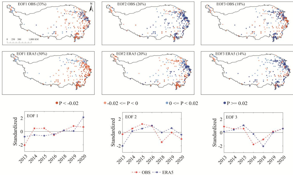
Figure 7. First three EOF modes of observed and ERA5-based mean annual rainfall erosivity on the TP in 2013–2020 (excluding 2017).
