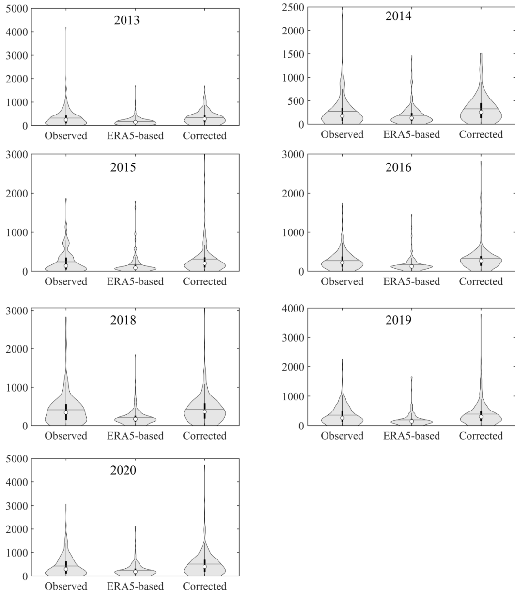
355 Figure 10. Violin plots of observed, ERA5-based, and corrected annual rainfall erosivity in validation grids for 2013–2020 (excluding 2017). Y axis shows annual rainfall erosivity in MJ·mm·ha -1 ·h -1 . The boxplot diagram of the median of the violin plots shows the maximum value, 75% quantile value, 50% quantile value, 25% quantile value, and minimum value. The horizontal lines represent average values.
