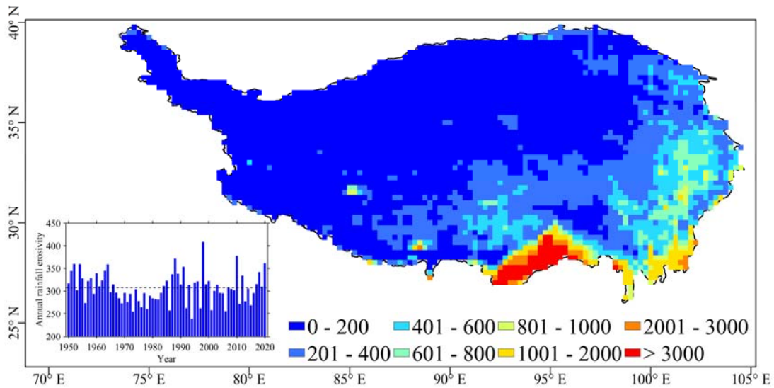
Figure 11. R factor map of TP with the 0.25^\circ spatial resolution for 1950–2020. Inset represents the yearly change in annual rainfall erosivity.
