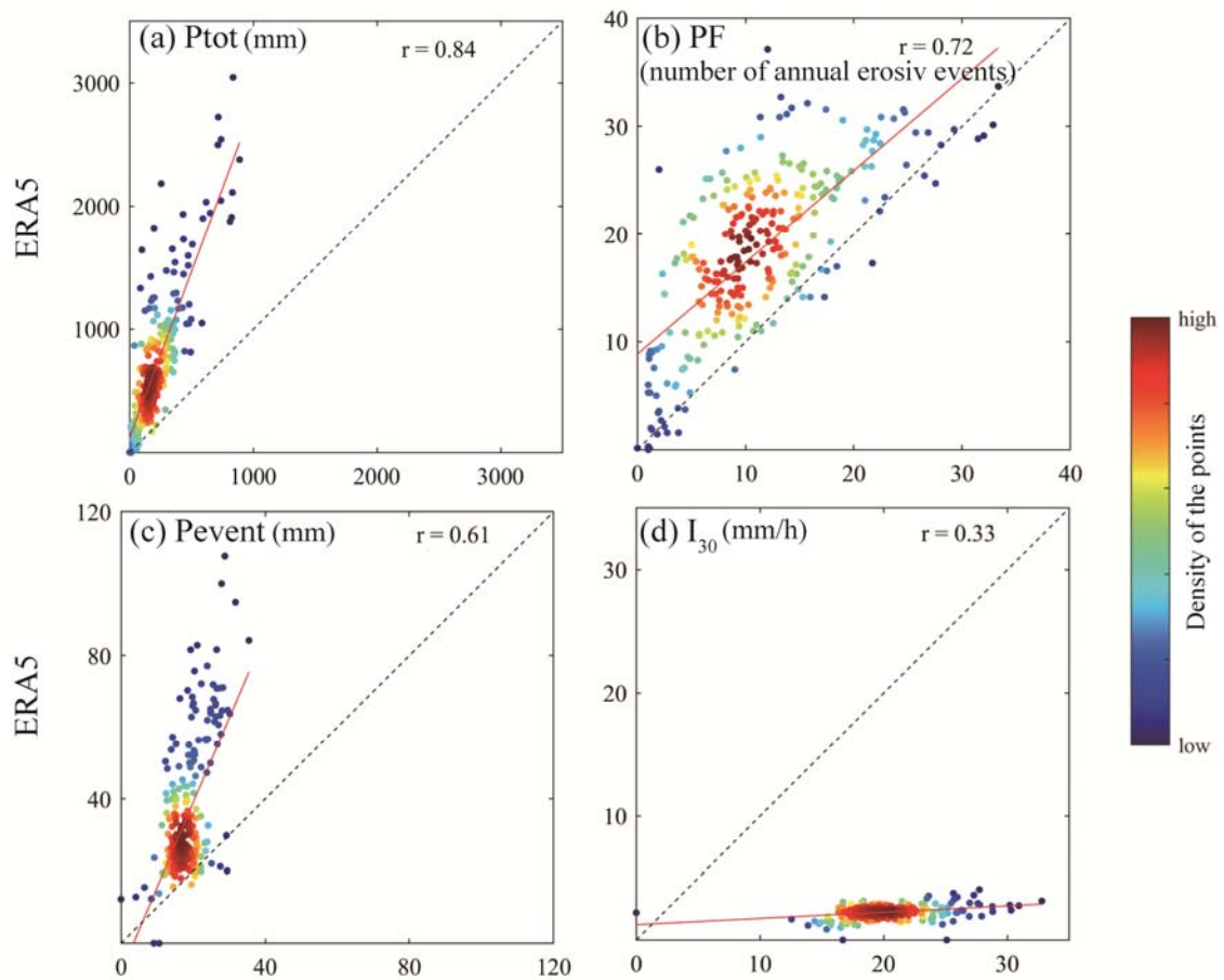
270 Figure 4. Scatterplots of the station-based multi-year averaged (a) annual erosive precipitation amount (Ptot), (b) annual erosive precipitation frequency (PF), (c) mean erosive event precipitation amount (Pevent), (d) mean I_{30} for erosive events ( I_{30} ) vs those derived from ERA5 data at the corresponding grid cells in 2013–2020.
