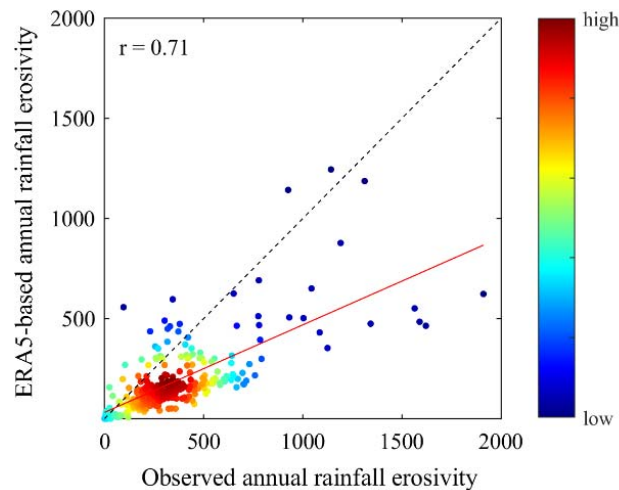
280 Figure 5. Comparison of mean annual rainfall erosivity based on observed and ERA5-based results for seven years (2013–2020, excluding 2017). The dotted line is the result of an optimal model (with an intercept of 0 and regression coefficient of 1). The red line is the regression result. Colors of dots represent the grid density. Unit: \text{MJ}\cdot\text{mm}\cdot\text{ha}^{-1}\cdot\text{h}^{-1}\cdot\text{yr}^{-1} .
